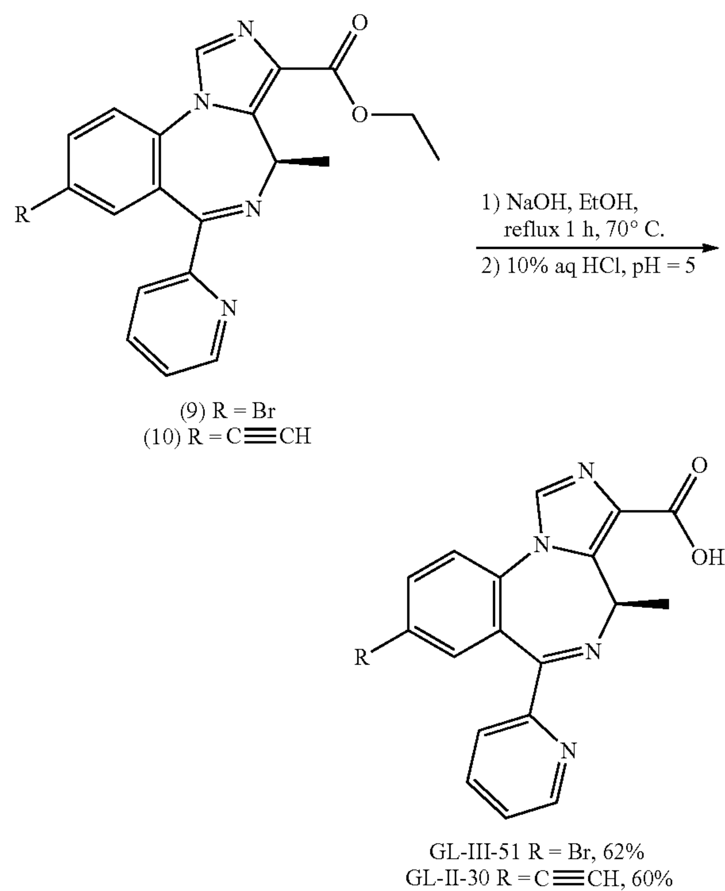
Scheme 3. Synthesis of compounds with formulae (I) part III.
