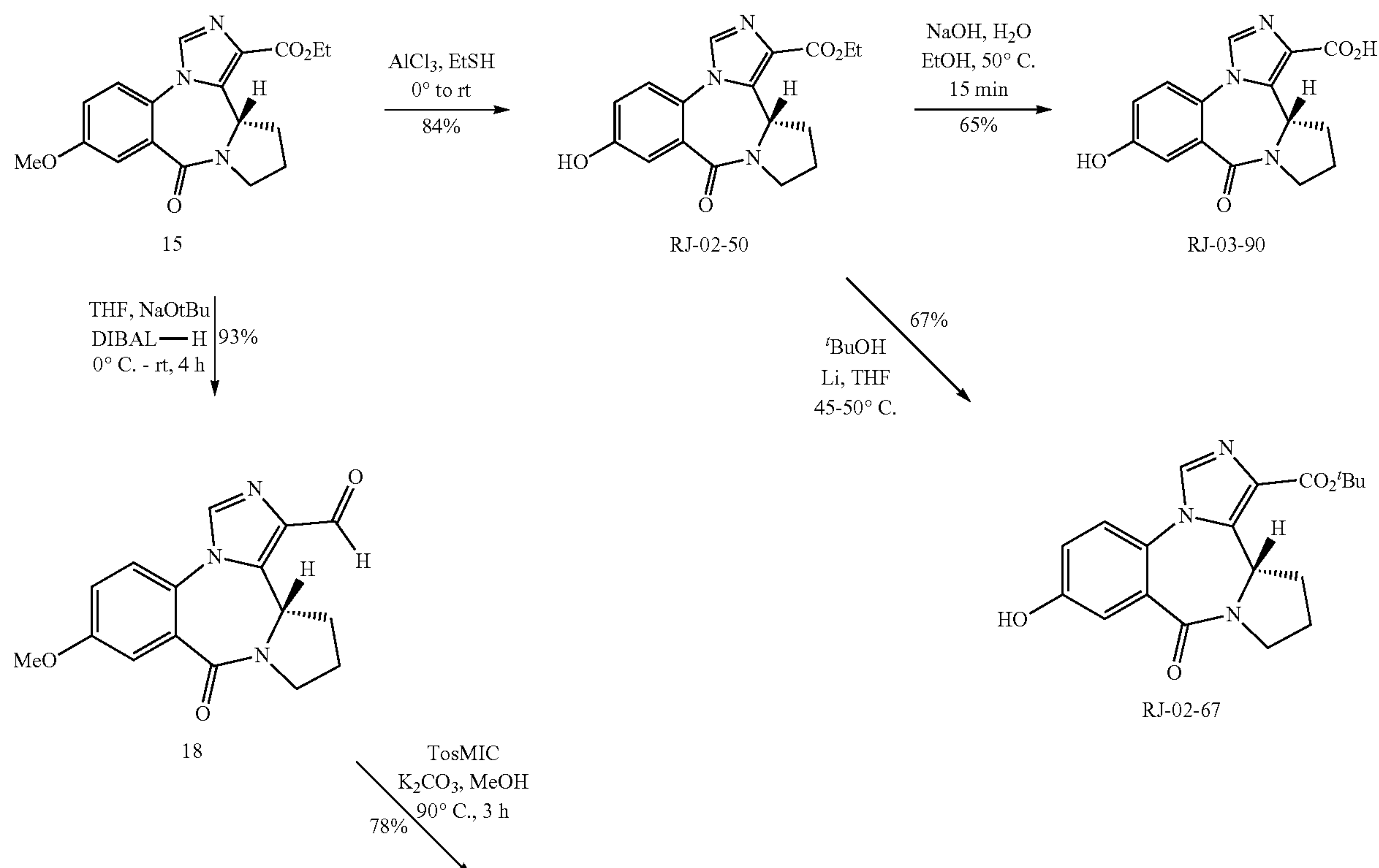
Scheme 5. Synthesis of compounds with formulae (II).
