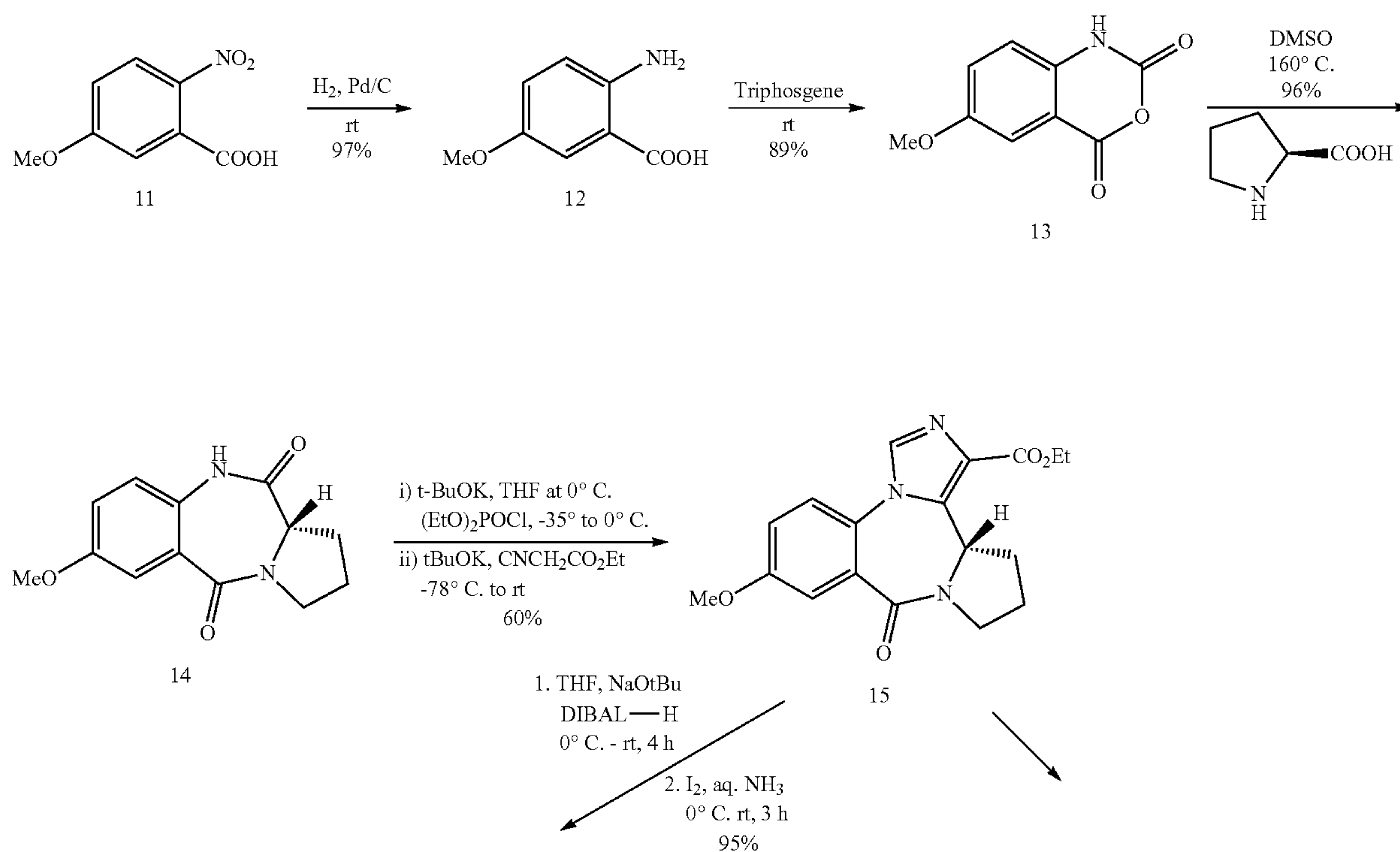
Scheme 4. Synthesis of compounds with formulae (II).
