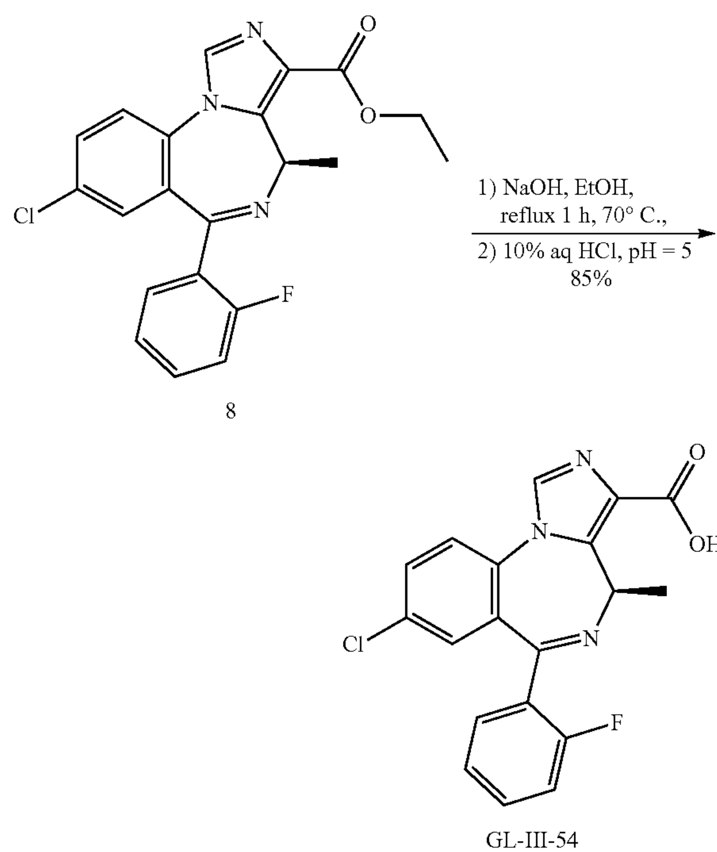
Scheme 2. Synthesis of compounds with formulae (I) part II.
