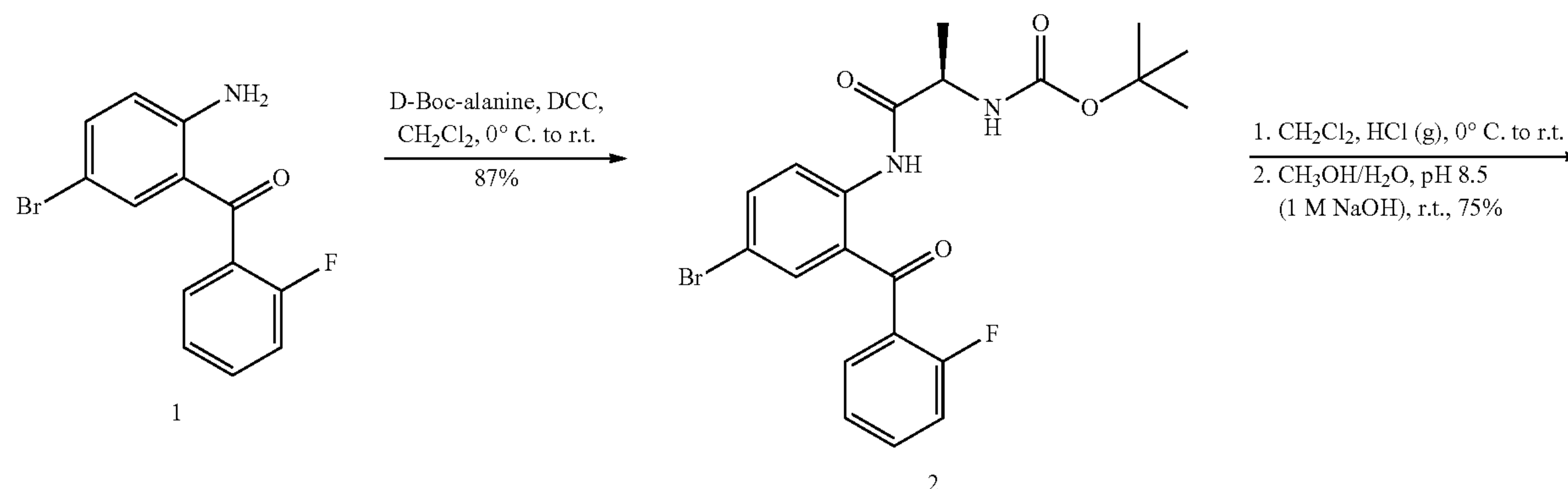
Scheme 1. Synthesis of compounds with formulae (I) part I.
