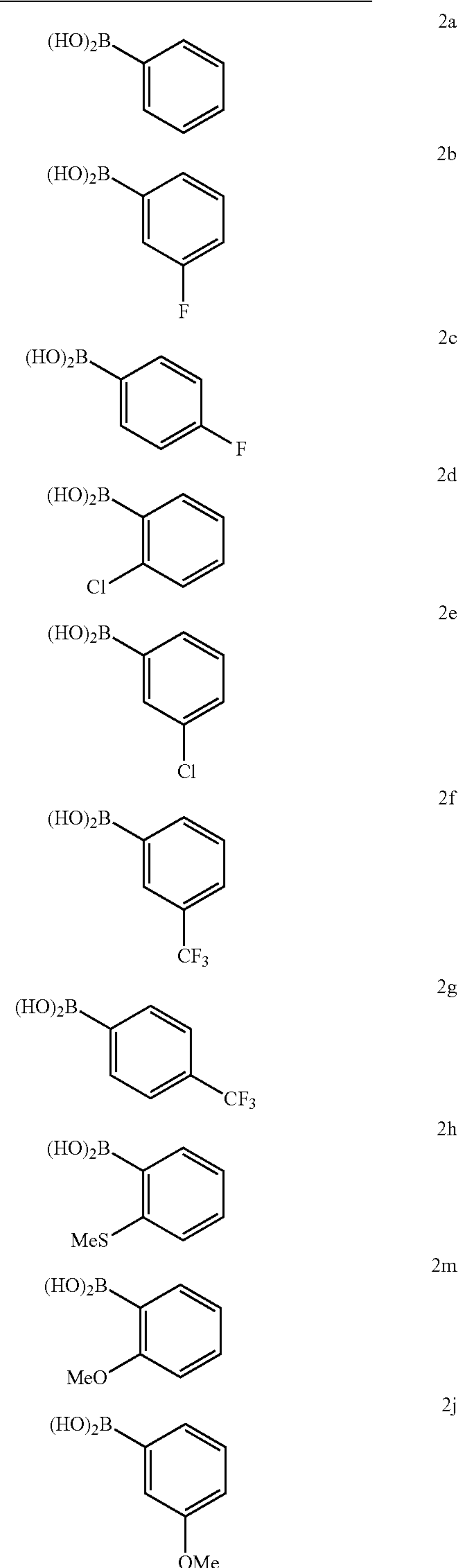
Scheme 2. Boronic acids selected for incorporation into novologue X scaffold.
