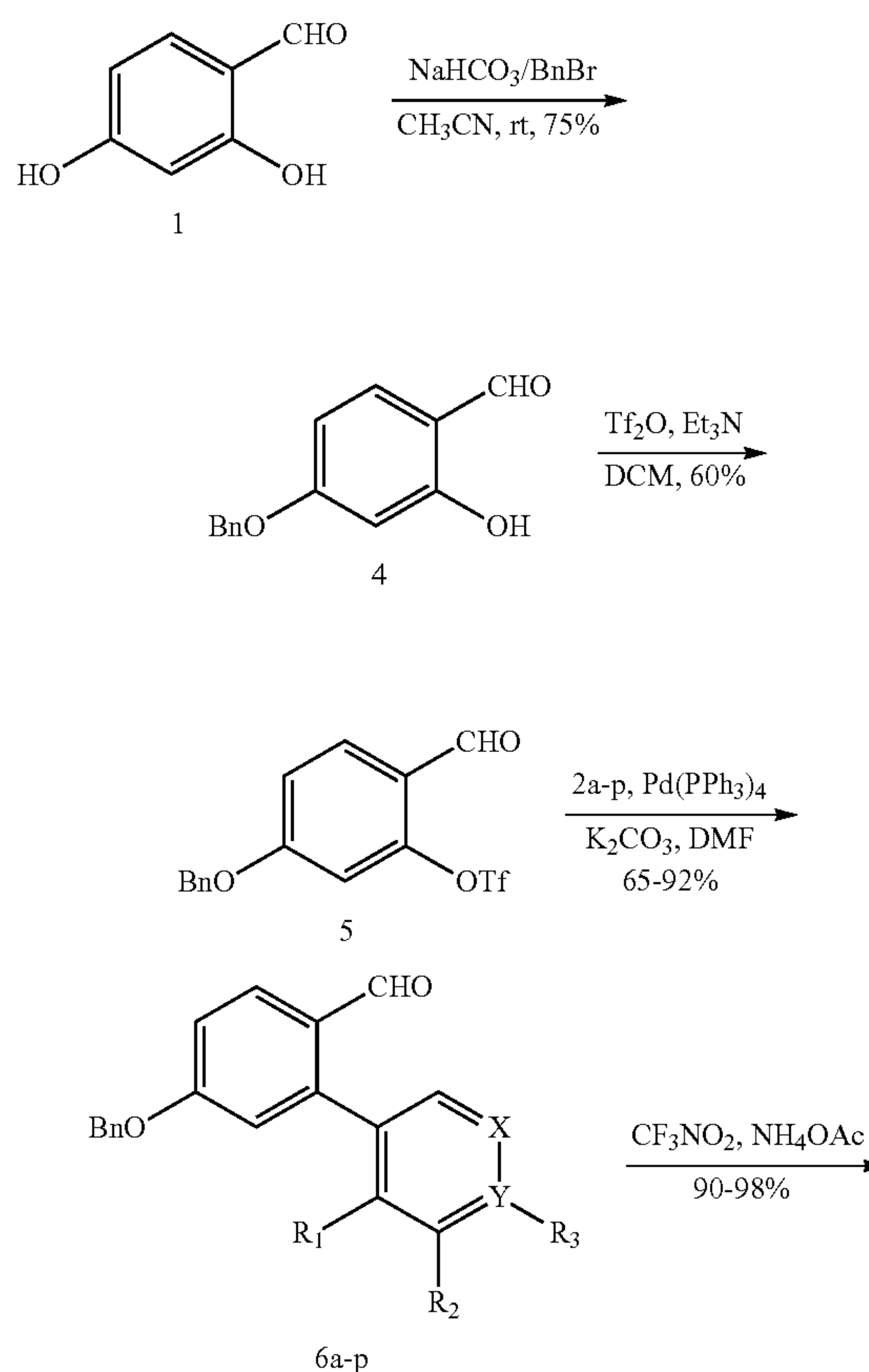
Scheme 3. Synthesis of ethyl acetamide side chain containing novologues.
