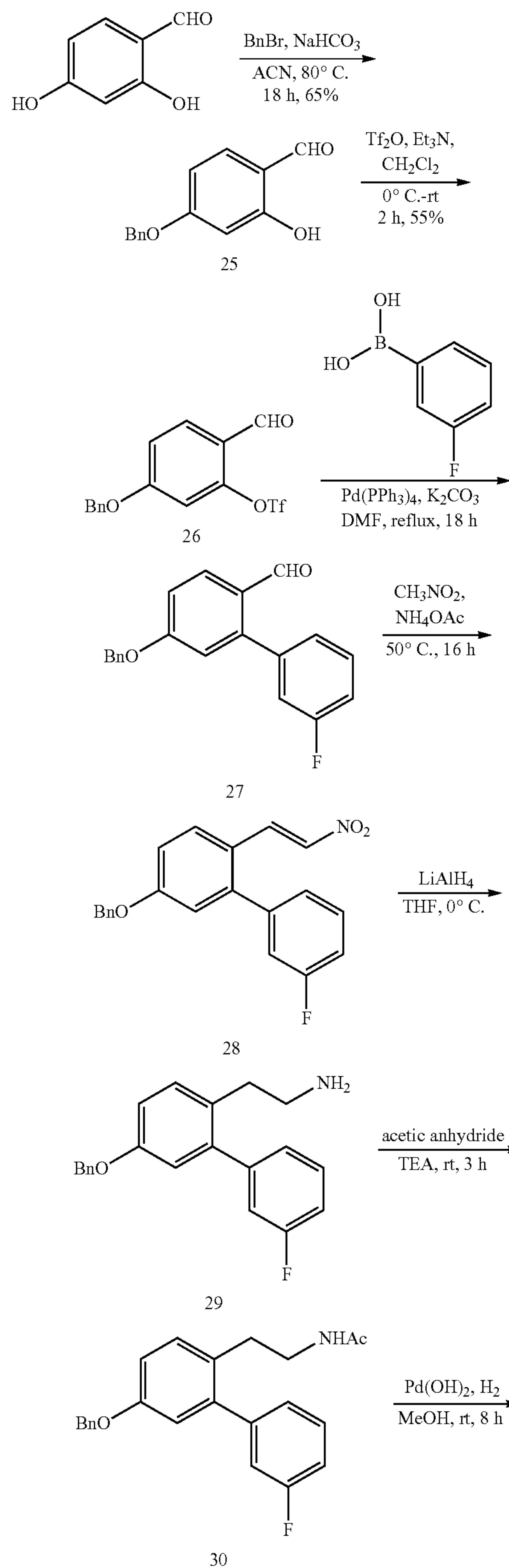
Scheme 6. Synthesis of phenol core intermediate 23.
