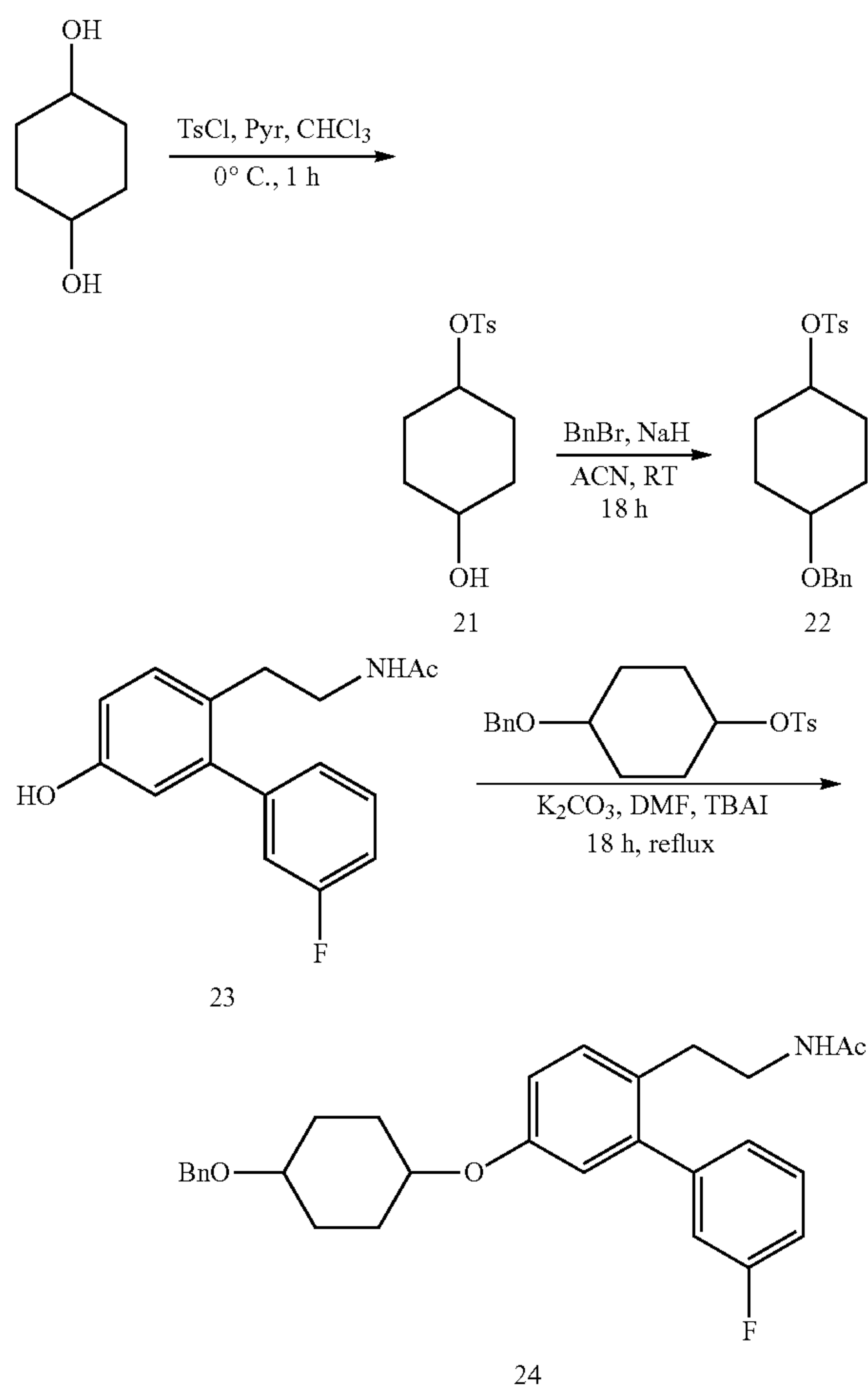
Scheme 5. Synthesis of carbocyclic sugar analogue compound 24.
