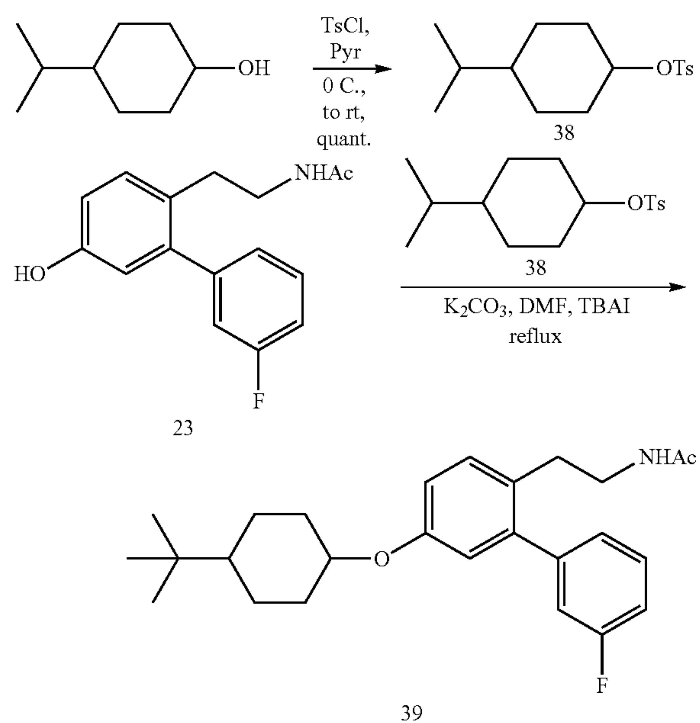
Scheme 8 Synthesis of carbocyclic compound 39.
