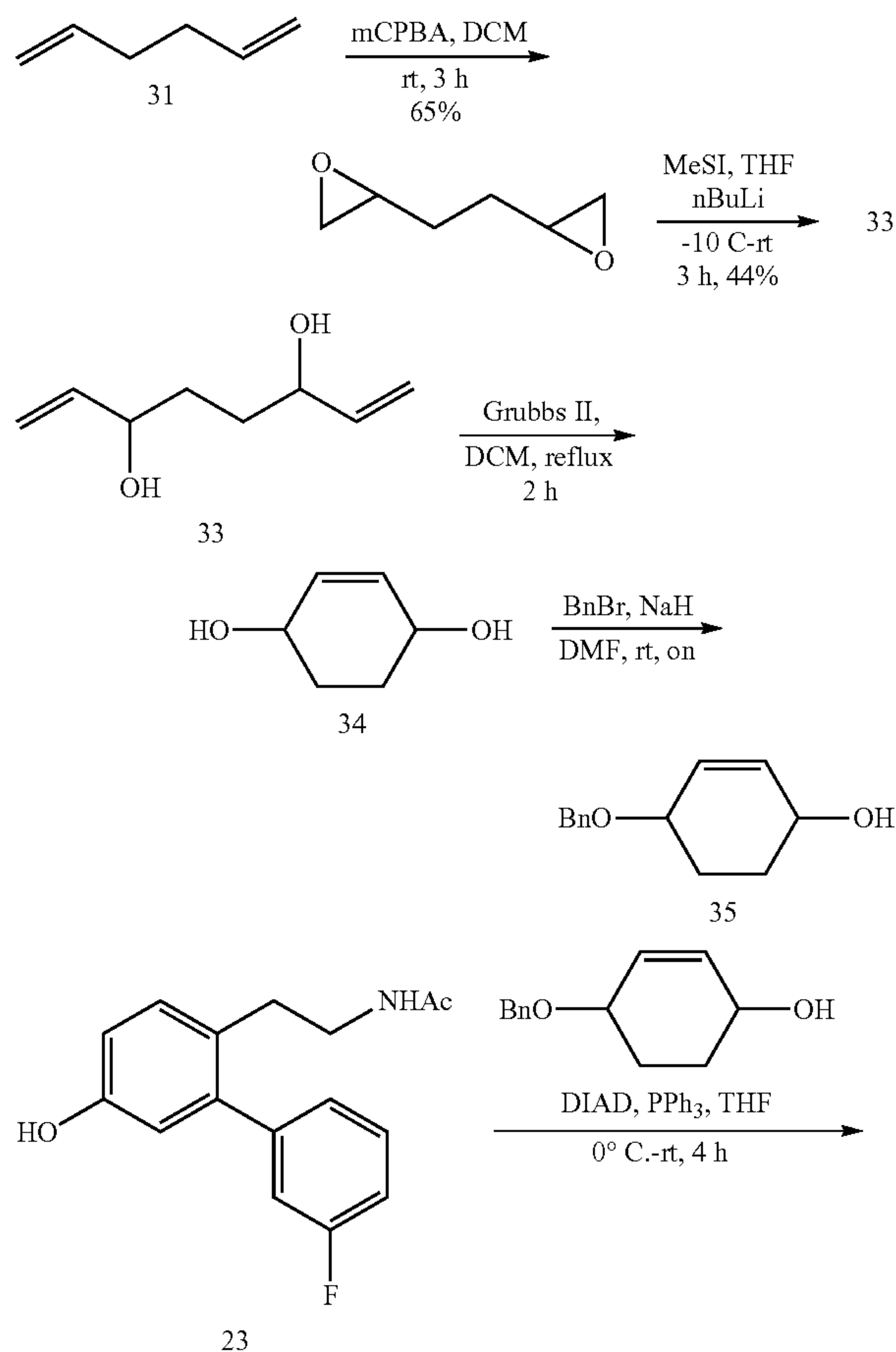
Scheme 7. Synthesis of carbocyclic sugar analogues 36 and 37.
