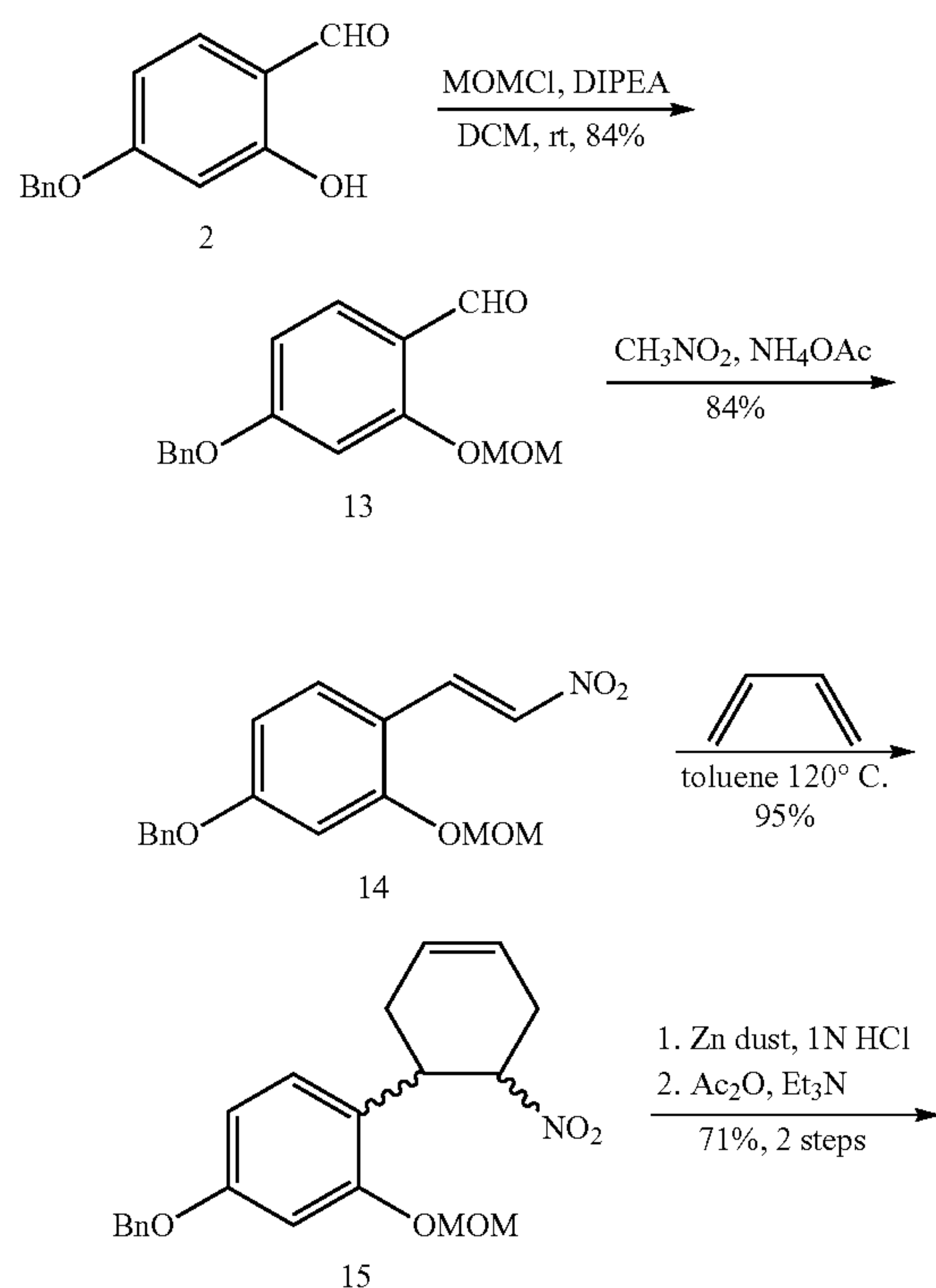
Scheme 4. Synthesis of cyclohexene containing novologues.
