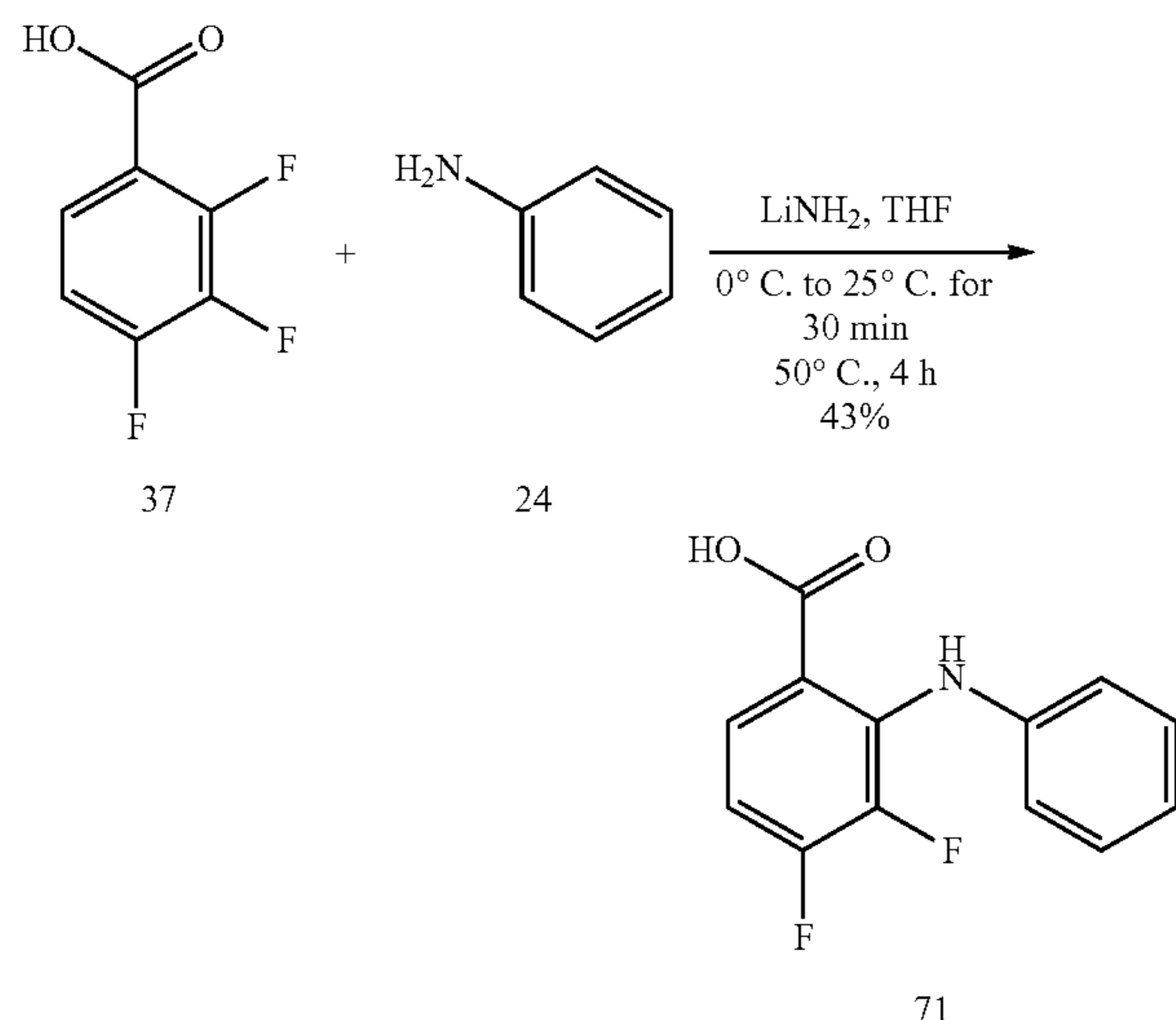
Scheme 6: Synthesis of 71 using lithium amide displacement method.
