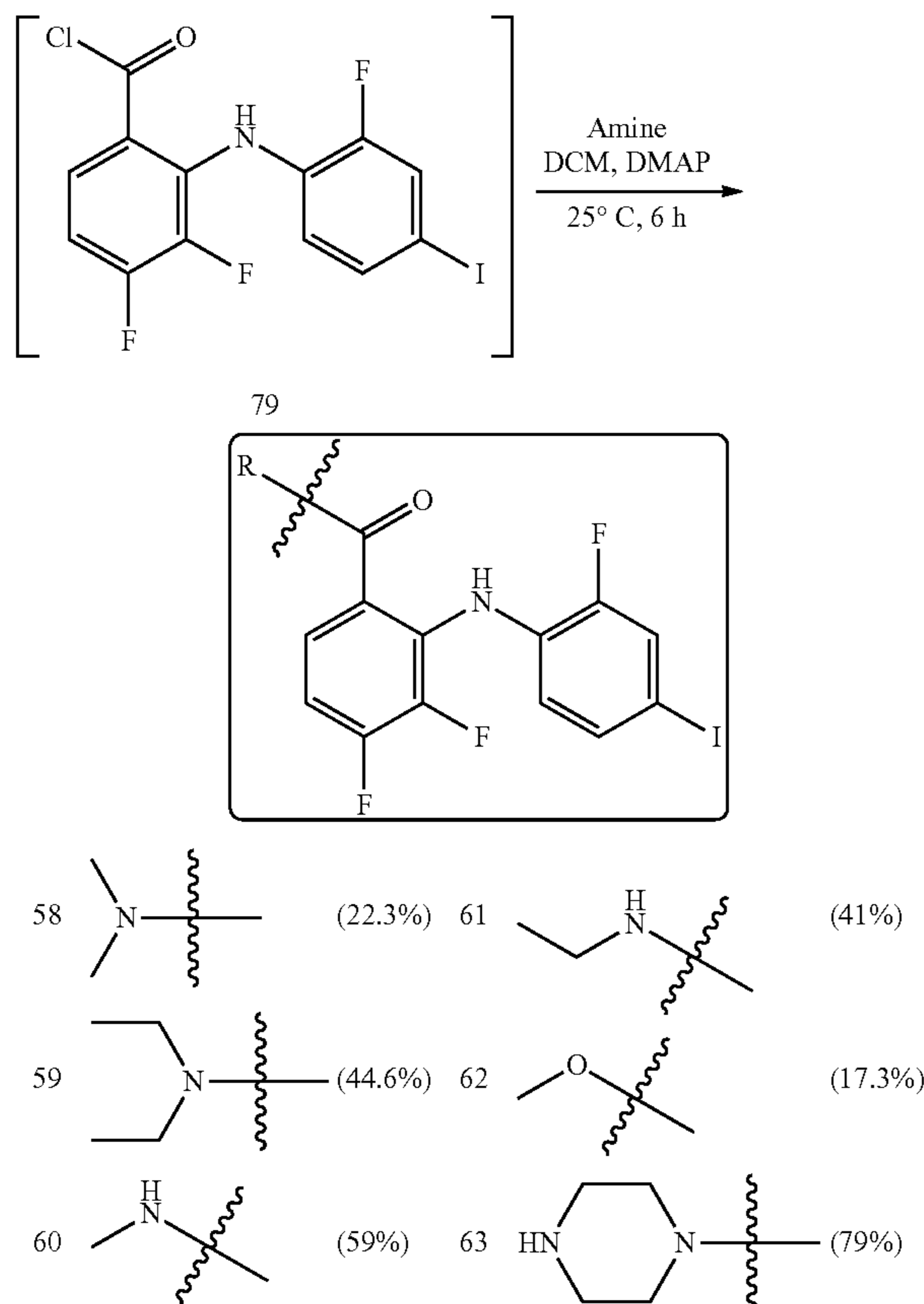
Scheme 3: Synthesis of simple amides using the acid chloride method.
