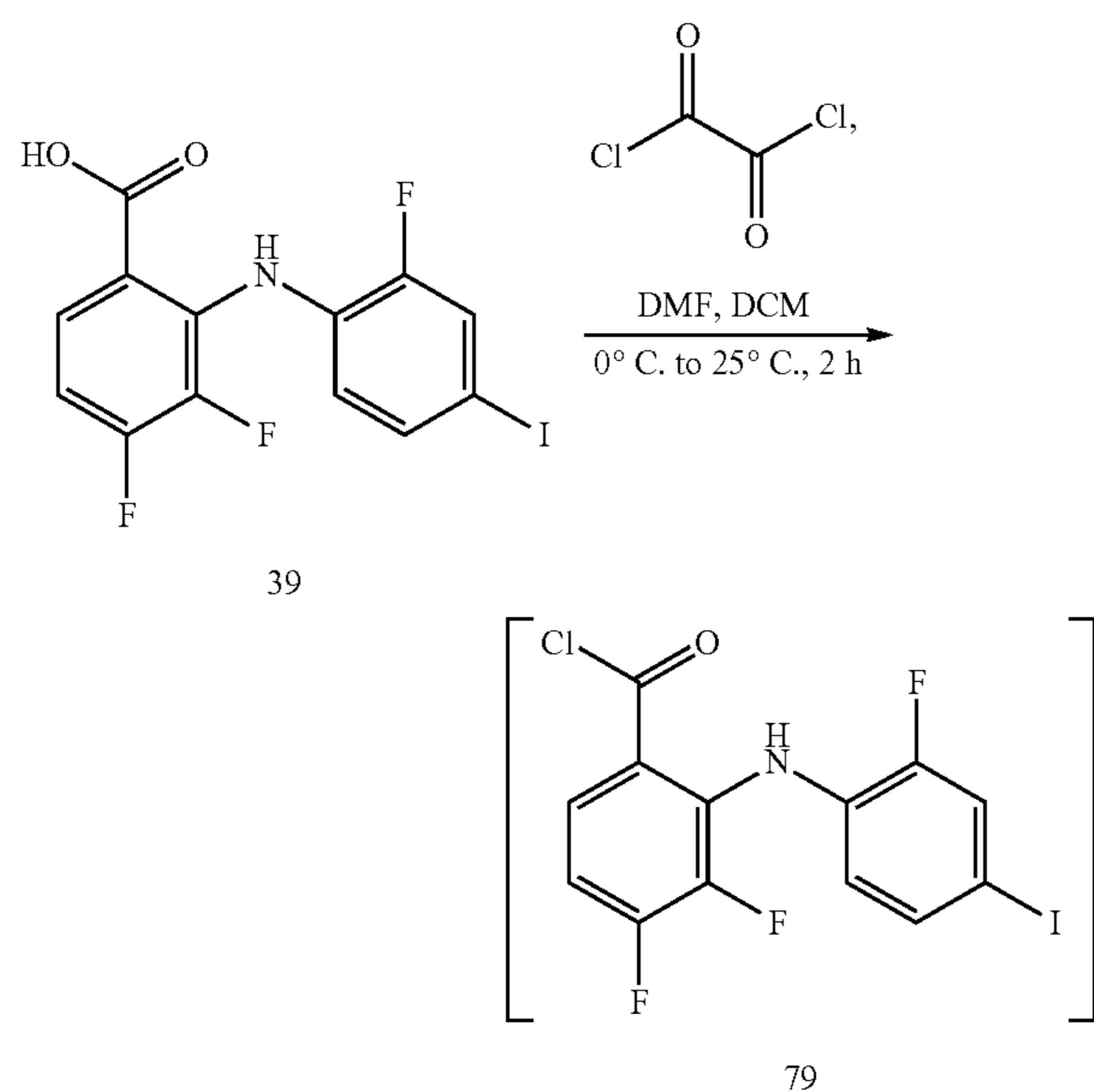
Scheme 2: Acid chloride formation.
