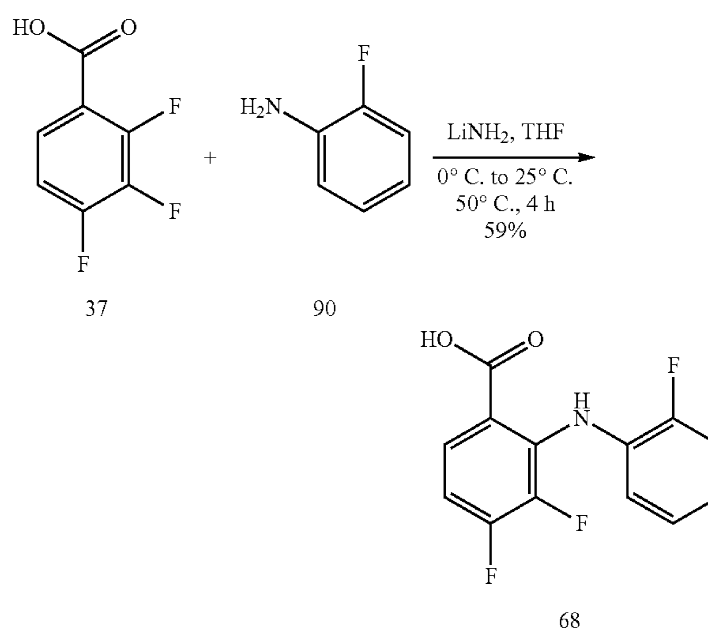
Scheme 4: Lithium amide displacement method (see Davis, et al. Org. Process Res. Dev. 2005, 9, 843-846).
