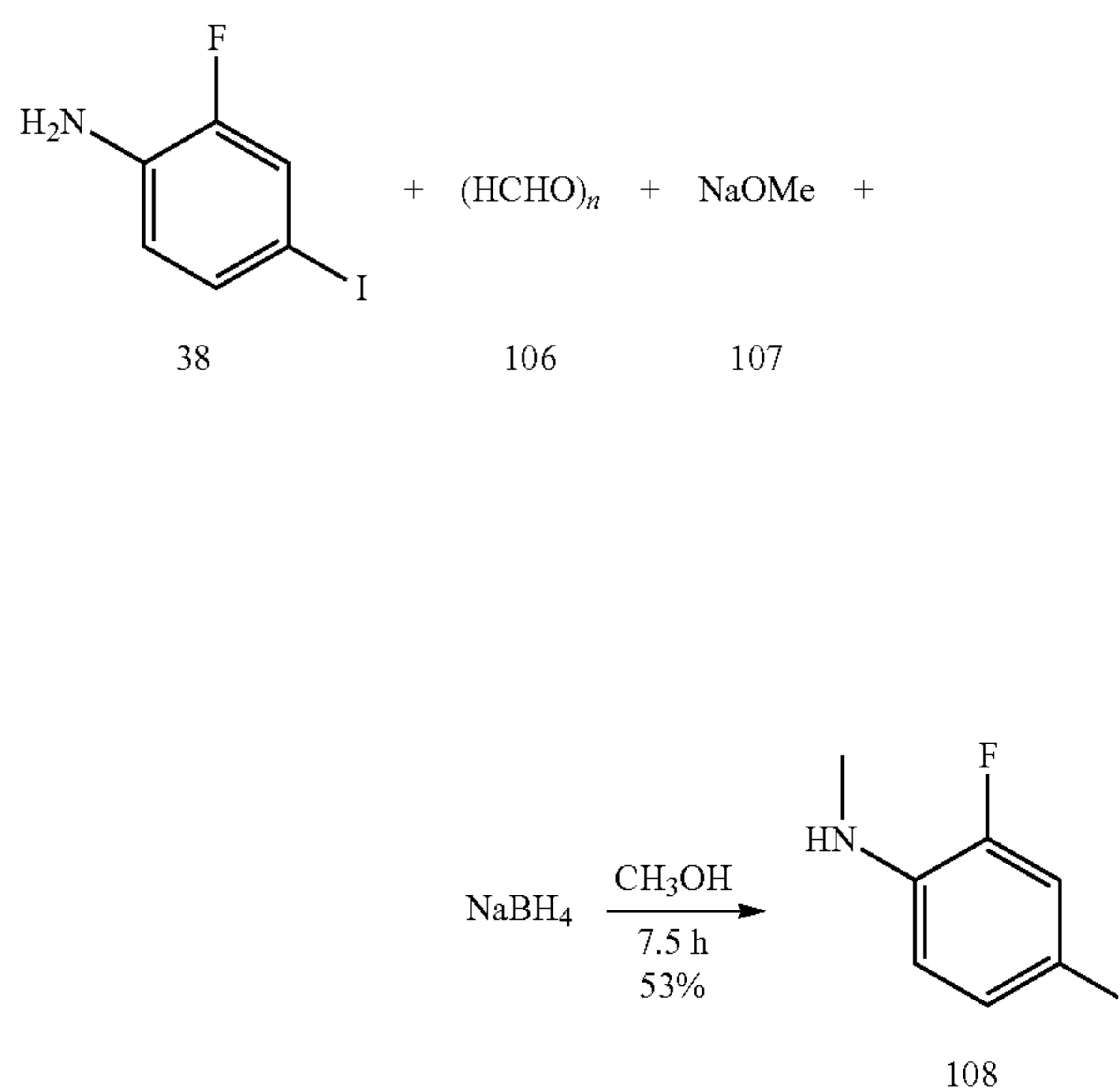
Scheme 13: Monomethylation reaction of 38.
