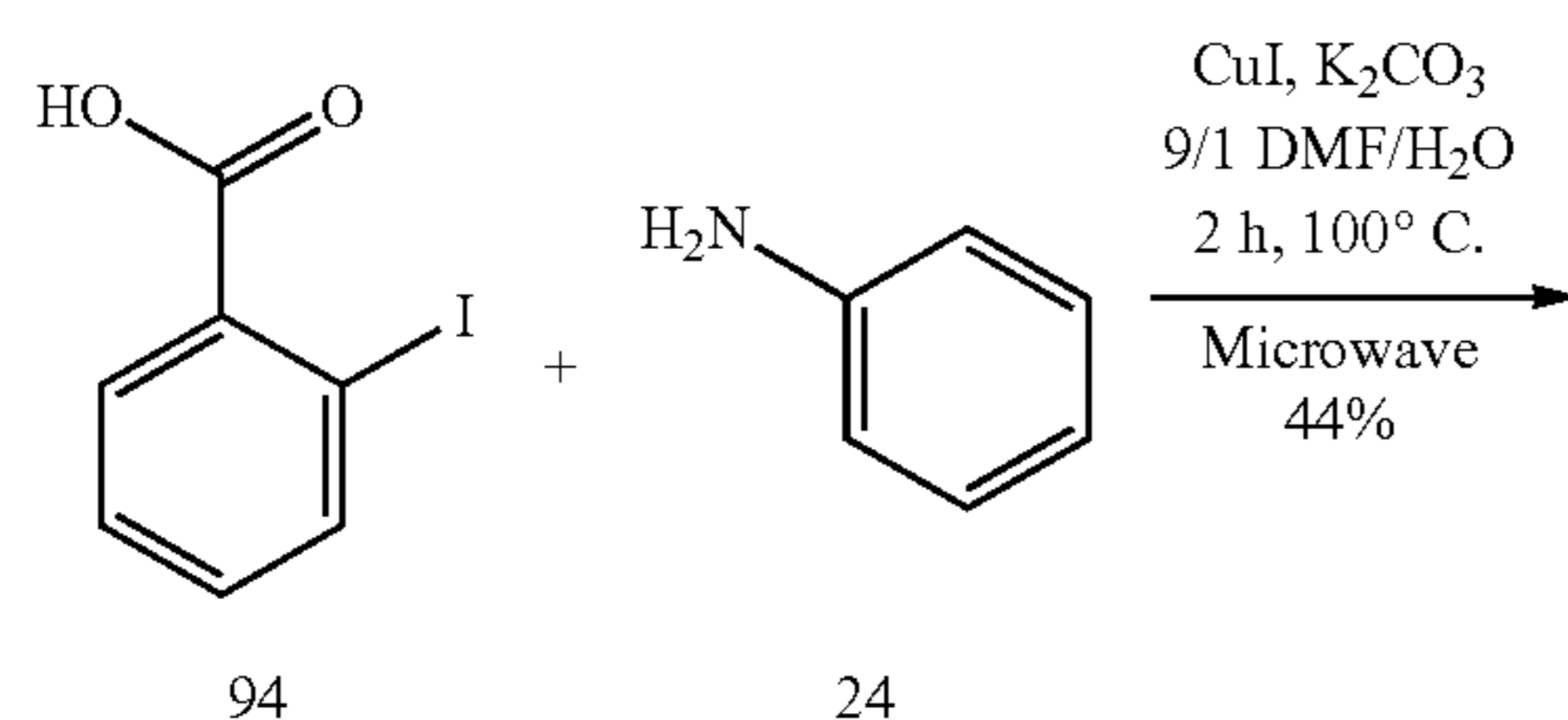
Scheme 9: Ullmann coupling strategy to synthesize 25.
