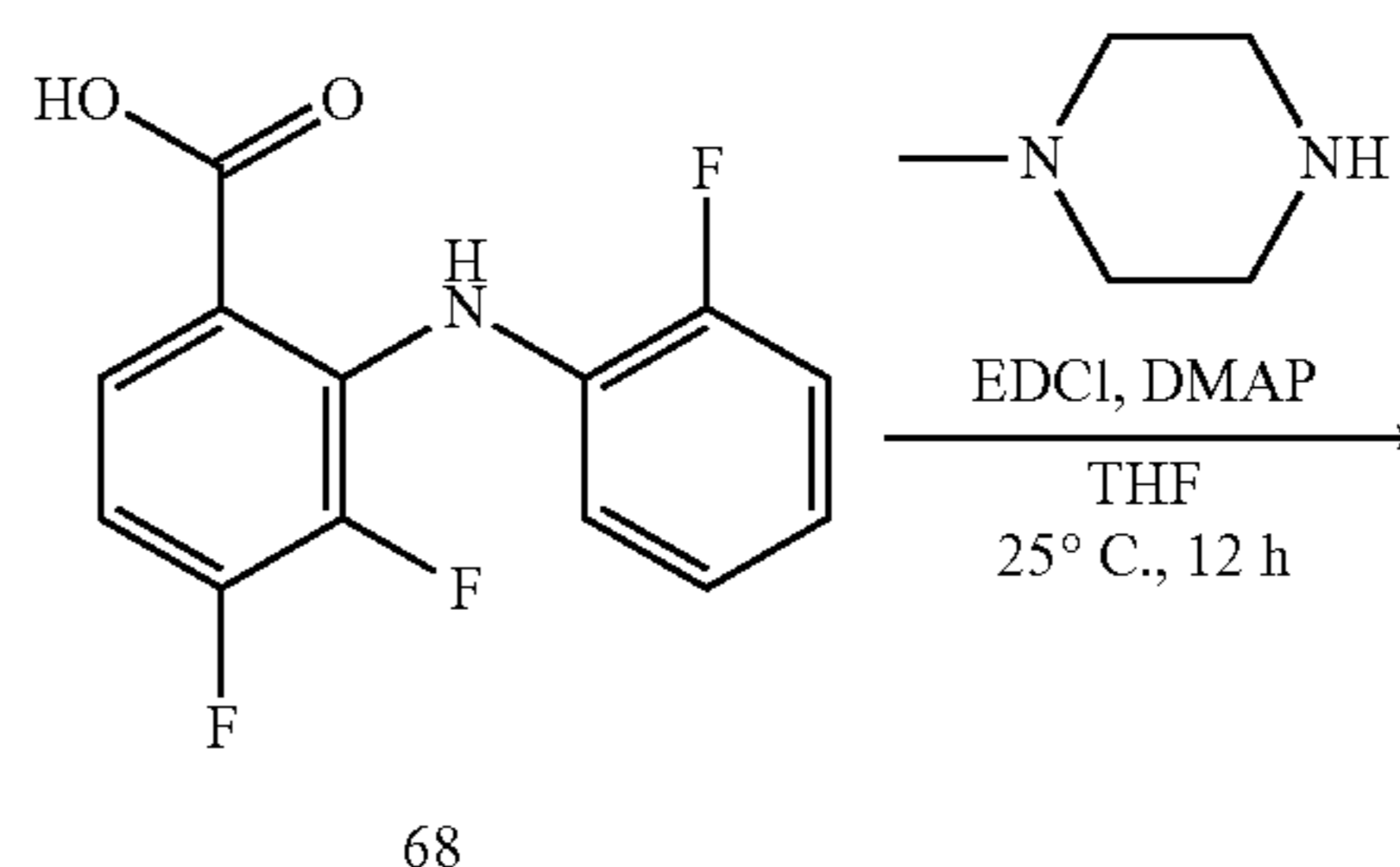
Scheme 5: Synthesis of 69 Fumarate by EDCI coupling.
