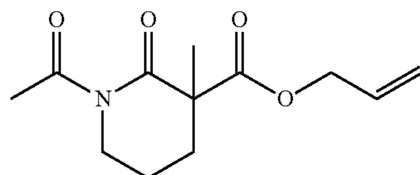
R is acetyl
