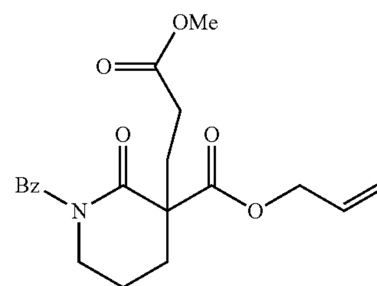
Benzoyl Lactam SI10
