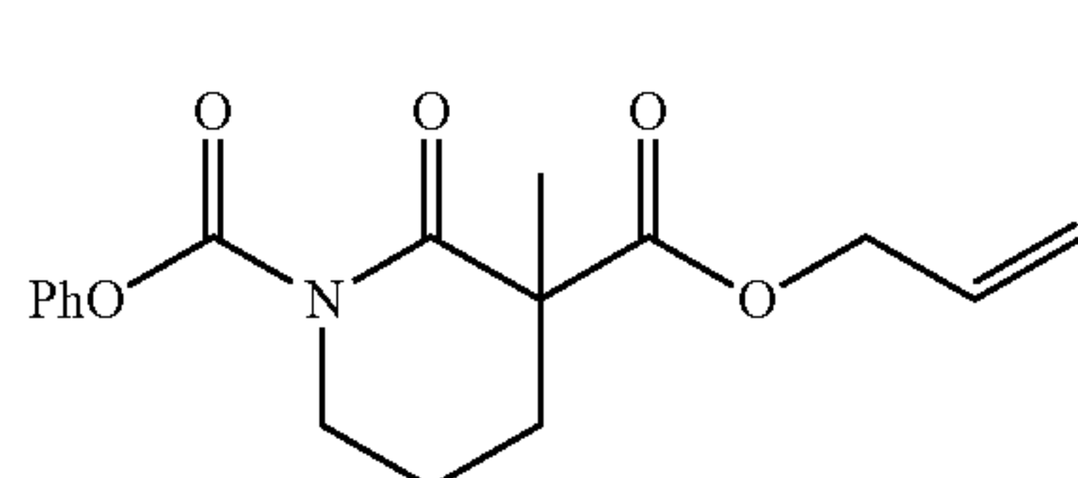
Phenyl Carbamate Lactam SI23
