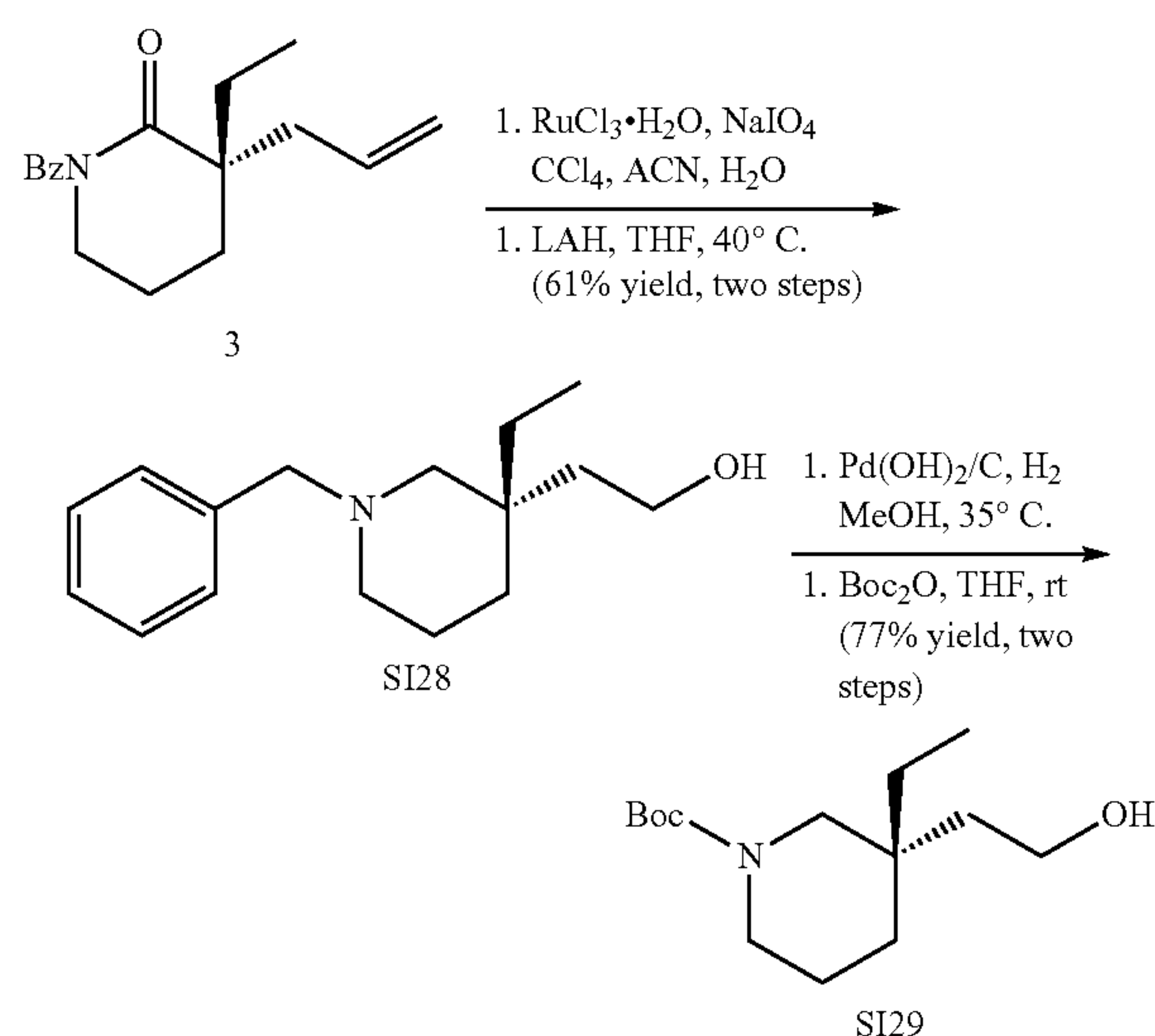
Benzoyl Lactam 3 Reaction Scheme 2
