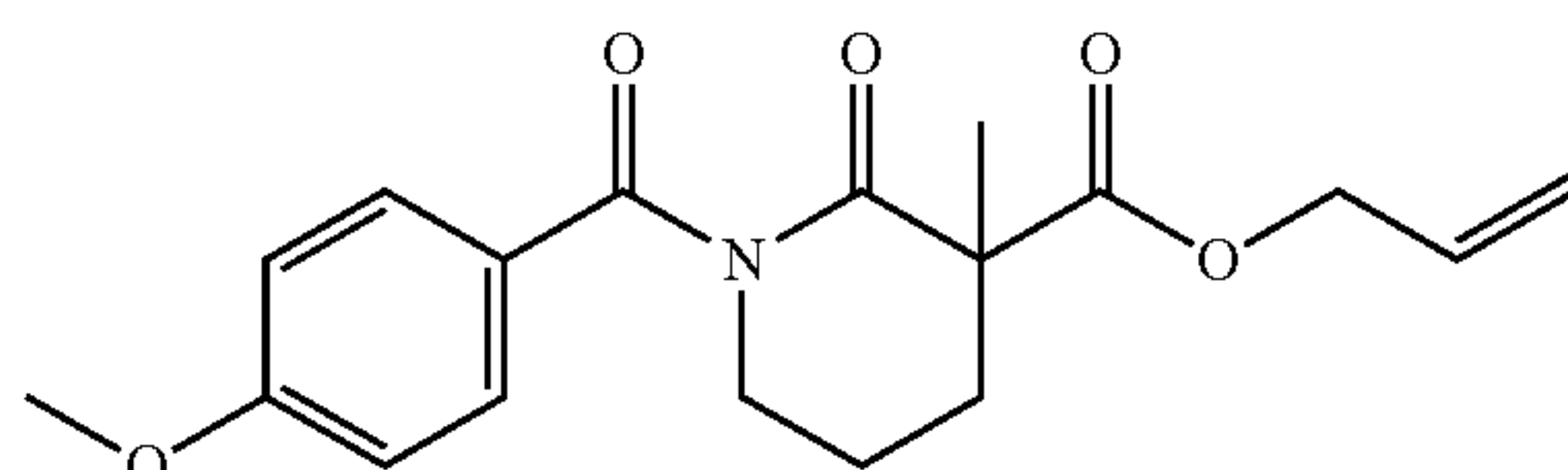
R is 4-OMe-Bz (i.e., 4-methoxybenzoyl)
