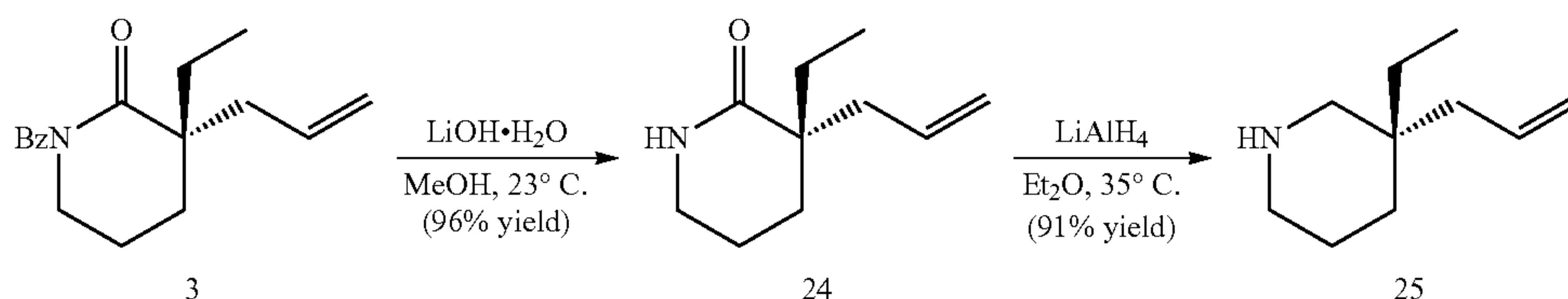
Synthesis Reaction Scheme
