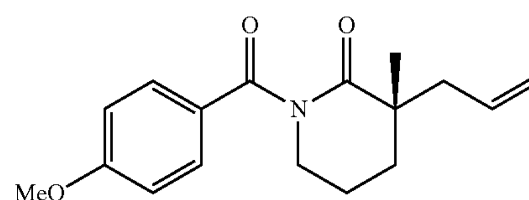
4-Methoxybenzoyl Lactam 2f
