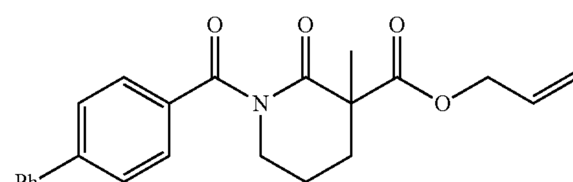
4-Phenylbenzoyl Lactam SI25
