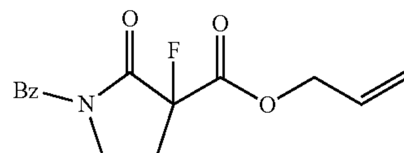
Benzoyl Lactam SI16
