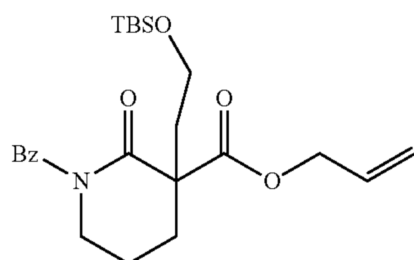
Benzoyl Lactam SI11
