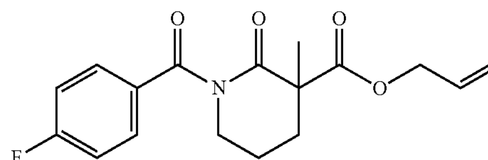
R is 4-F-Bz (i.e., 4-fluorobenzoyl)
