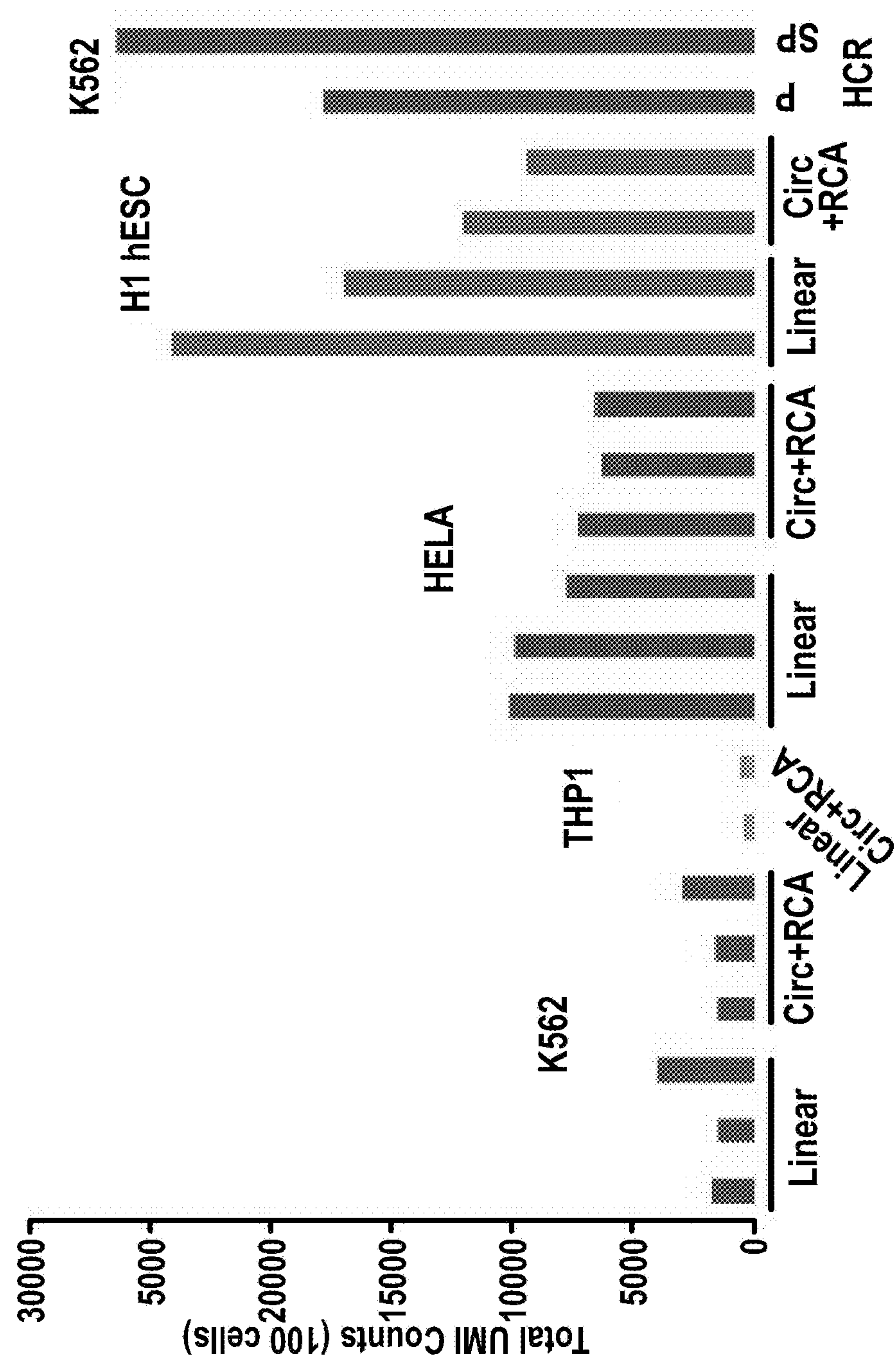
GAPDH UMIs increased in K562s with the Adapted HCR System
