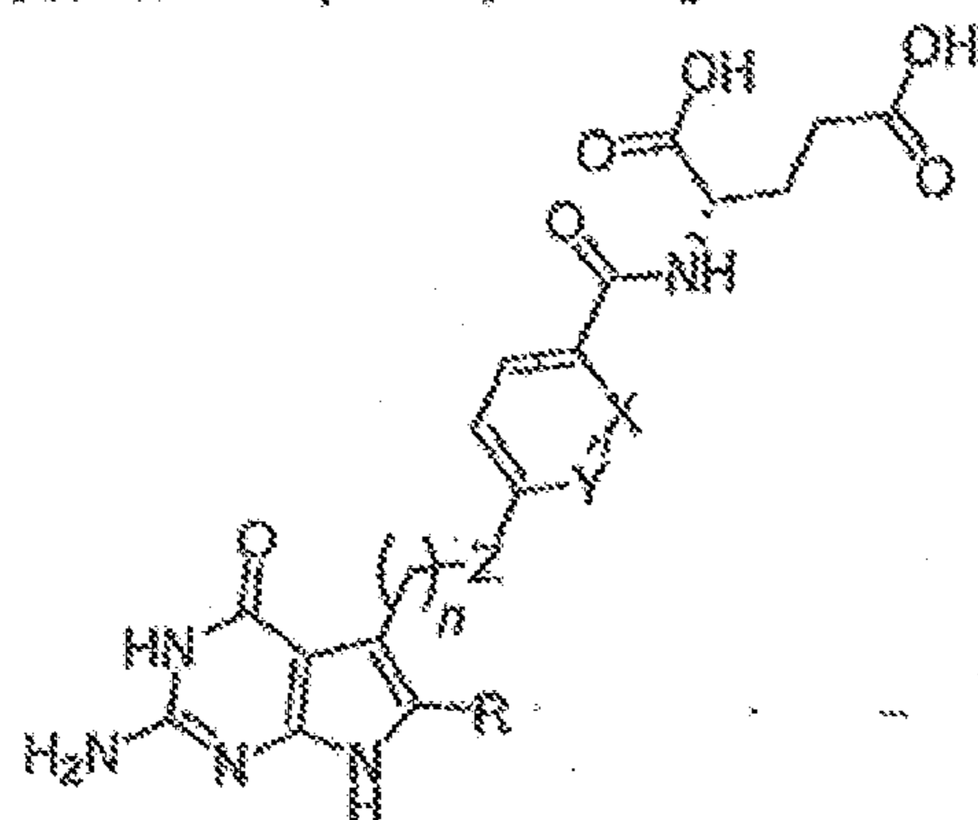
FORMULA III
