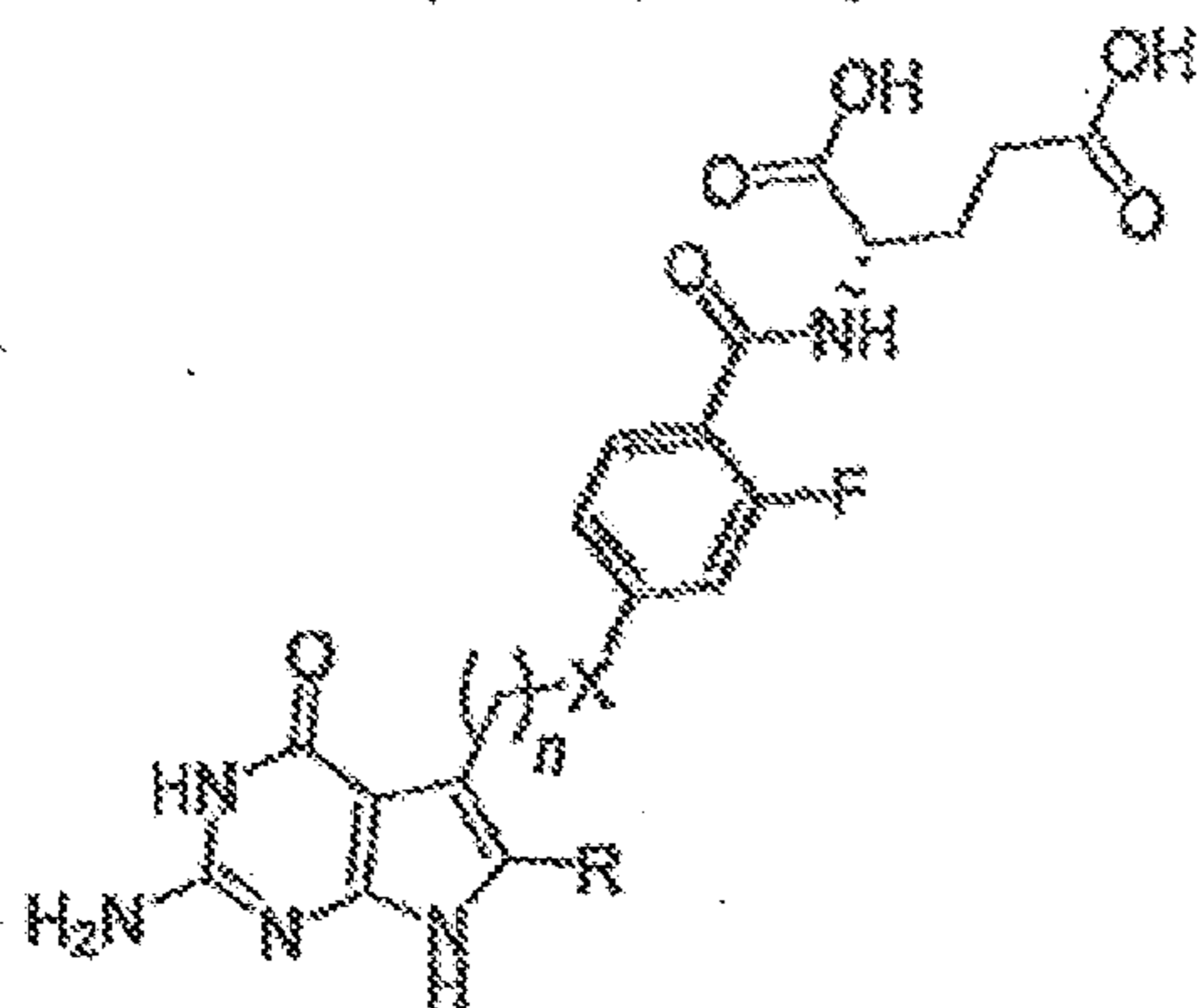
FORMULA II
