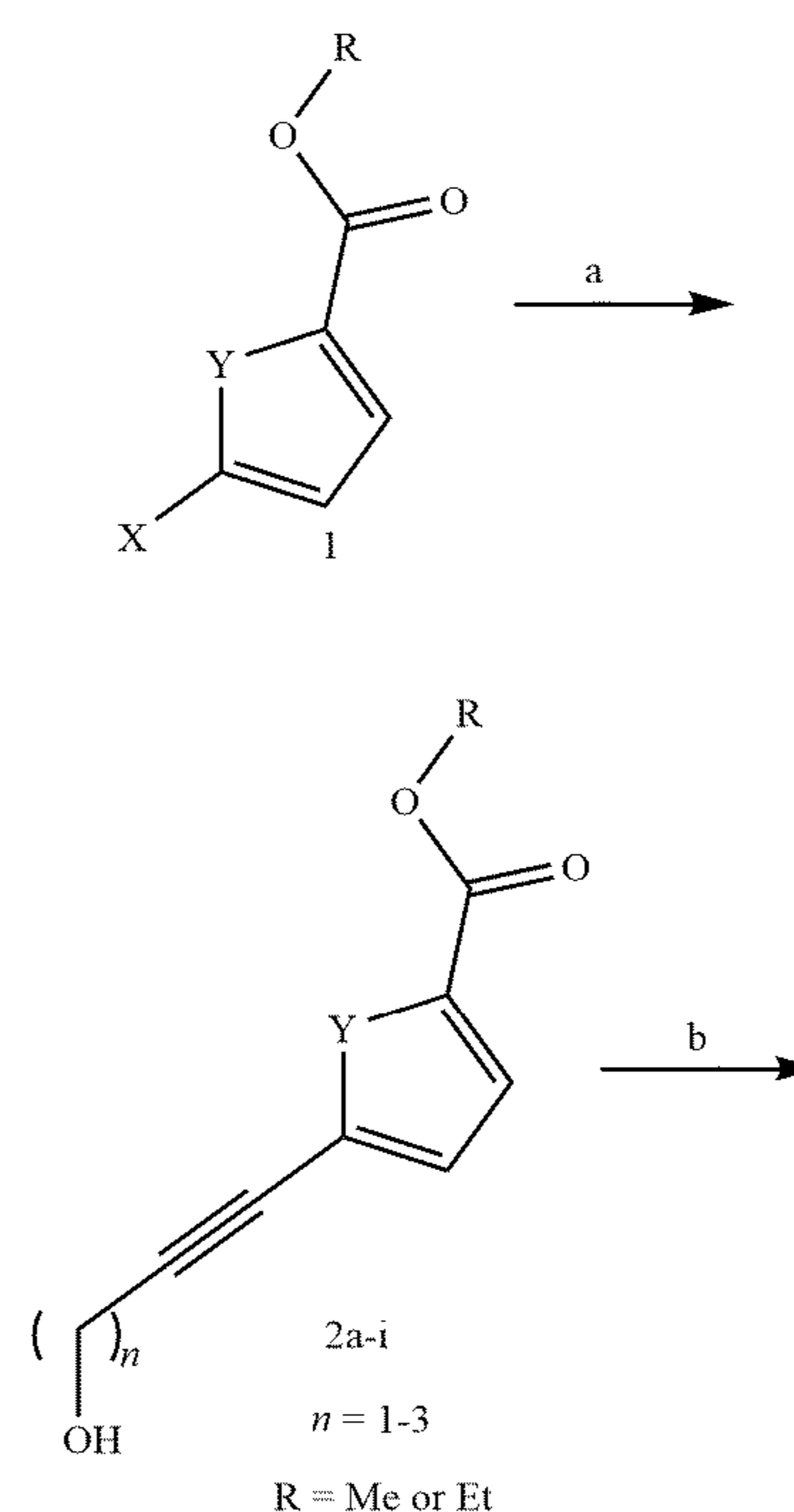
Synthetic Scheme
