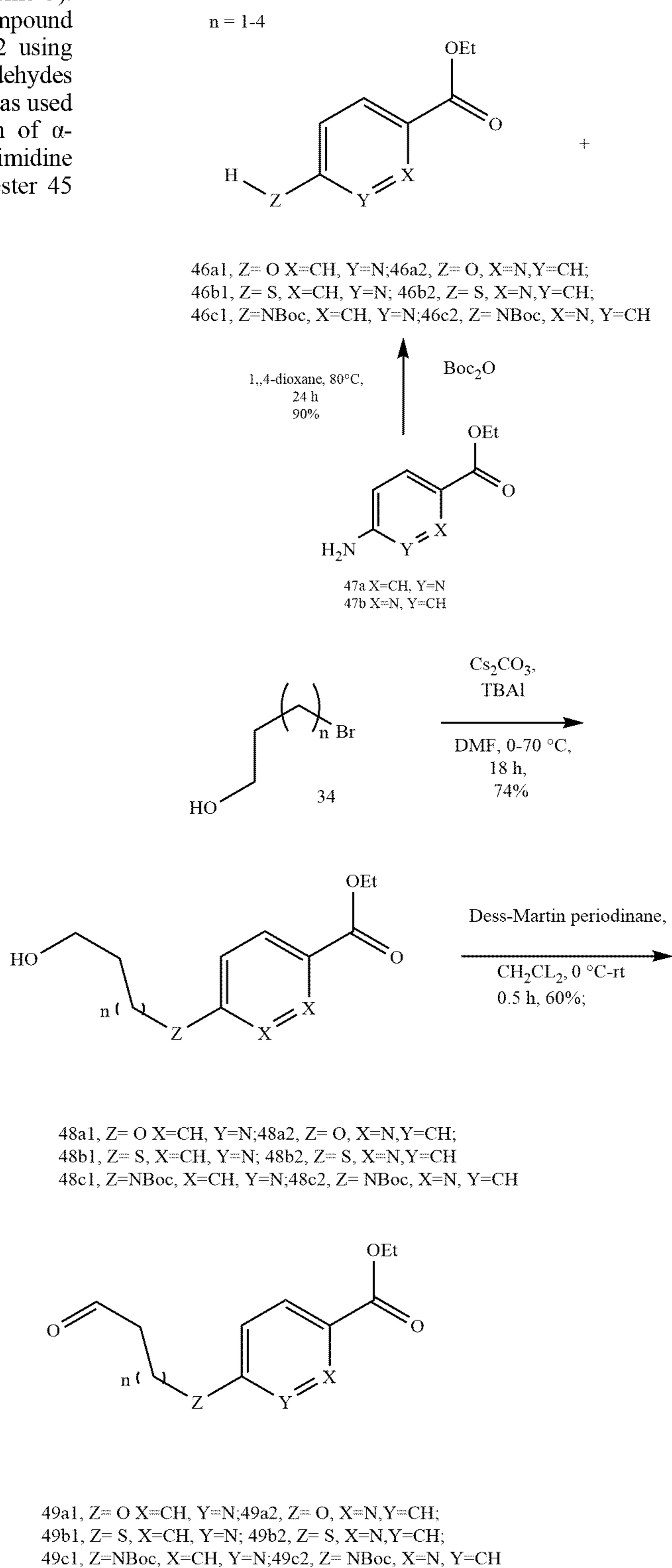
Scheme 6
