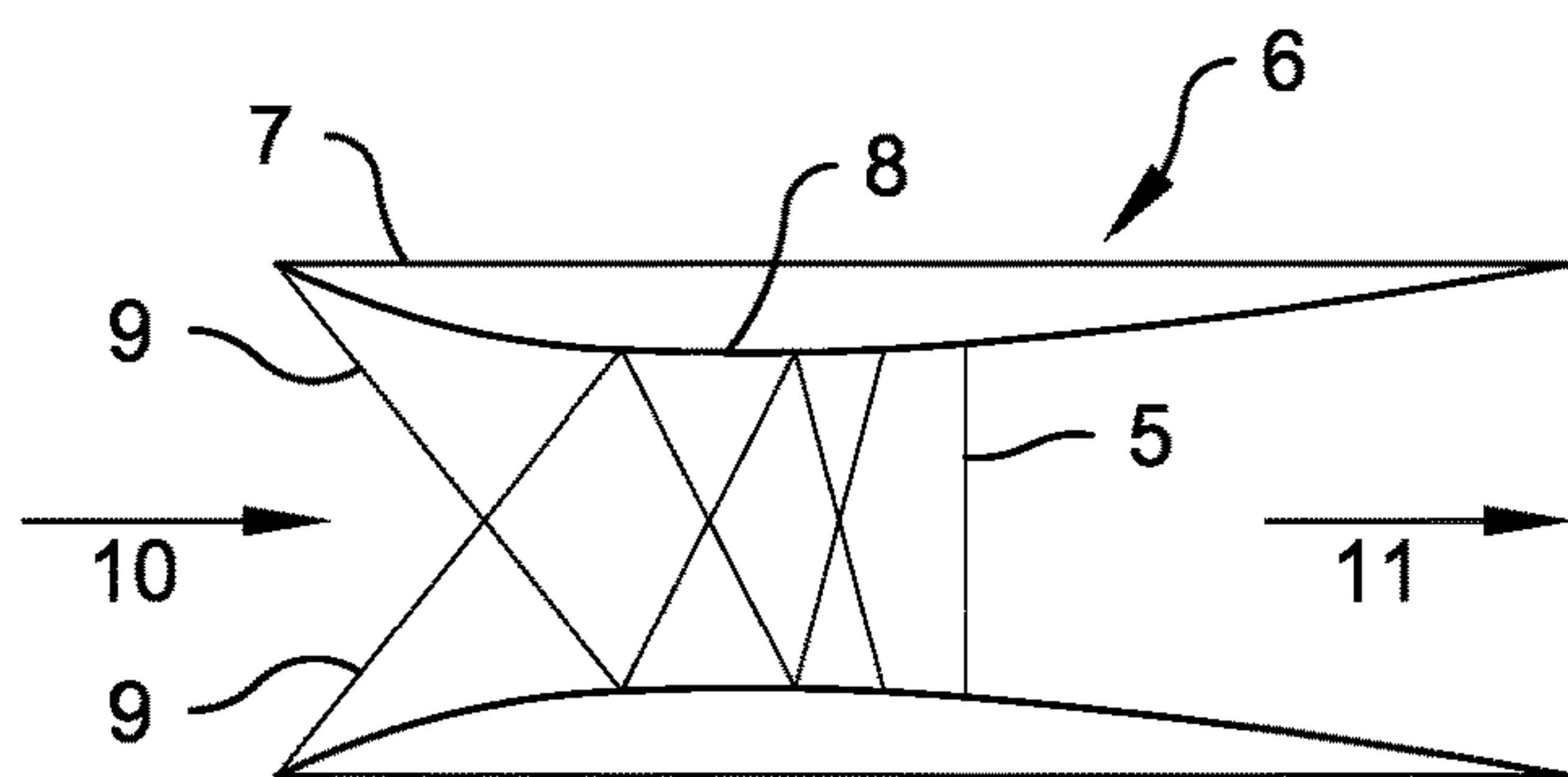
Fig. 1 (Prior Art)
