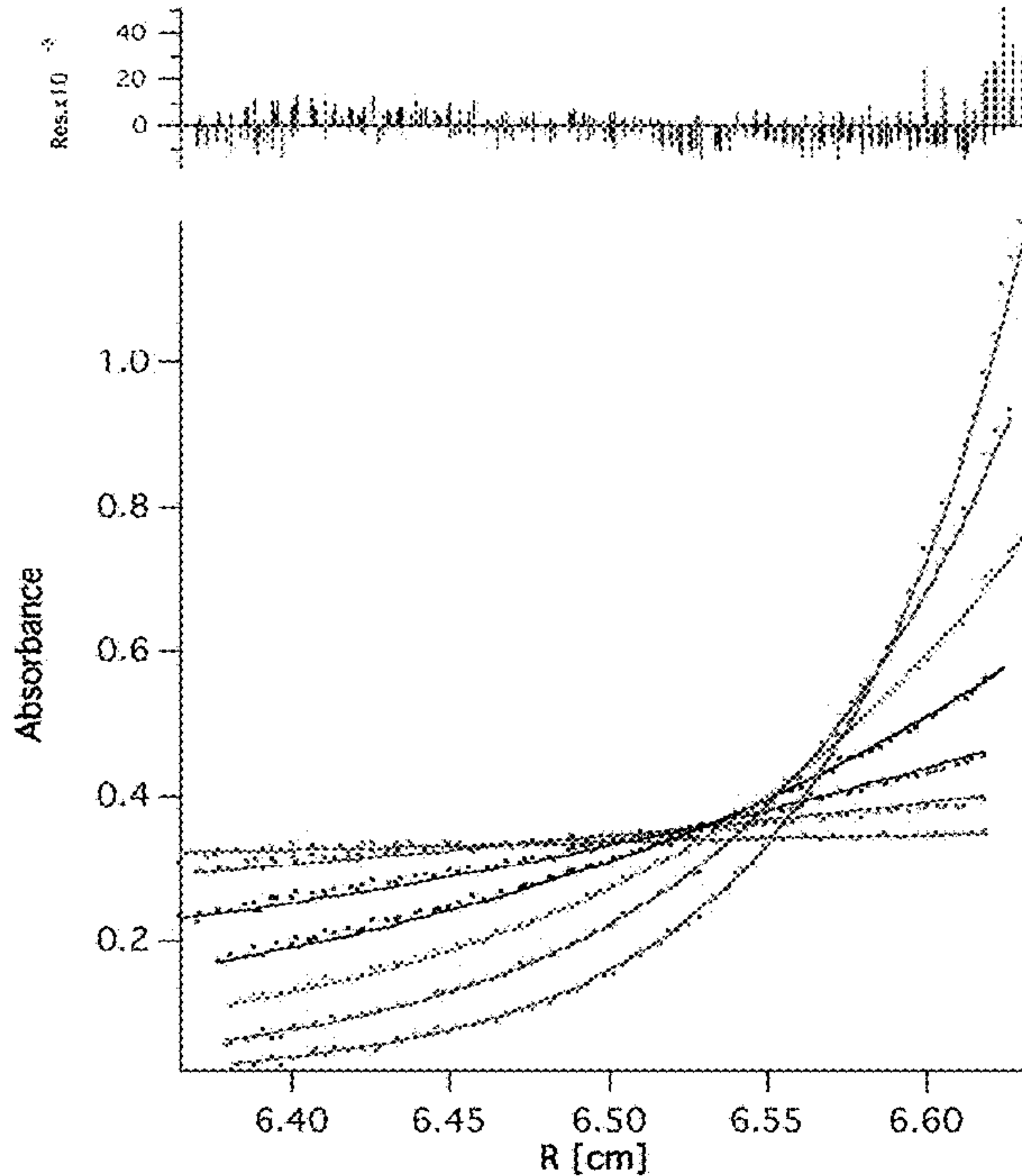
Fig. 36C. trastuzumab fab
