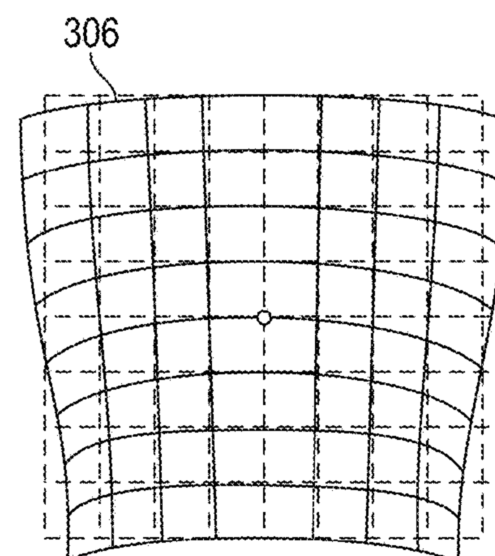
Tangential Distortion
