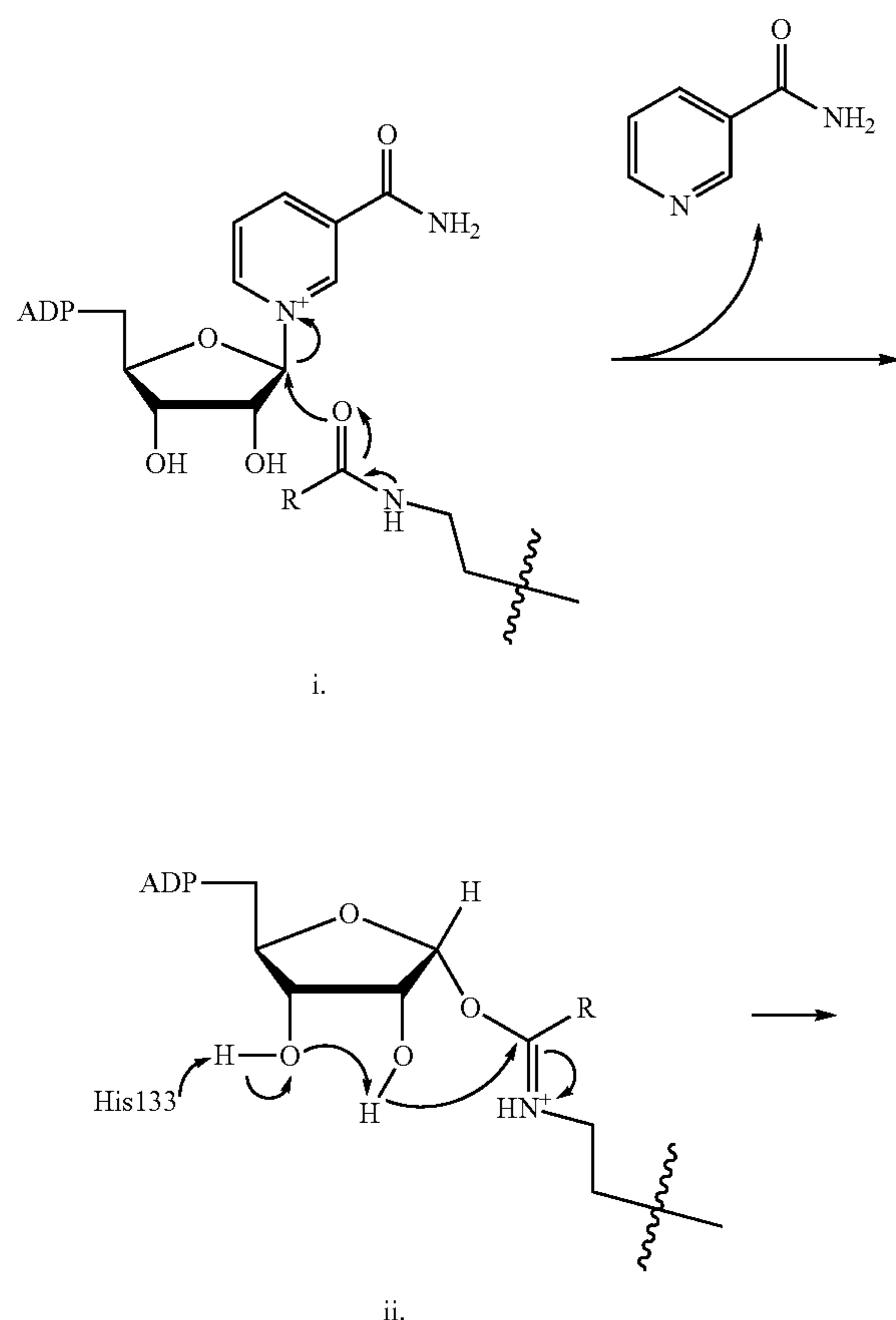
Scheme 2
