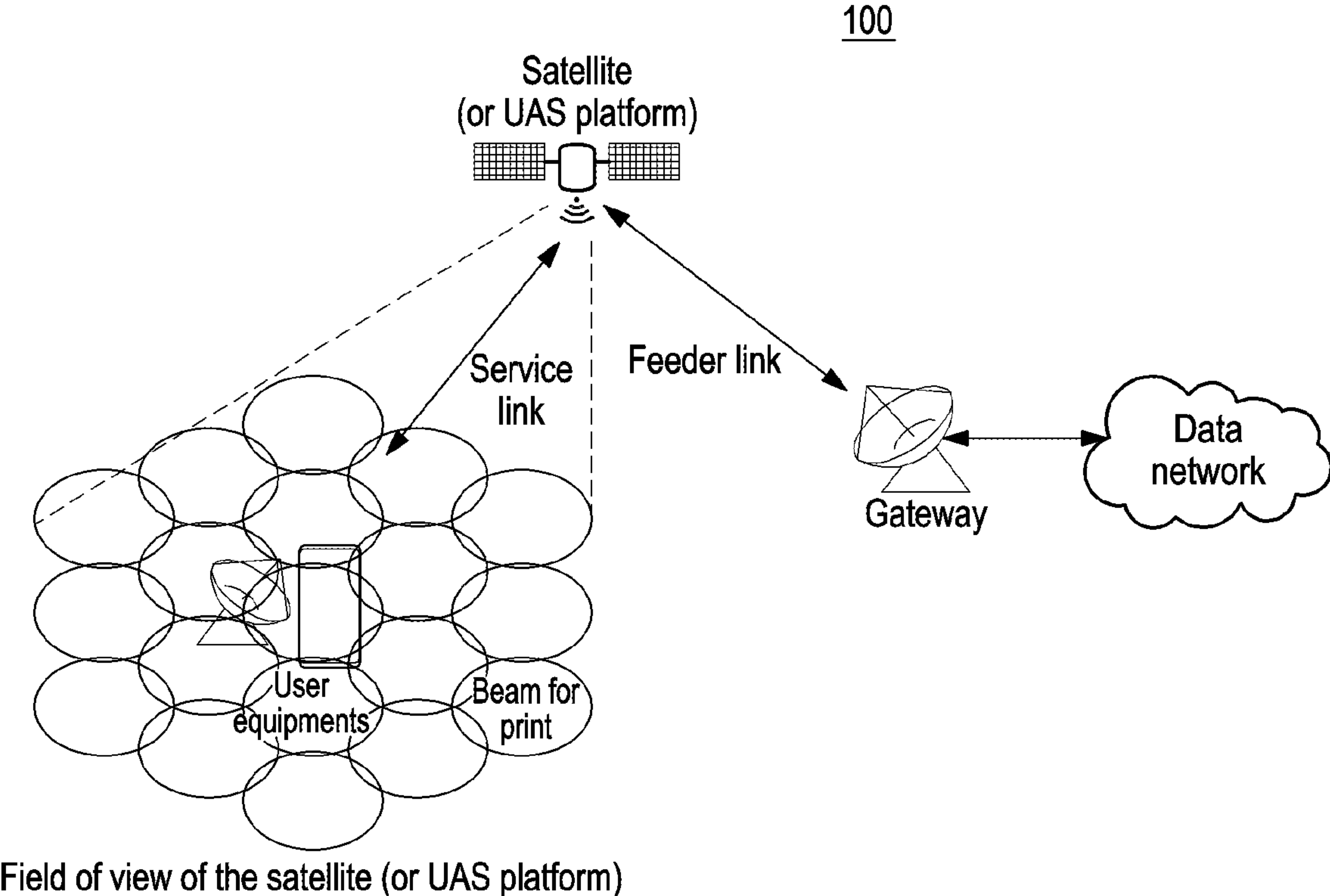
FIG. 1 (CONVENTIONAL ART)
