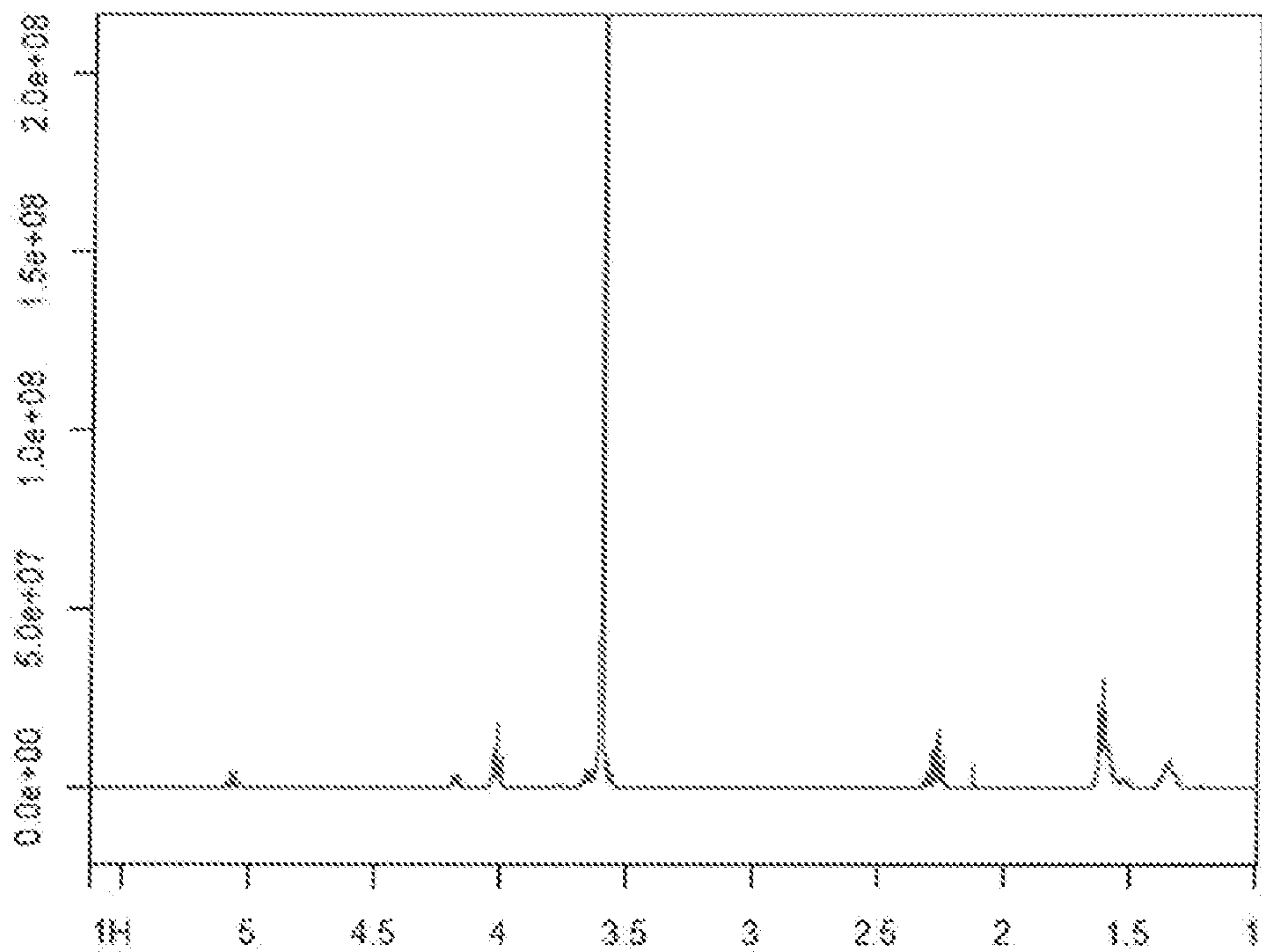
Figure 7: Proton nuclear magnetic resonance spectrum of PCL 4 -PEG 23 -PCL 4 .
