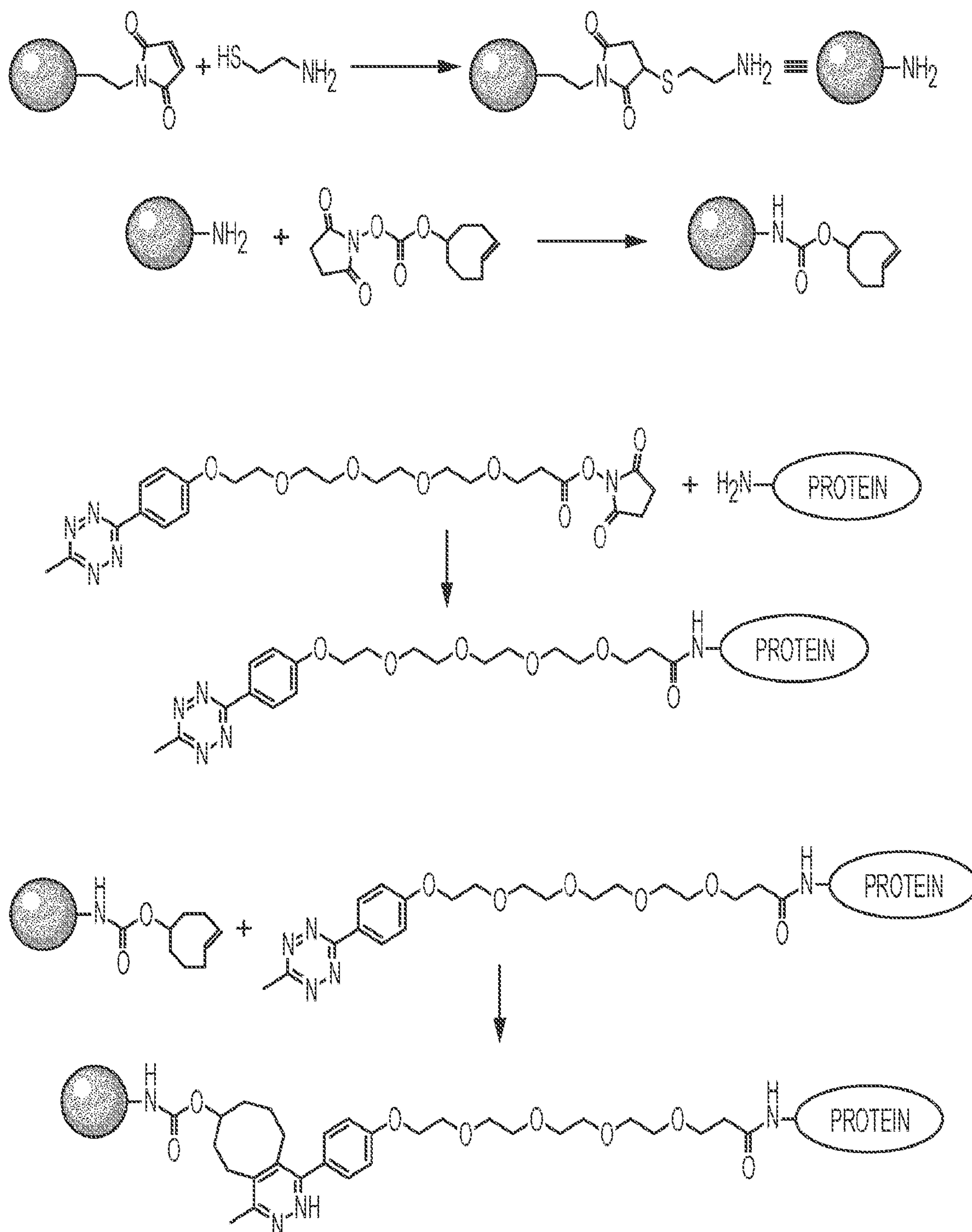
SCHEME 2. ALKENE-TETRAZINE CHEMISTRY
