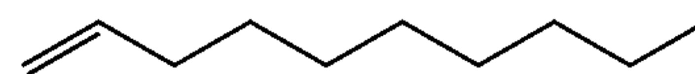
1-Decene C_{10}H_{20} BP = 172° C., Vapor Pressure: 1.67 mmHg at 25° C.
