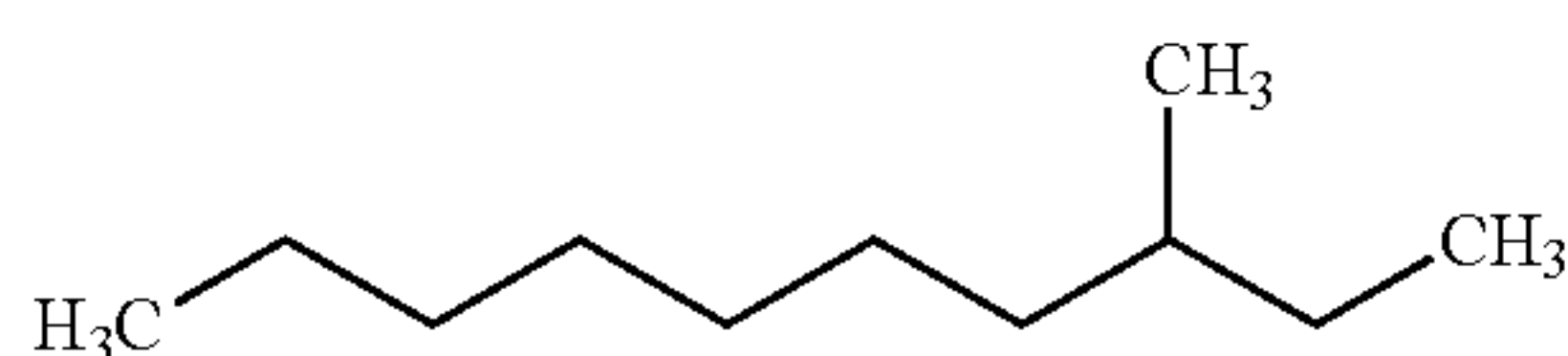
3-Methyldecane C_{11}H_{24} BP = 188° C., Vapor Pressure: N/A
