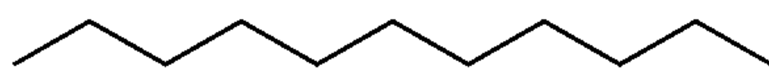
n-Dodecane C_{12}H_{26} BP = 216° C., Vapor Pressure: 0.14 mmHg at 25° C.
