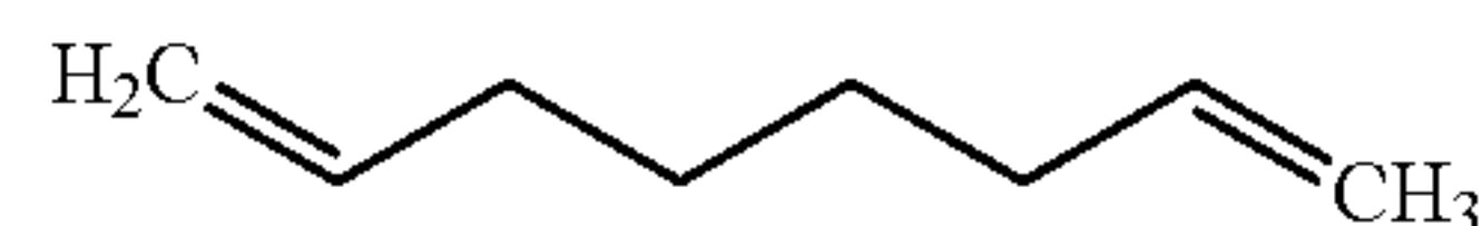
1,7-Octadiene C_8H_{14} BP = 118° C., Vapor Pressure: 19 mmHg at 25° C.
