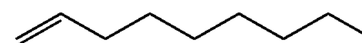
1-Nonene C_9H_{18} BP = 146° C., Vapor Pressure: 11 mmHg at 37.7° C.
