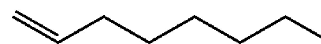
1-Octene C_8H_{16} BP = 122° C., Vapor Pressure: 36 mmHg at 37.7° C.
