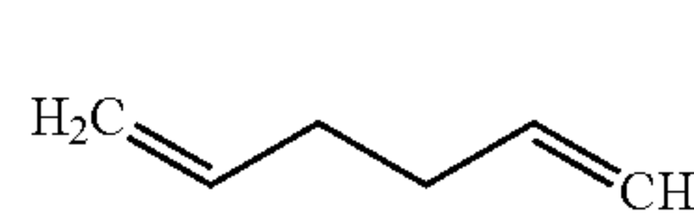
1,5-Hexadiene C_6H_{10} BP = 60° C., Vapor Pressure: 367 mmHg at 37.7° C.
