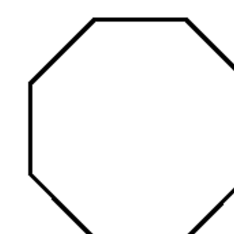
Cyclooctane C_8H_{16} BP = 149° C., Vapor Pressure: 16 mmHg at 37.7° C.
