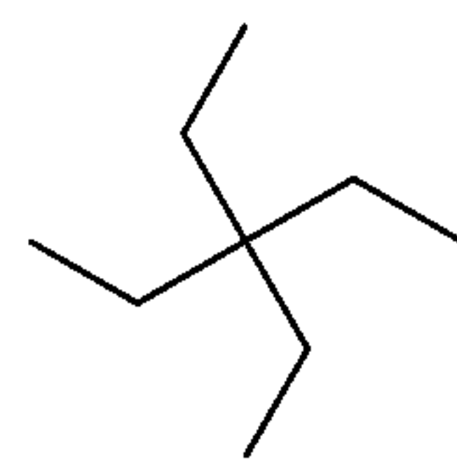
Tetraethylmethane C_9H_{20} BP = 146° C., Vapor Pressure: 7.3 mmHg at 25° C.
