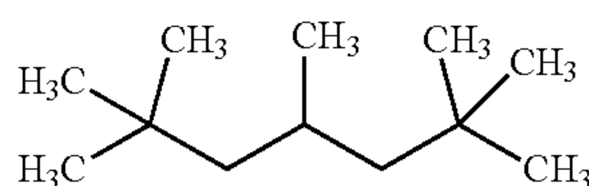
Isododecane C_{12}H_{26} BP = 180° C., Vapor Pressure: 0.301 mmHg at 20° C.
