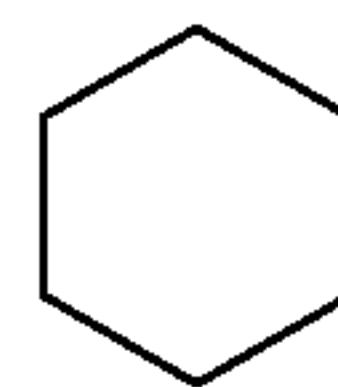
Cyclohexane C_6H_{12} BP = 81° C., Vapor Pressure: 78 mmHg at 20° C.
