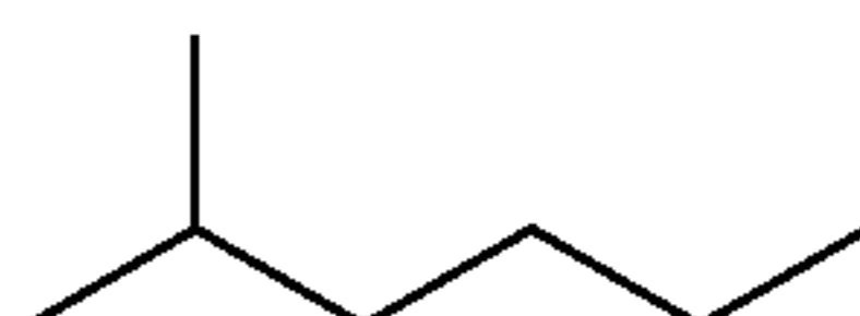
Isoheptane C_7H_{16} BP = 90° C., Vapor Pressure: 66 mmHg at 20° C.
