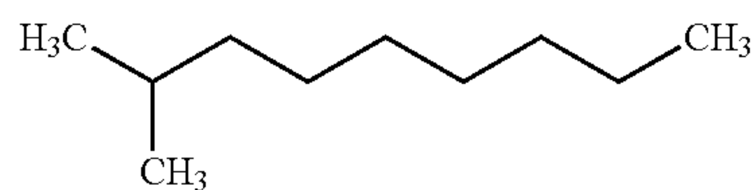
Isodecane C_{10}H_{22} BP = 167° C., Vapor Pressure: 2.3 mmHg at 25° C.
