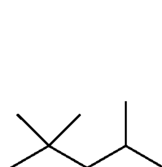
Isooctane C_8H_{18} BP = 99° C., Vapor Pressure: 41 mmHg at 21° C.
