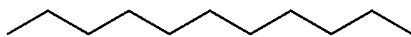
n-Undecane C_{11}H_{24} BP = 196° C., Vapor Pressure: 0.4 mmHg at 25° C.
