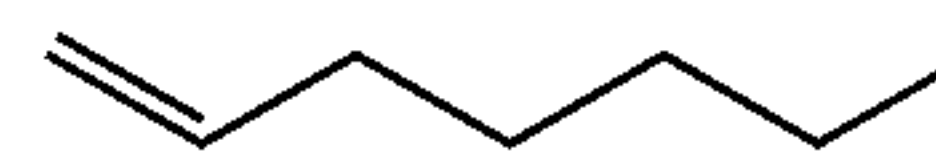
1-Heptene C_7H_{14} BP = 94° C., Vapor Pressure: 101 mmHg at 37.7° C.
