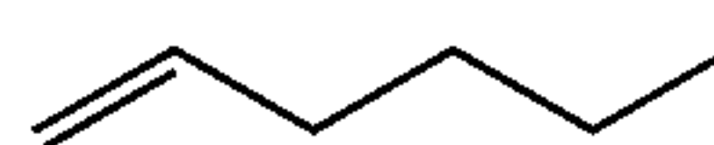
1-Hexene C_6H_{12} BP = 64° C., Vapor Pressure: 155 mmHg at 21° C.
