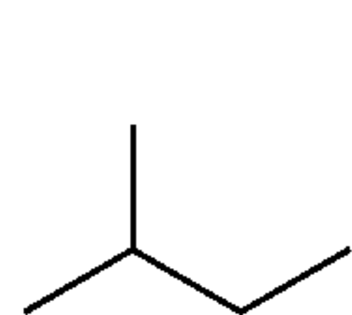
Isopentane C_5H_{12} BP = 28° C., Vapor Pressure: 577 mmHg at 20° C.
