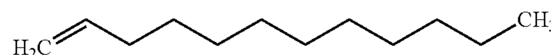
1-Dodecene C_{12}H_{24} BP = 214° C., Vapor Pressure: N/A
