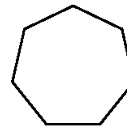
Cycloheptane C_7H_{14} BP = 118° C., Vapor Pressure: 22 mmHg at 20° C.
