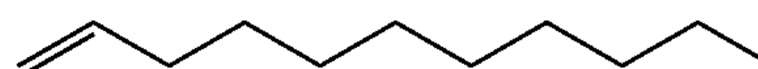
1-Undecene C_{11}H_{22} BP = 192° C., Vapor Pressure: N/A
