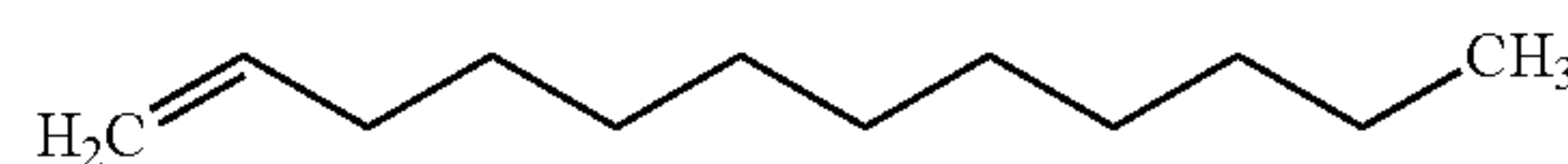
1-Dodecene C_{12}H_{24} BP = 214° C., Vapor Pressure: N/A
