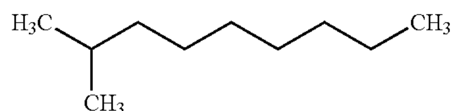
Isodecane C_{10}H_{22} BP = 167° C., Vapor Pressure: 2.3 mmHg at 25° C.
