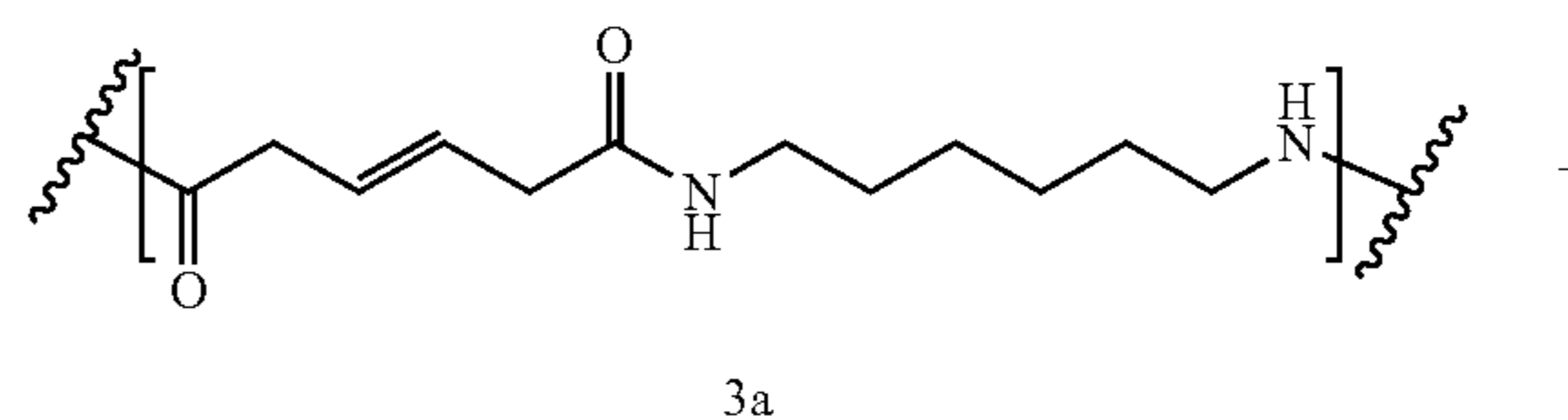
Scheme 24
