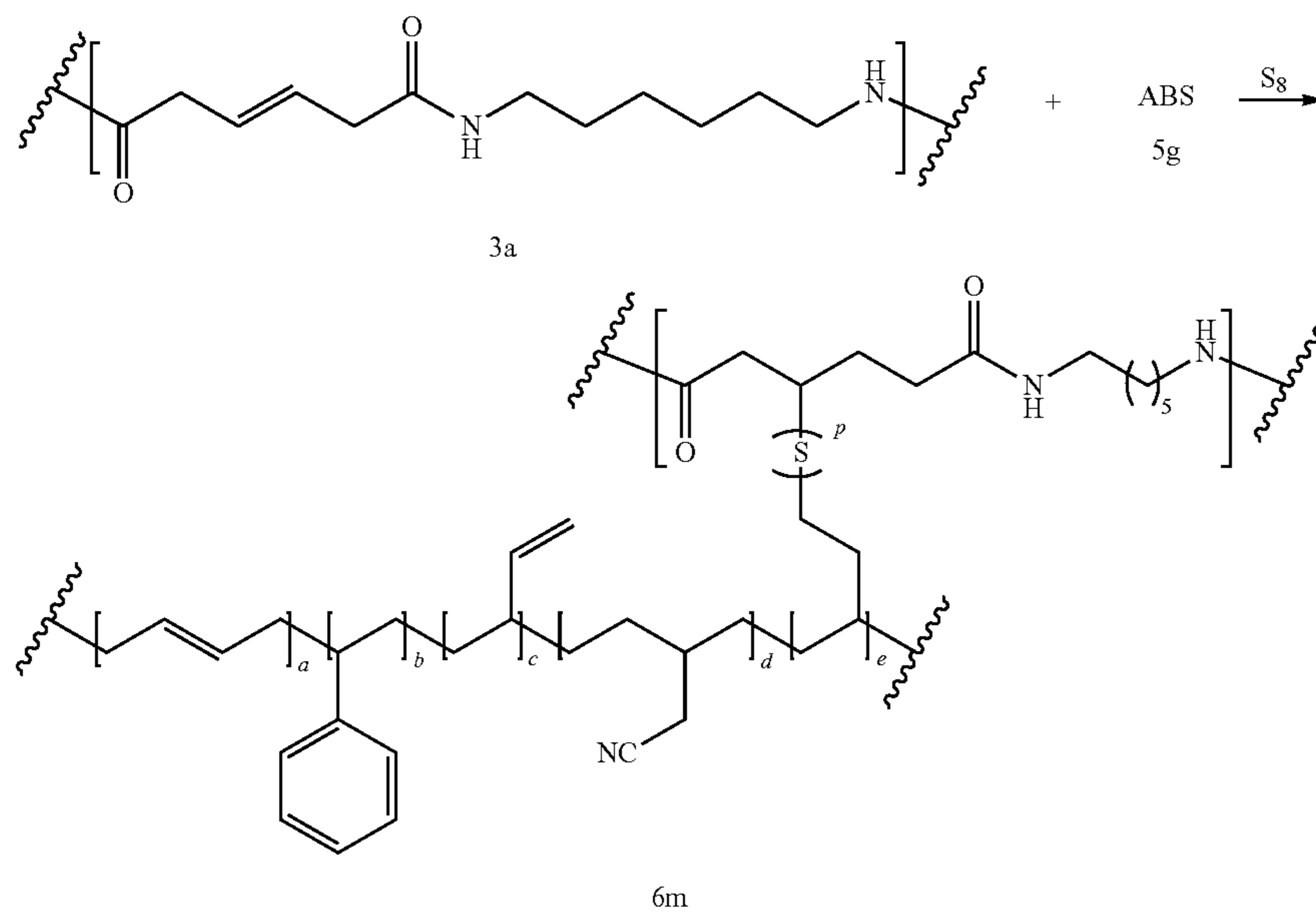
Scheme 22
