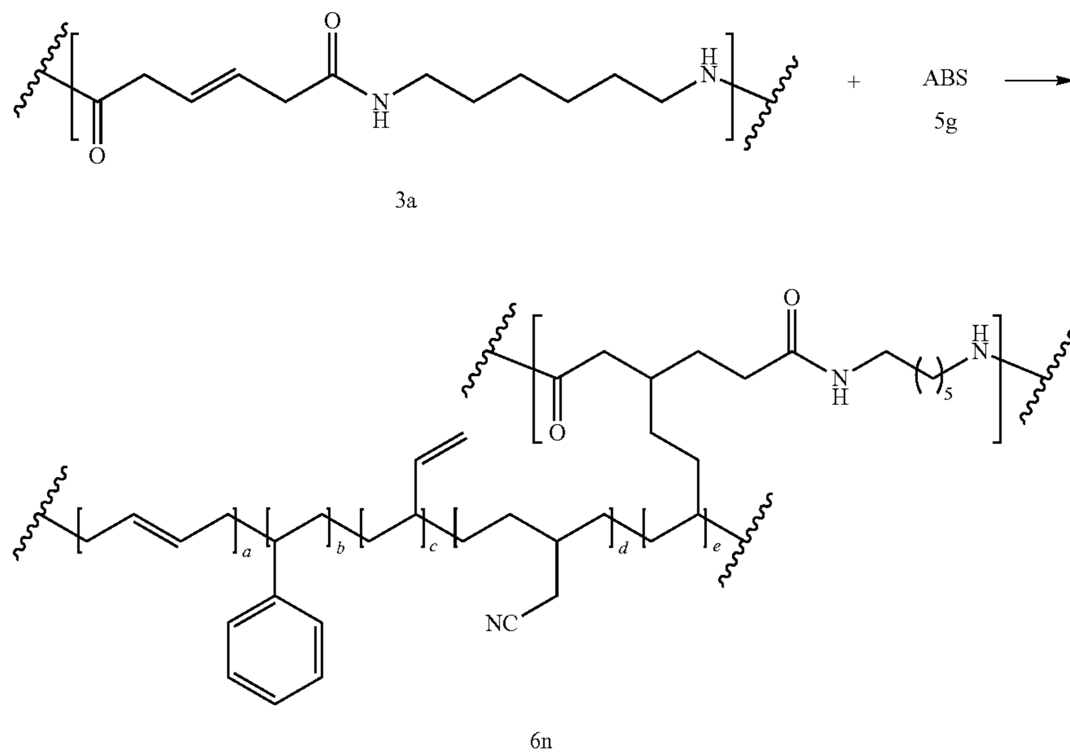
Scheme 23
