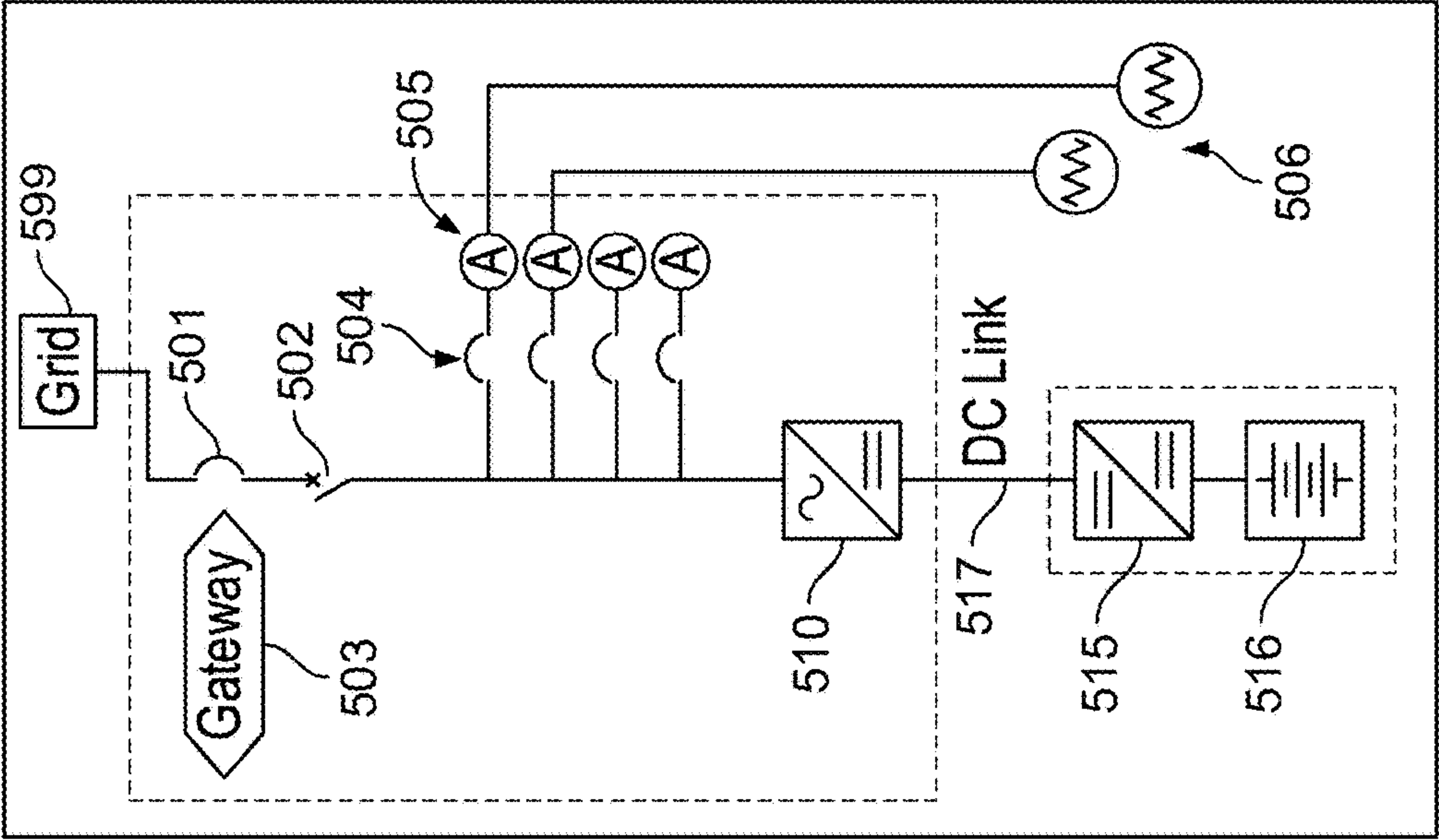
DC-coupled Storage Battery
