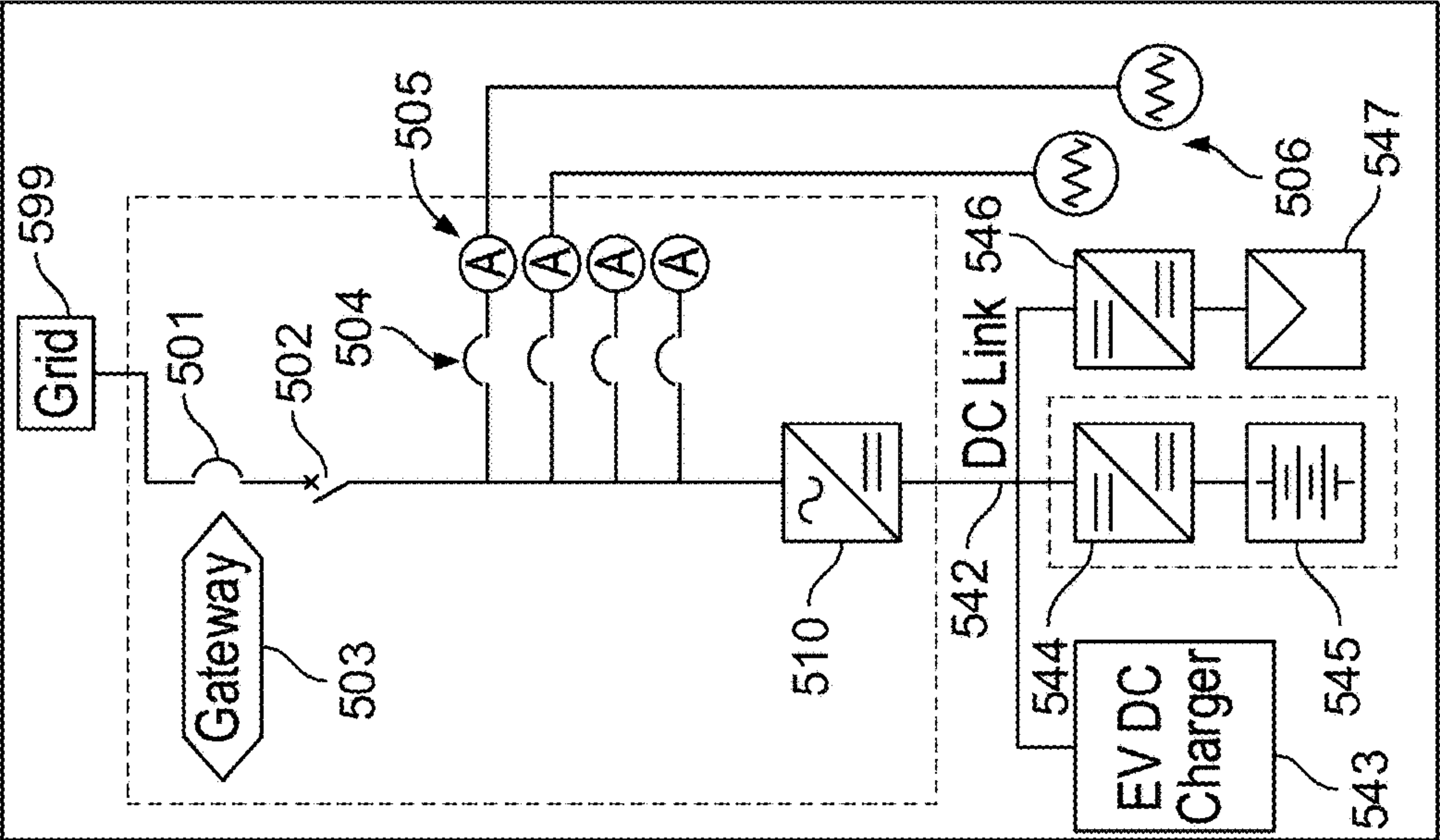
DC-coupled Storage, PV, and EV Charger
