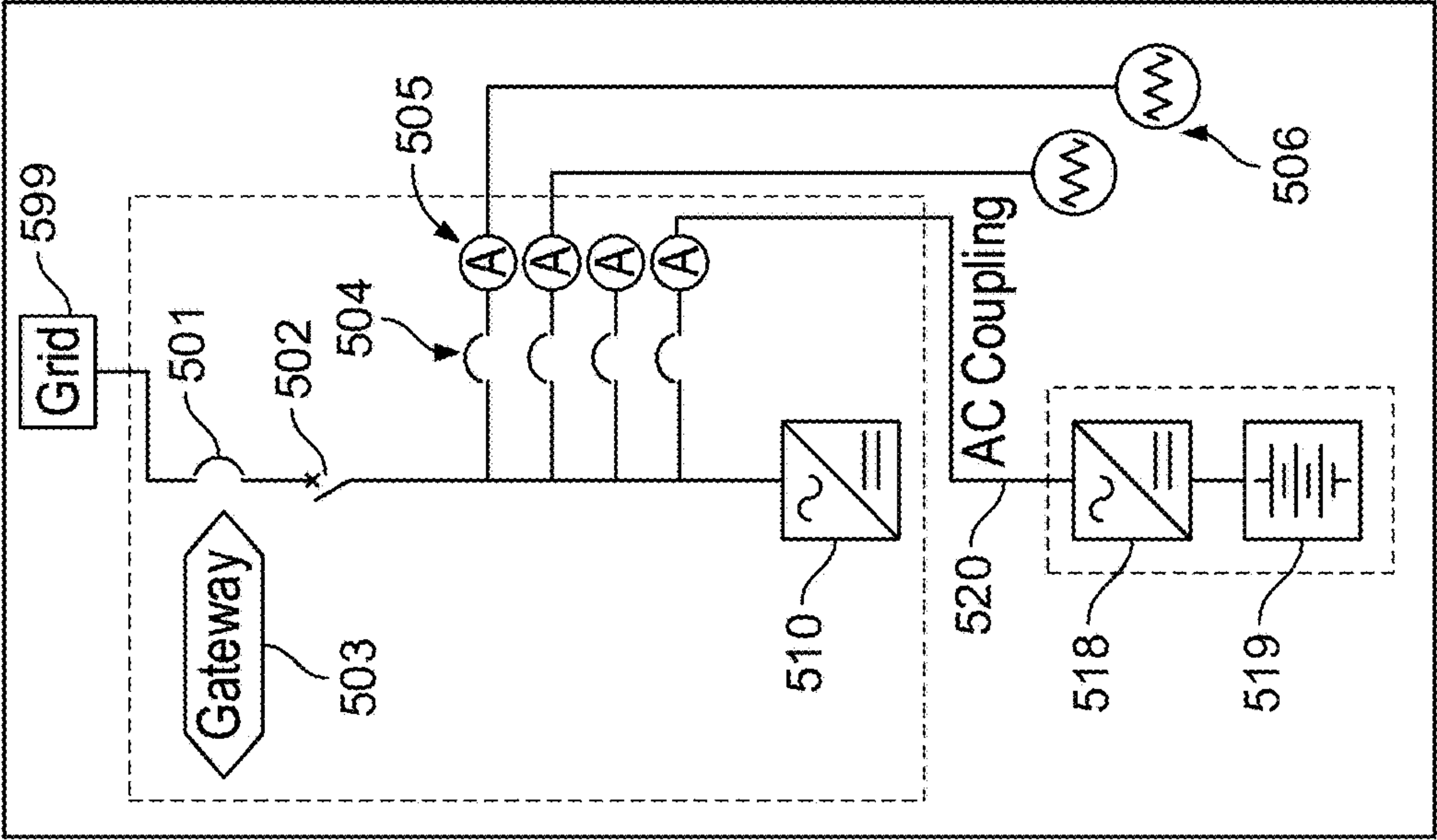
AC-coupled Storage Battery
