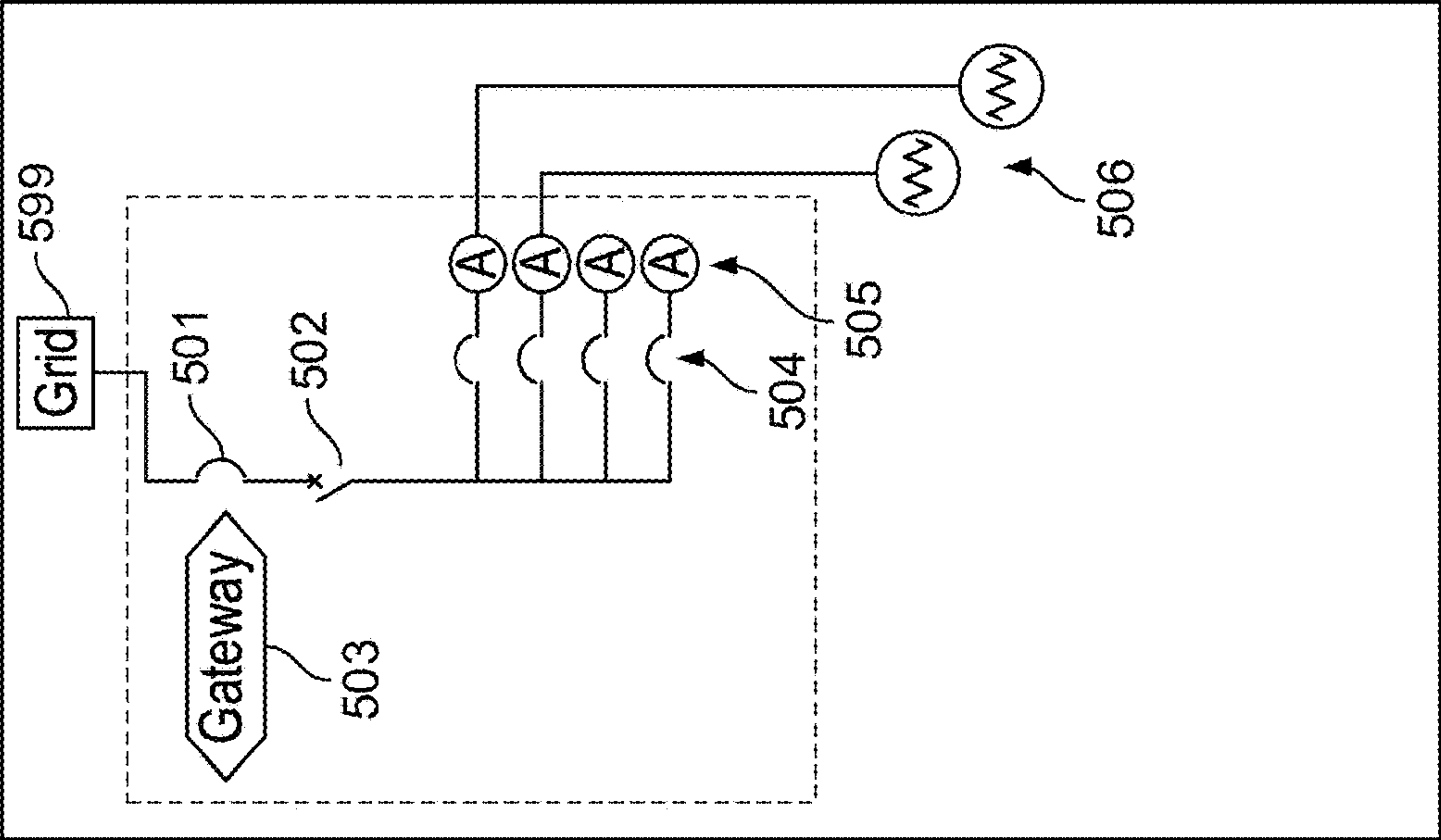
500 Standalone Panel for Control & Metering
