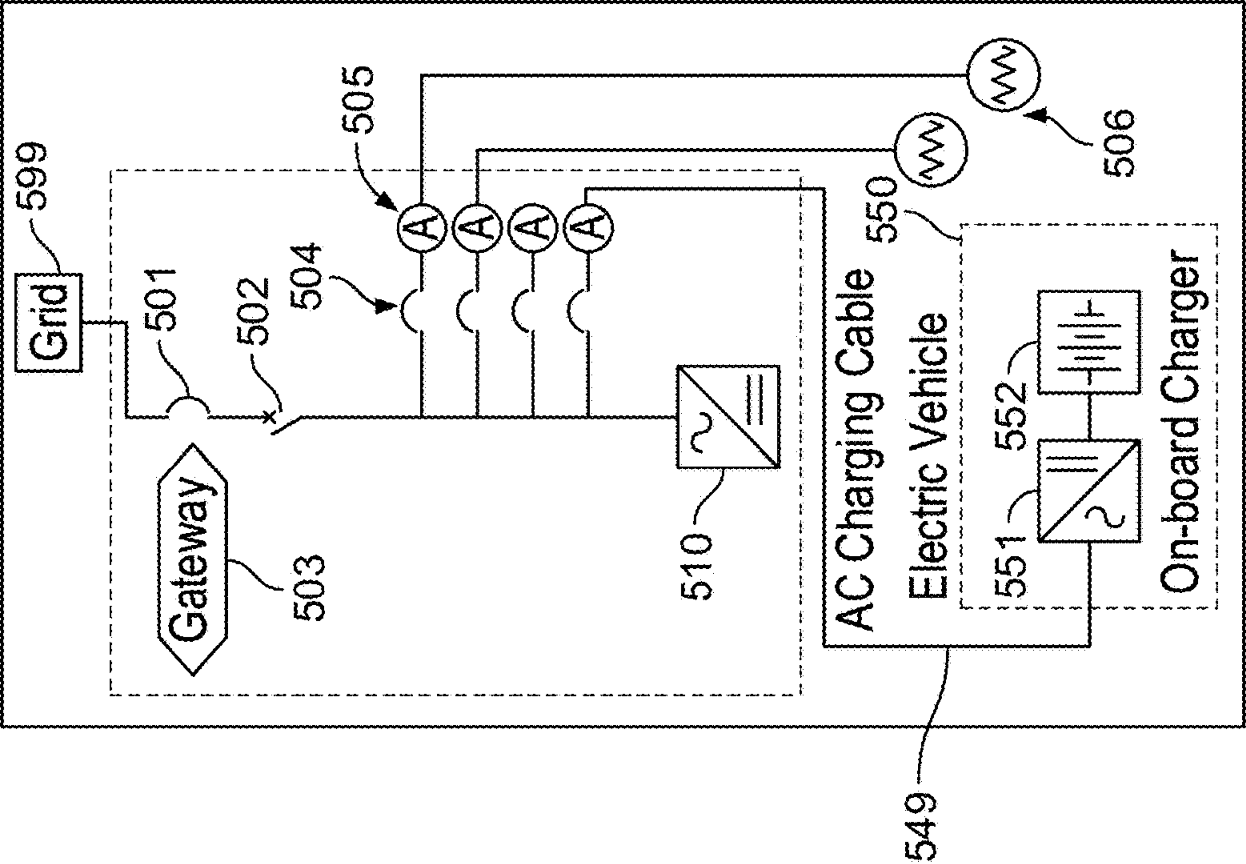
AC-coupled Vehicle Charging
