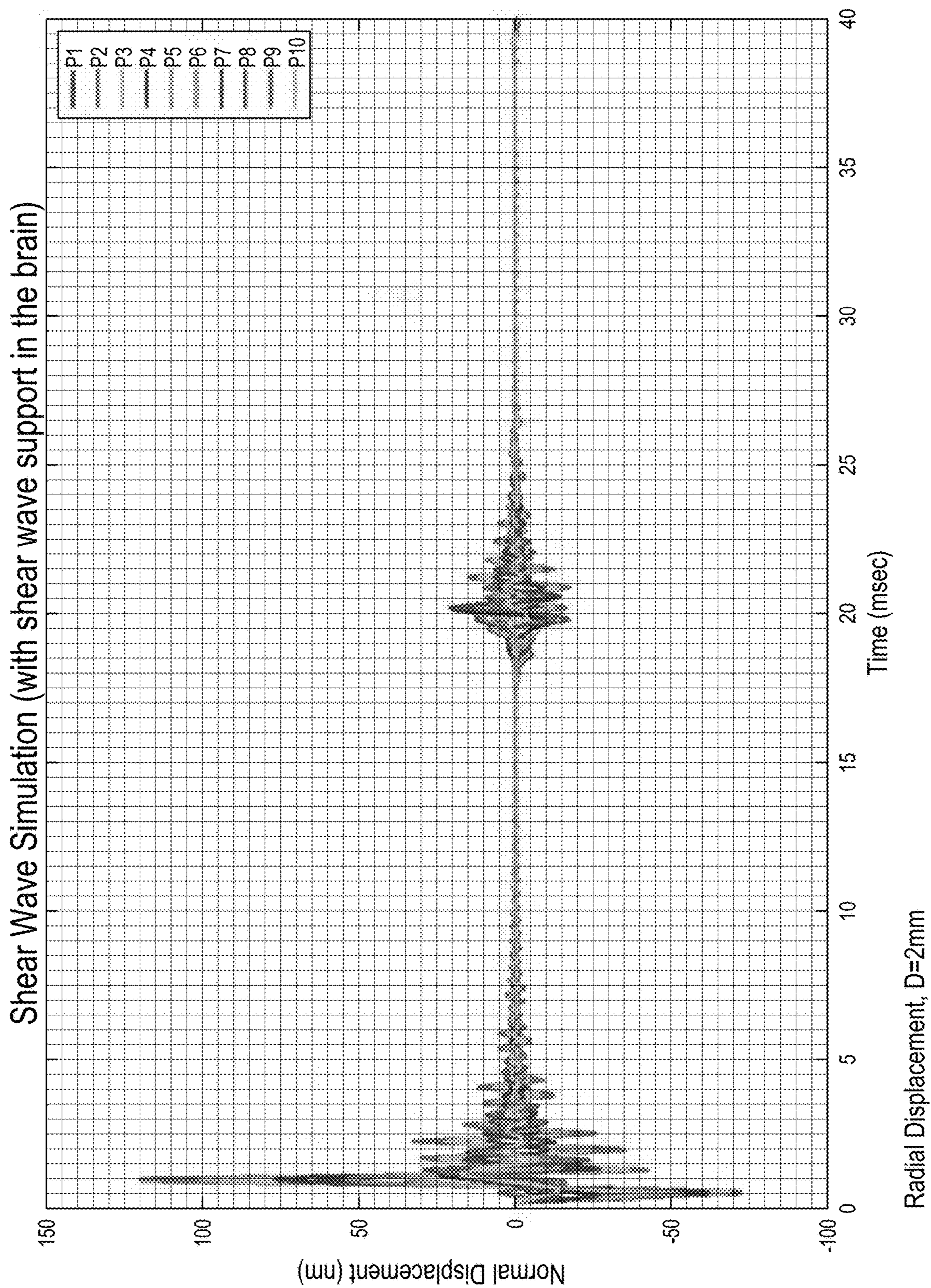
Radial Displacement, D=2mm
