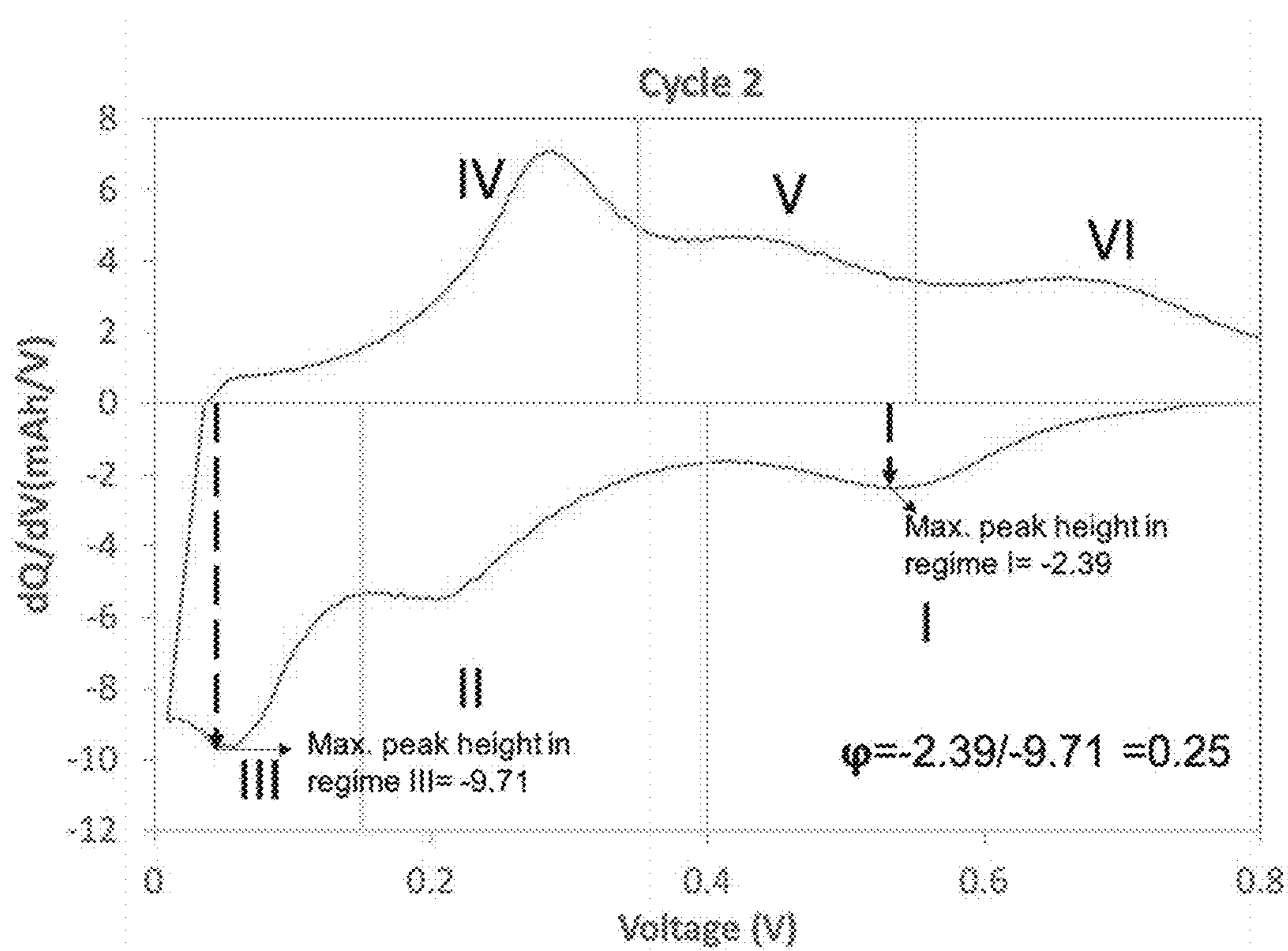
Figure 5. Example of calculation of \phi for Silicon-Carbon Composite 3.
