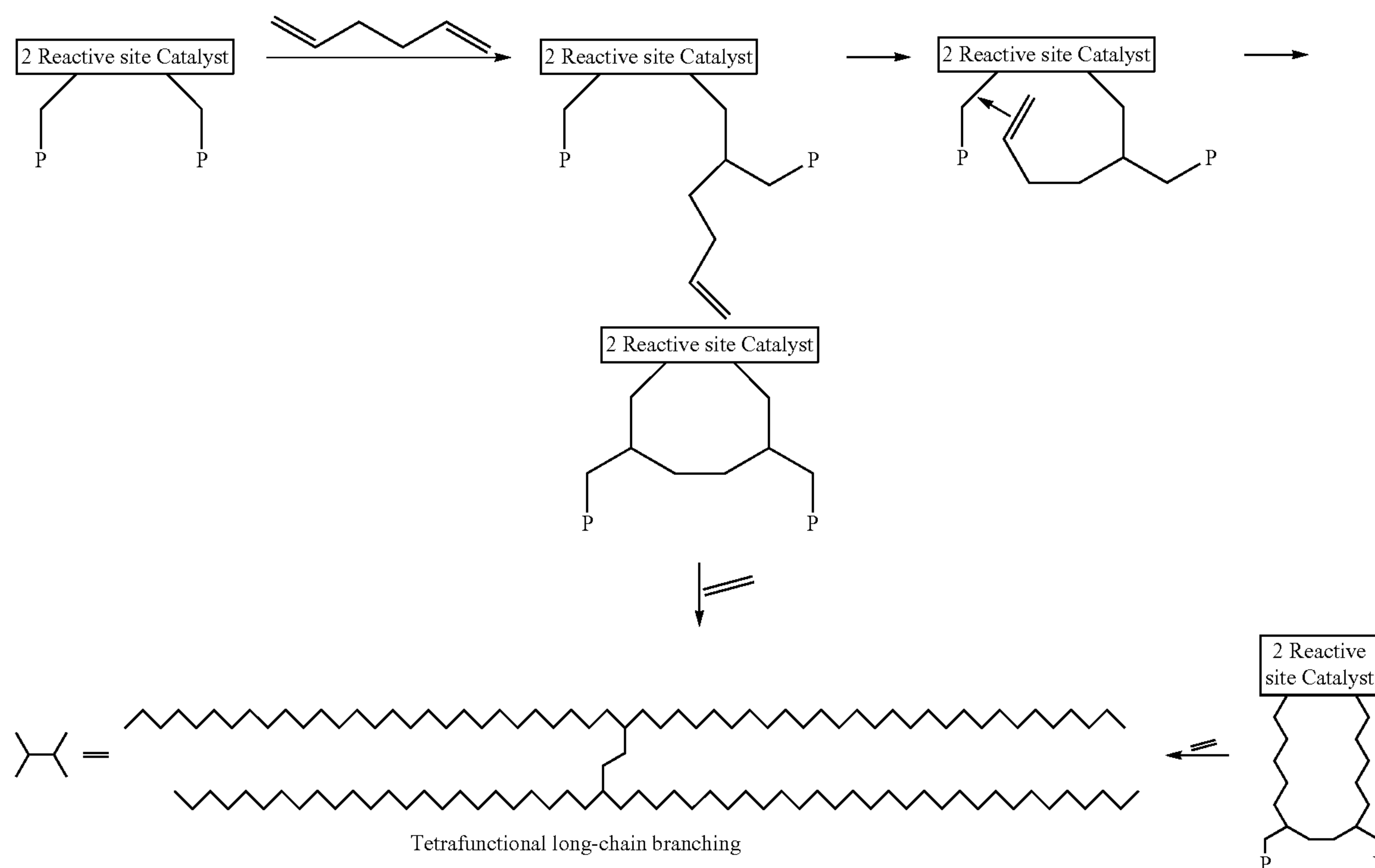
Scheme 3: Depiction of incorporating the diene in a concerted fashion (P is a polymer chain), also called the "Ladder Branching" mechanism.
