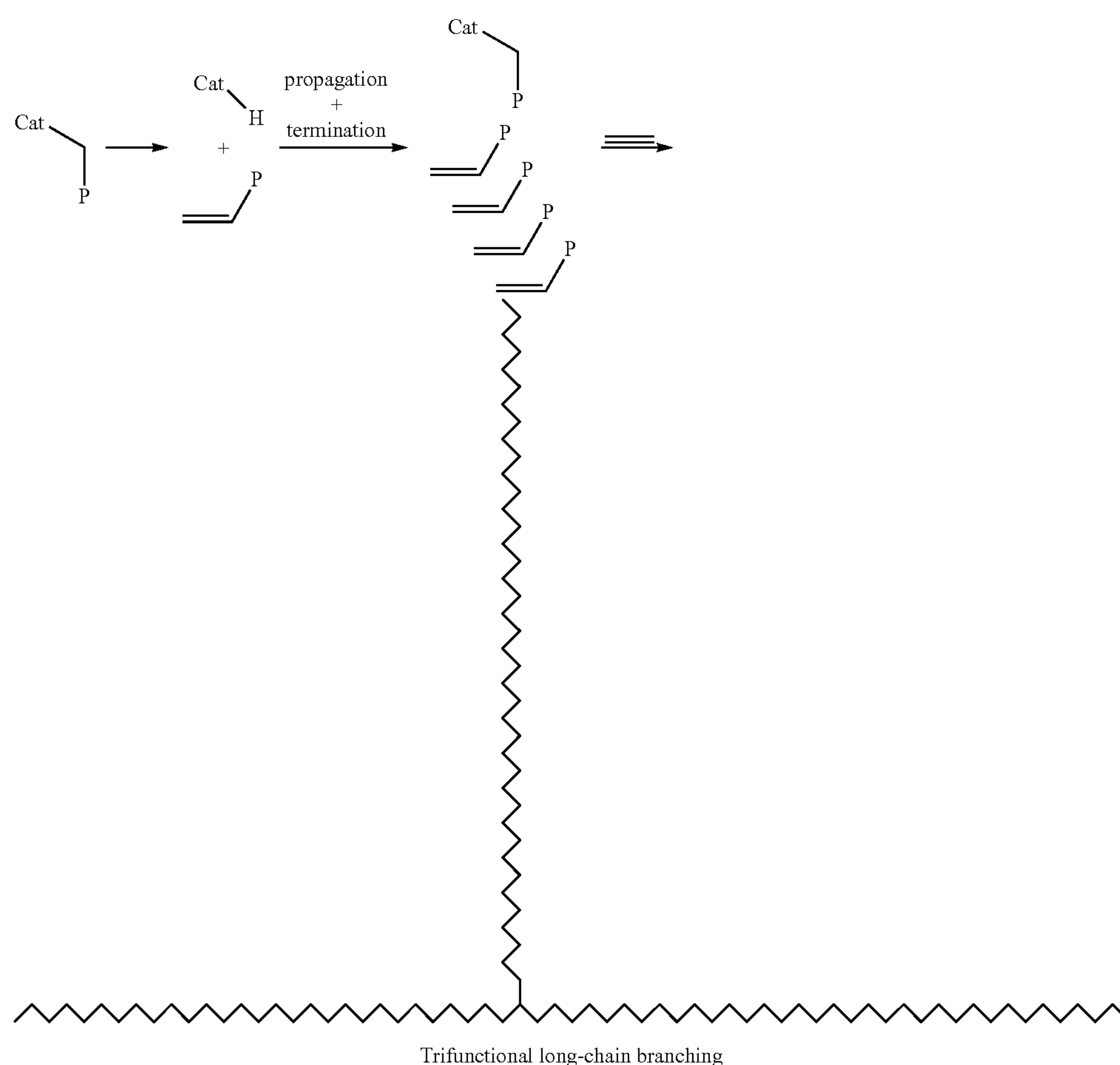
Scheme 1: Naturally occurring long-chain branching: Chain transfer event leading to vinyl terminated polymers
