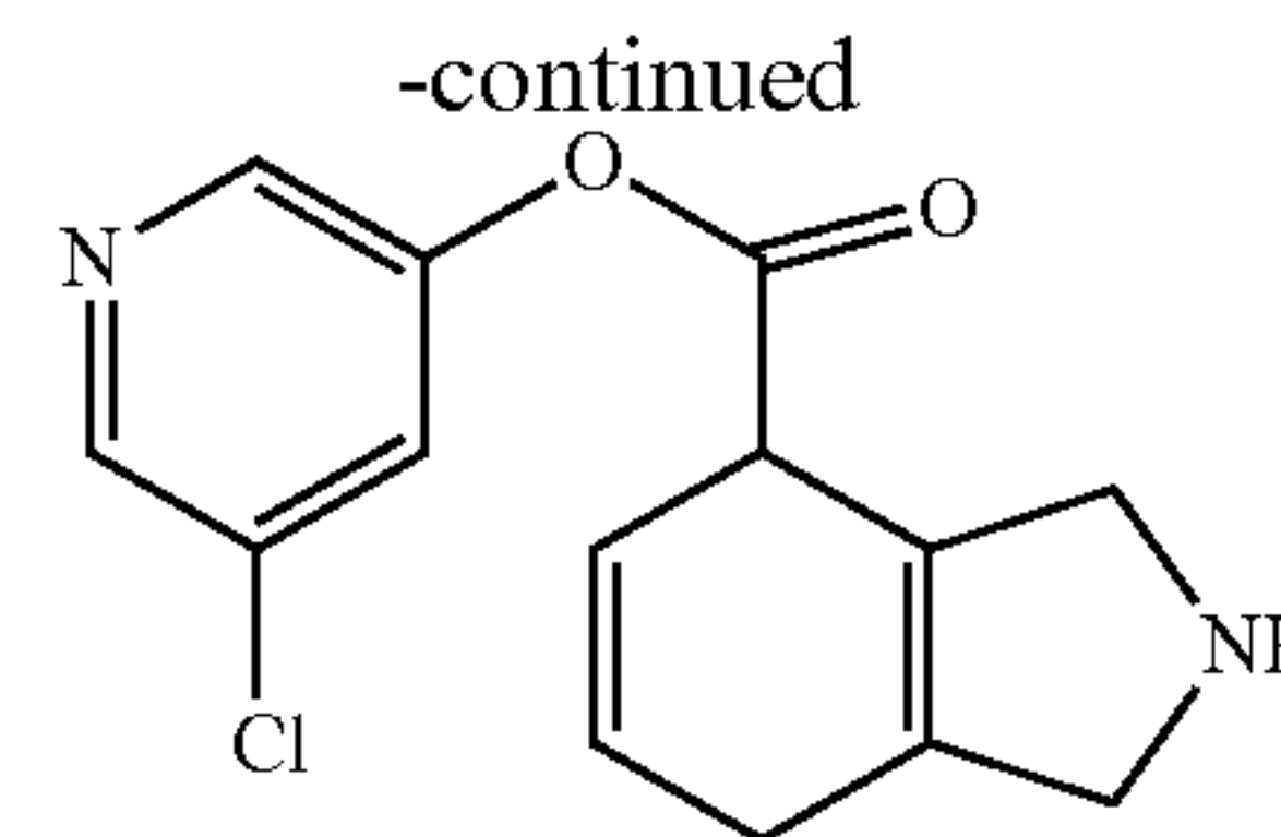
Reference Molecule
