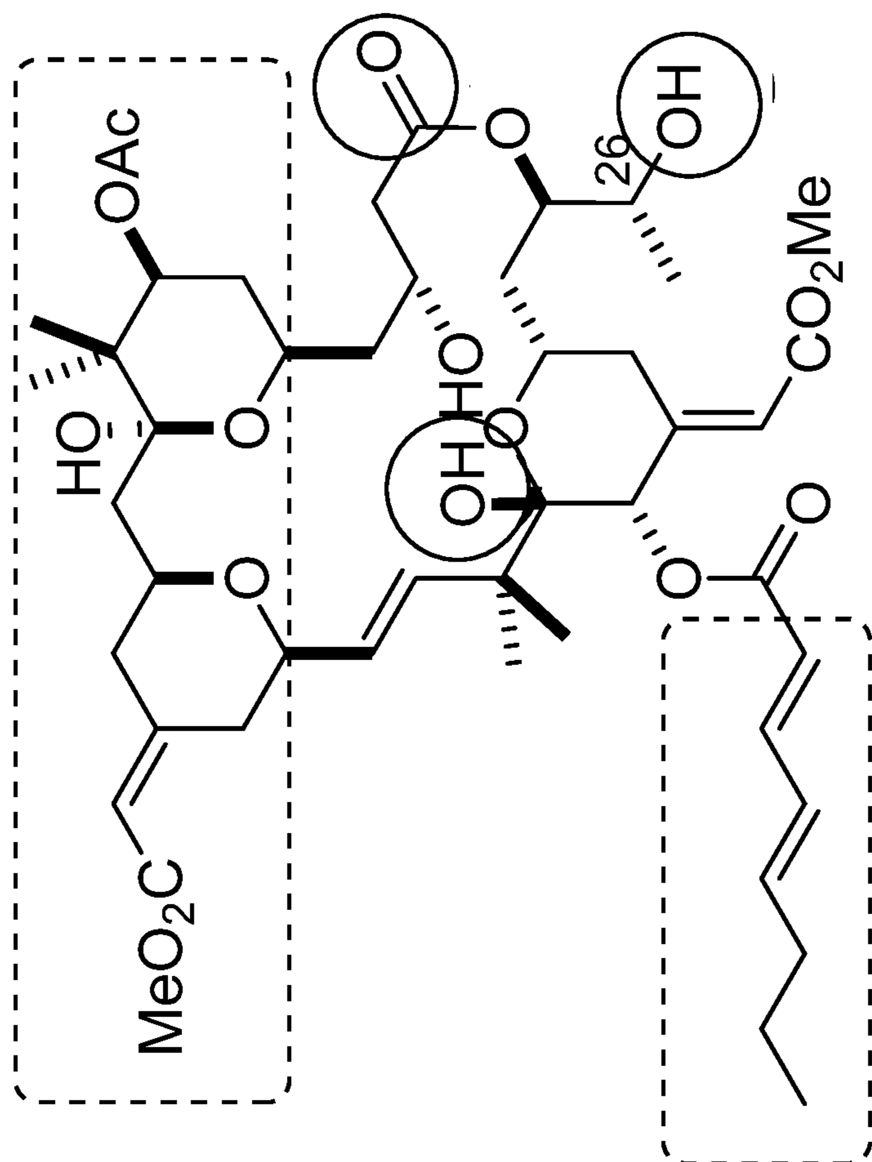
Bryostatin 1
