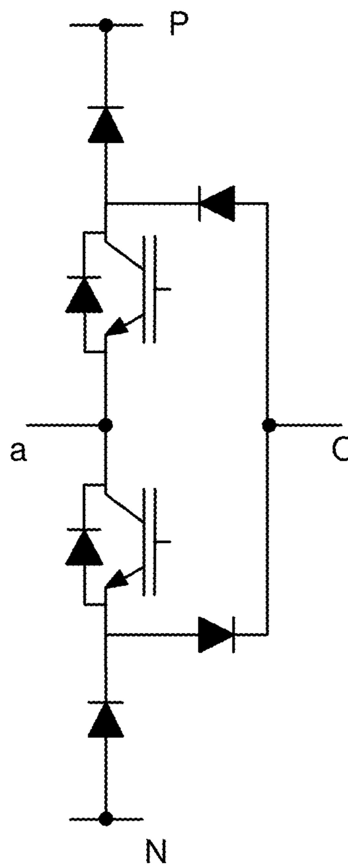
Conventional Type 3 Level (NPC Type with Rectifier)
