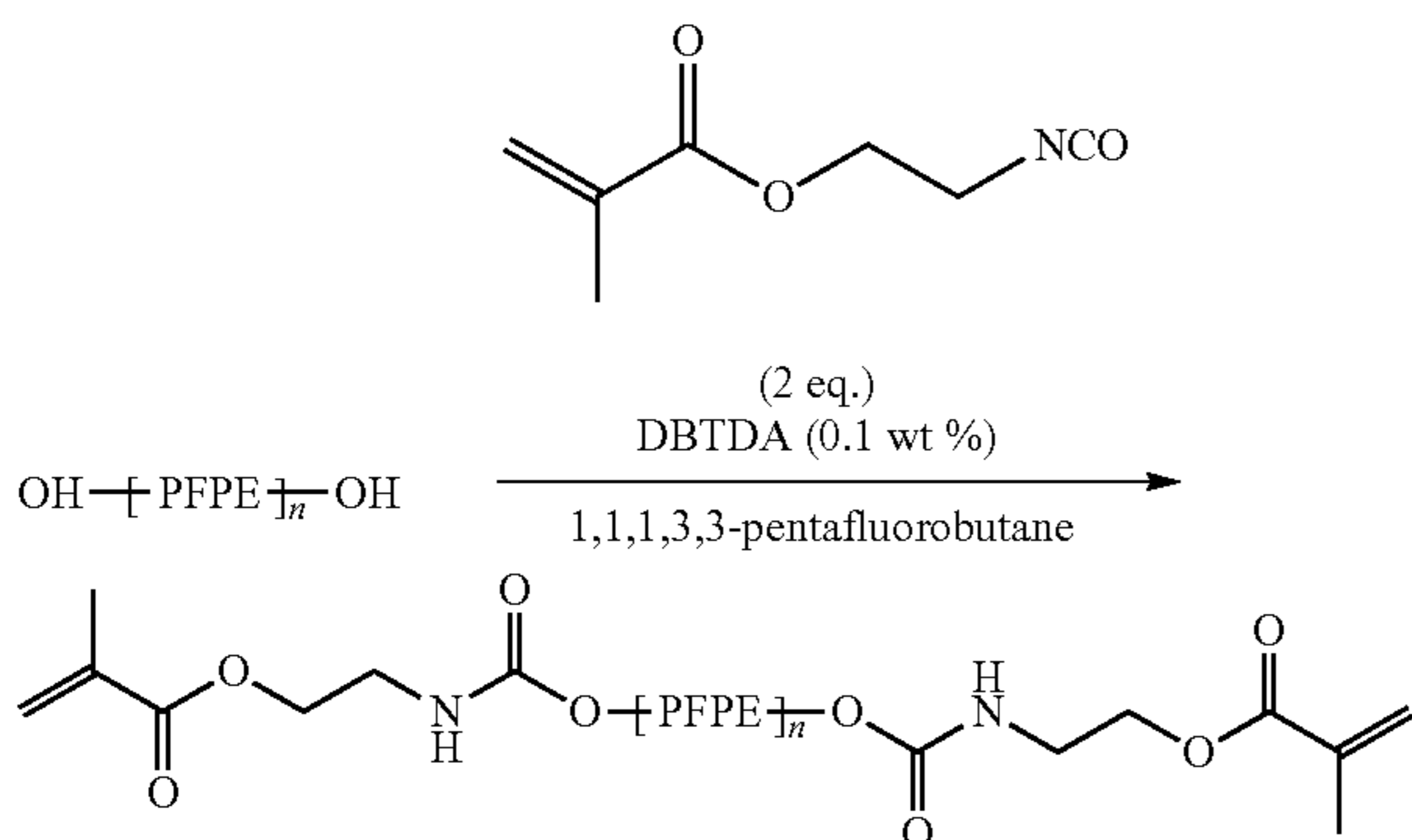
Scheme 2. Synthesis of 4 kg/mol dimethylacrylate-functionalized perfluoropolyether (PFPE-DMA) monomer.
