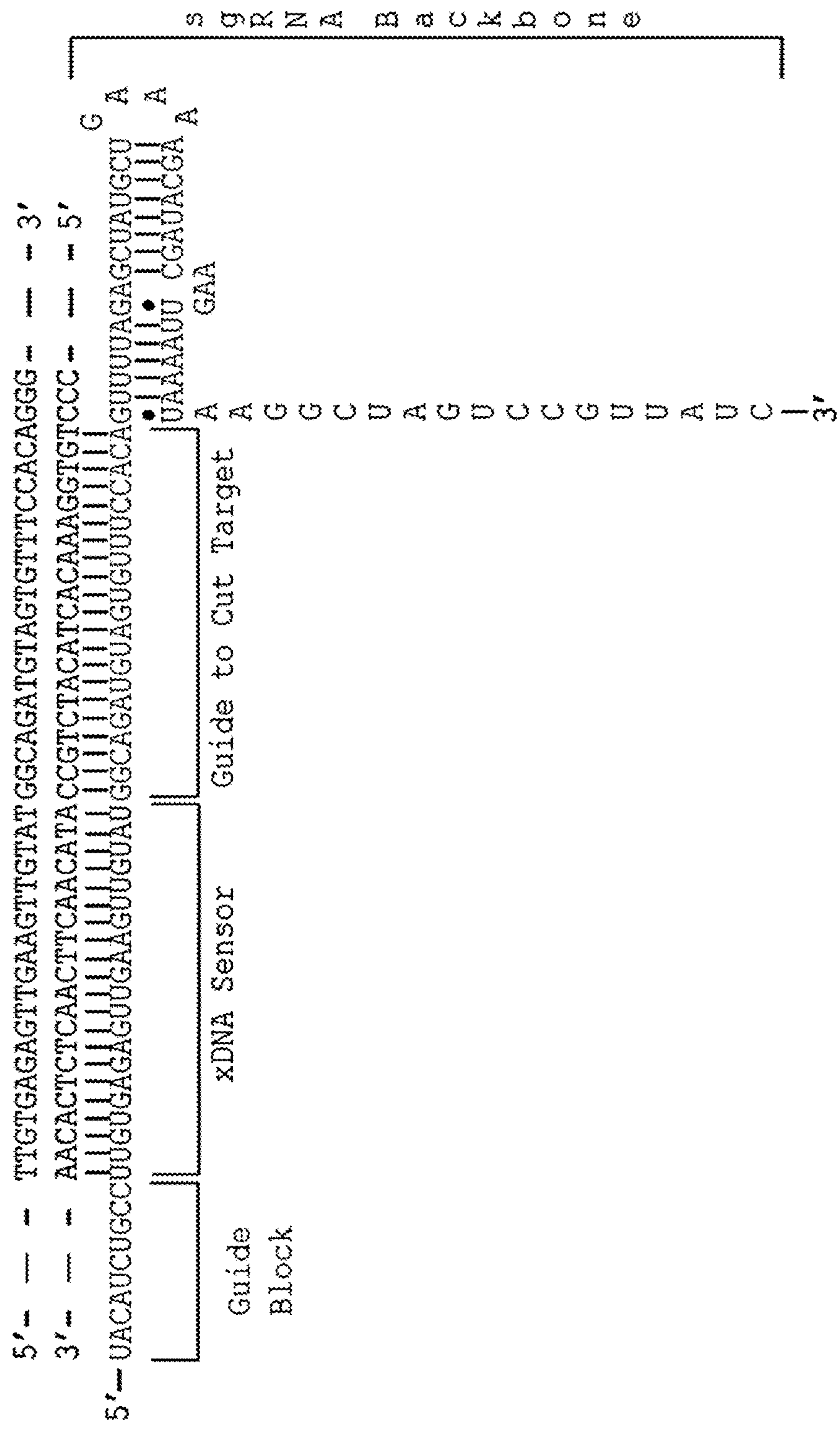
gRNA 5' xDNA sensing, On State
