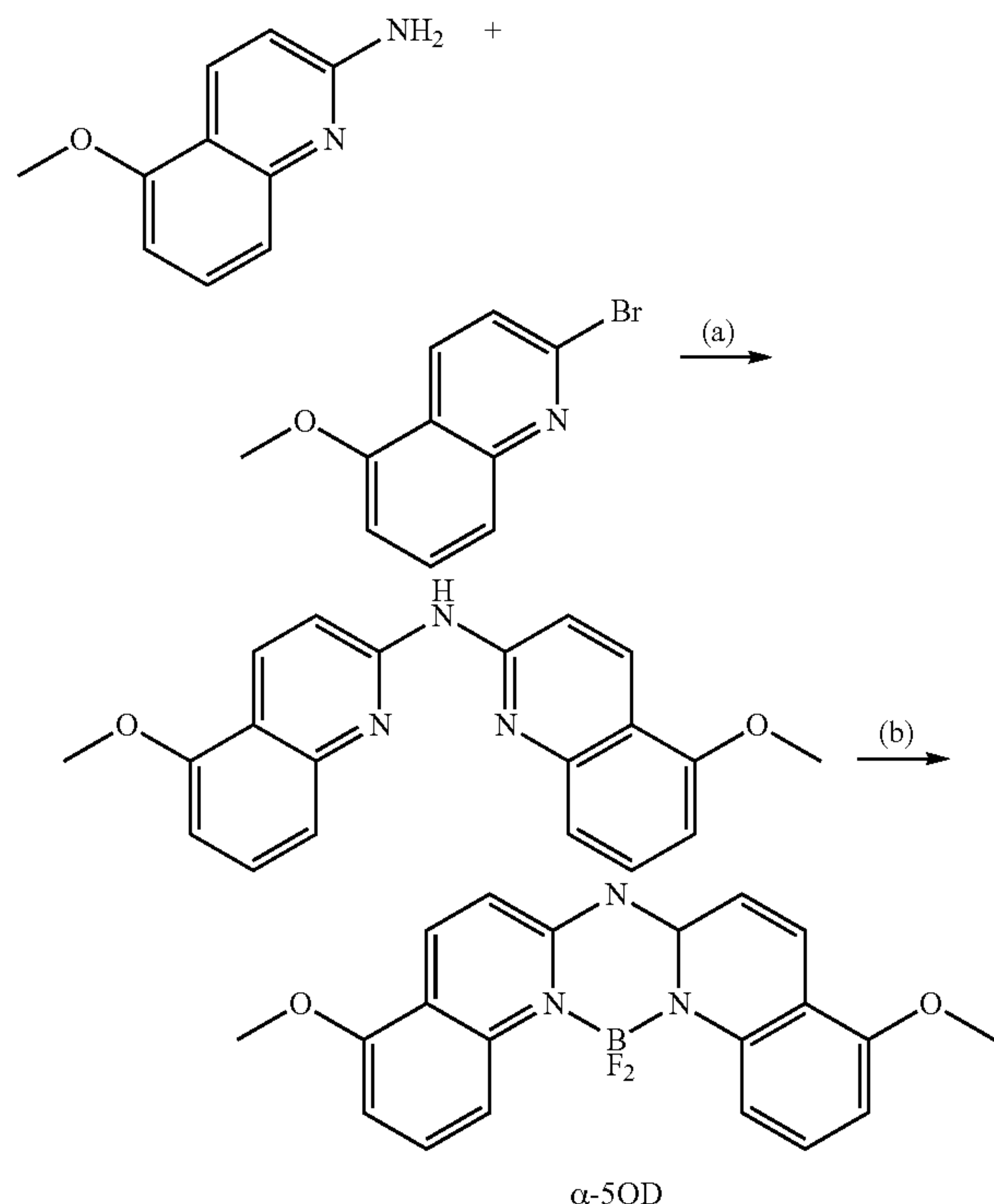
Synthetic scheme to make substituted α-5OD compound.
