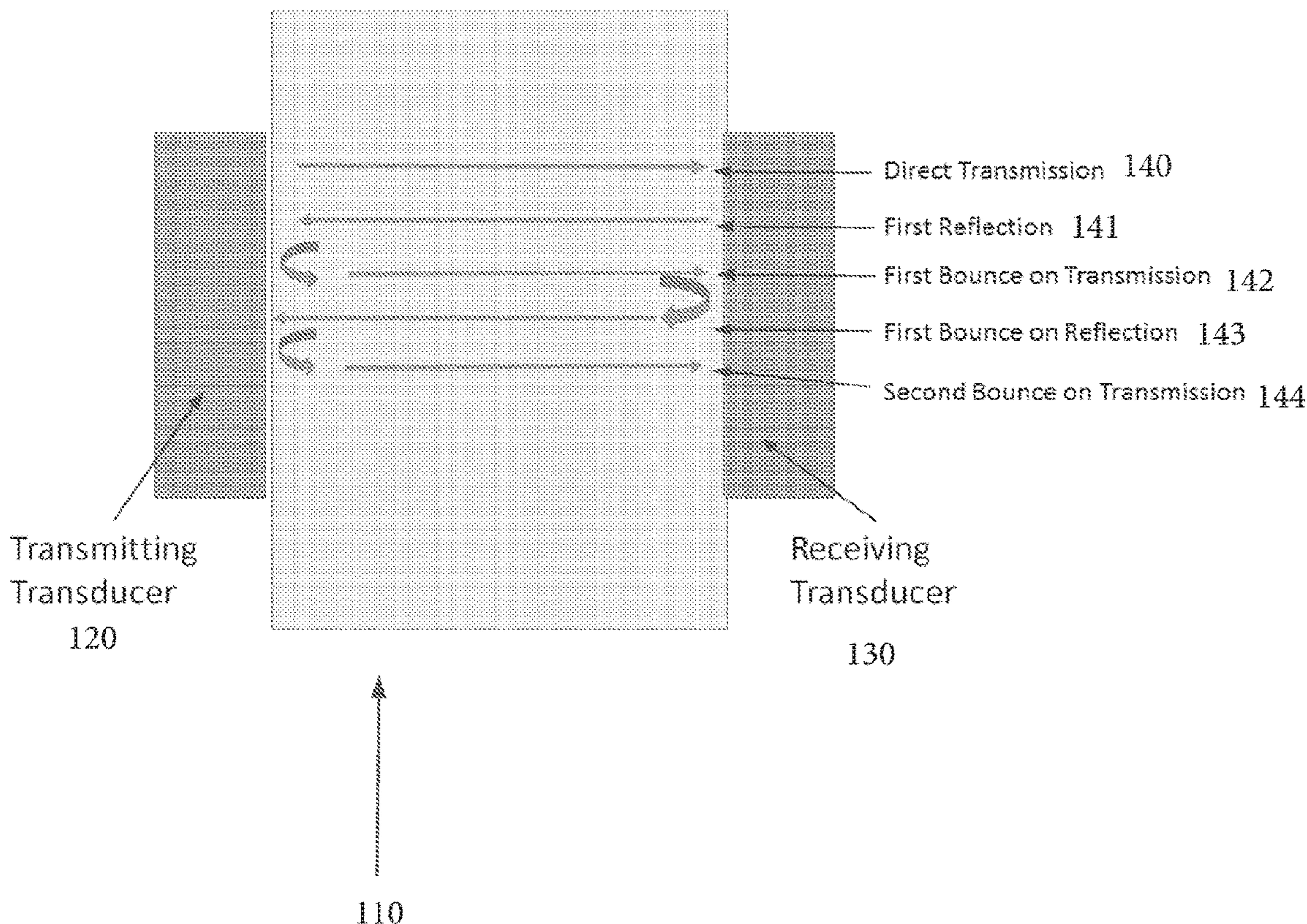
Ultrasound Pulse/Echo with Bounces
