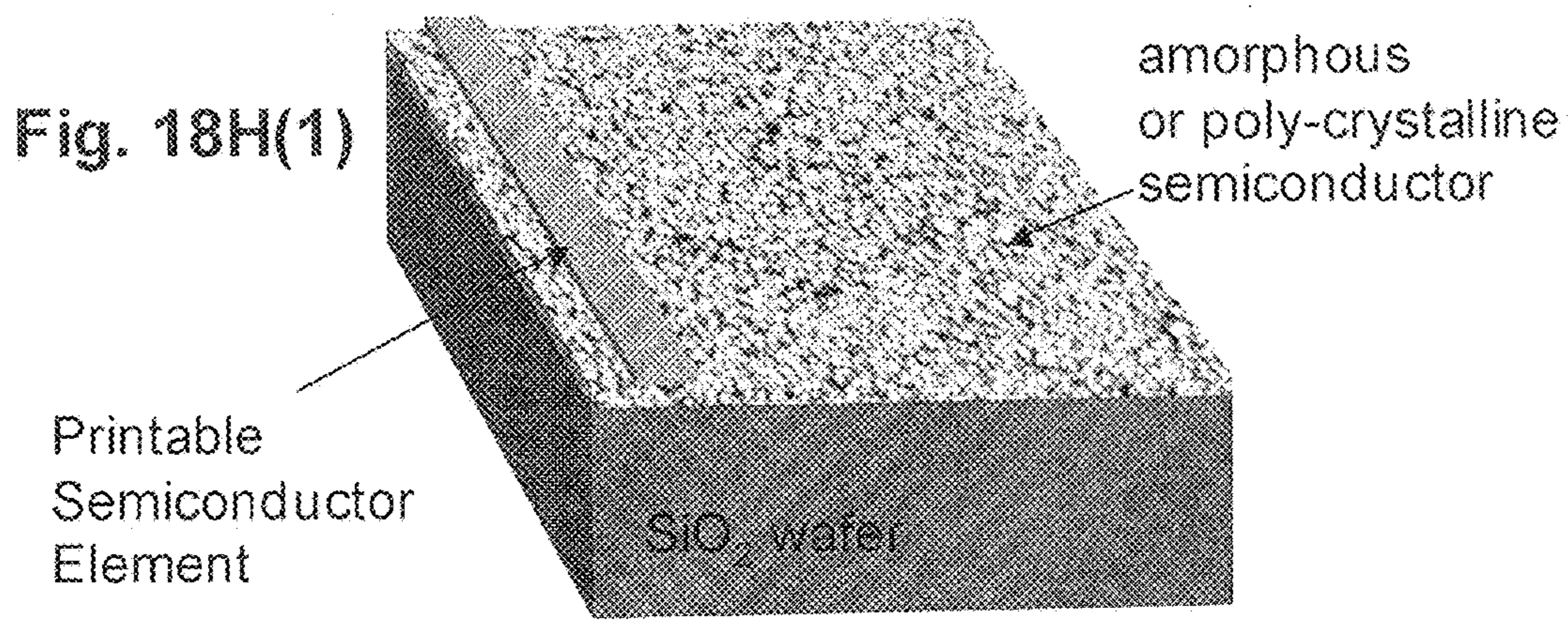
Transfer of a Printable Semiconductor Element (seed)
