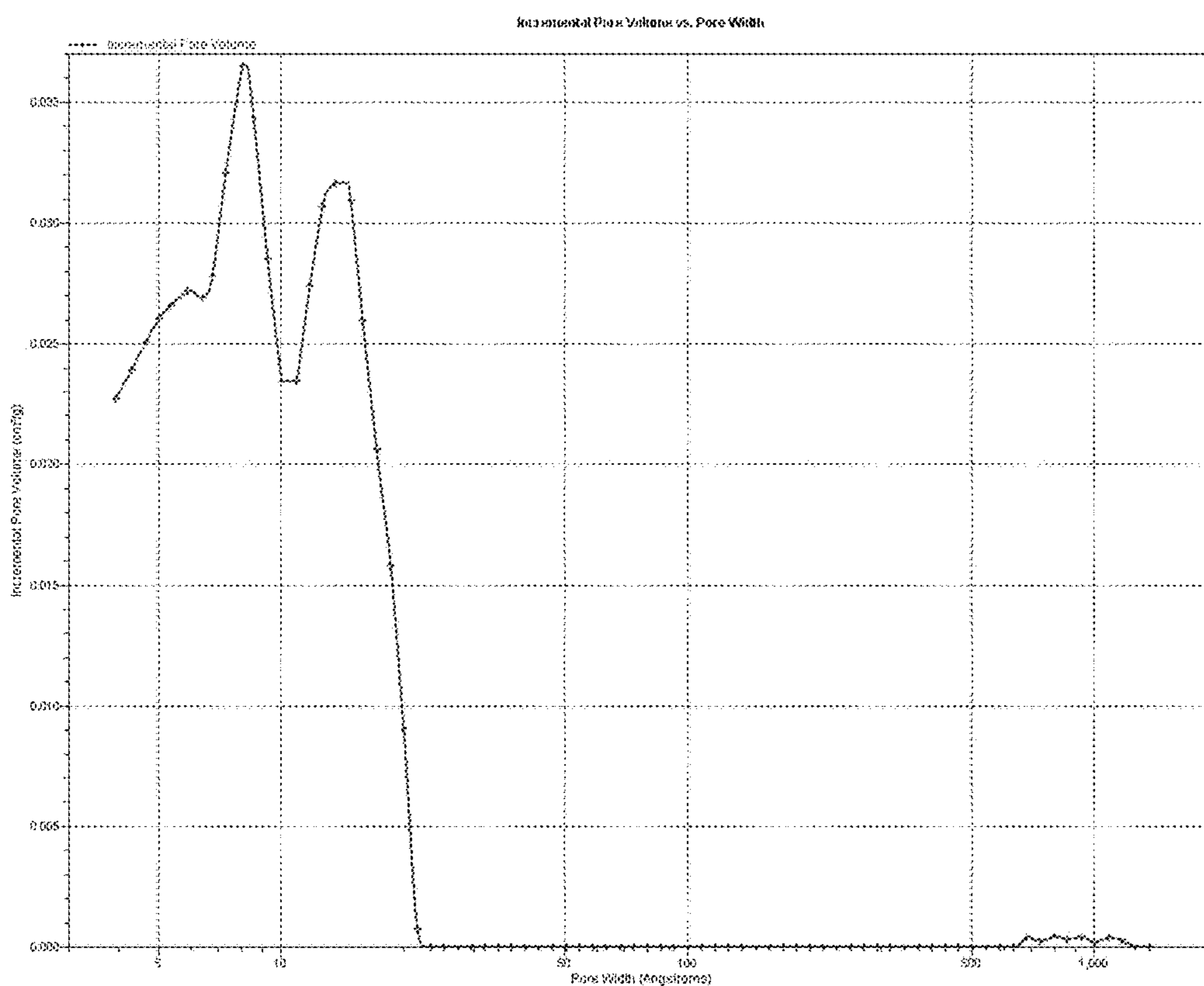
Figure 2. Pore distribution for carbon of Example 8.
