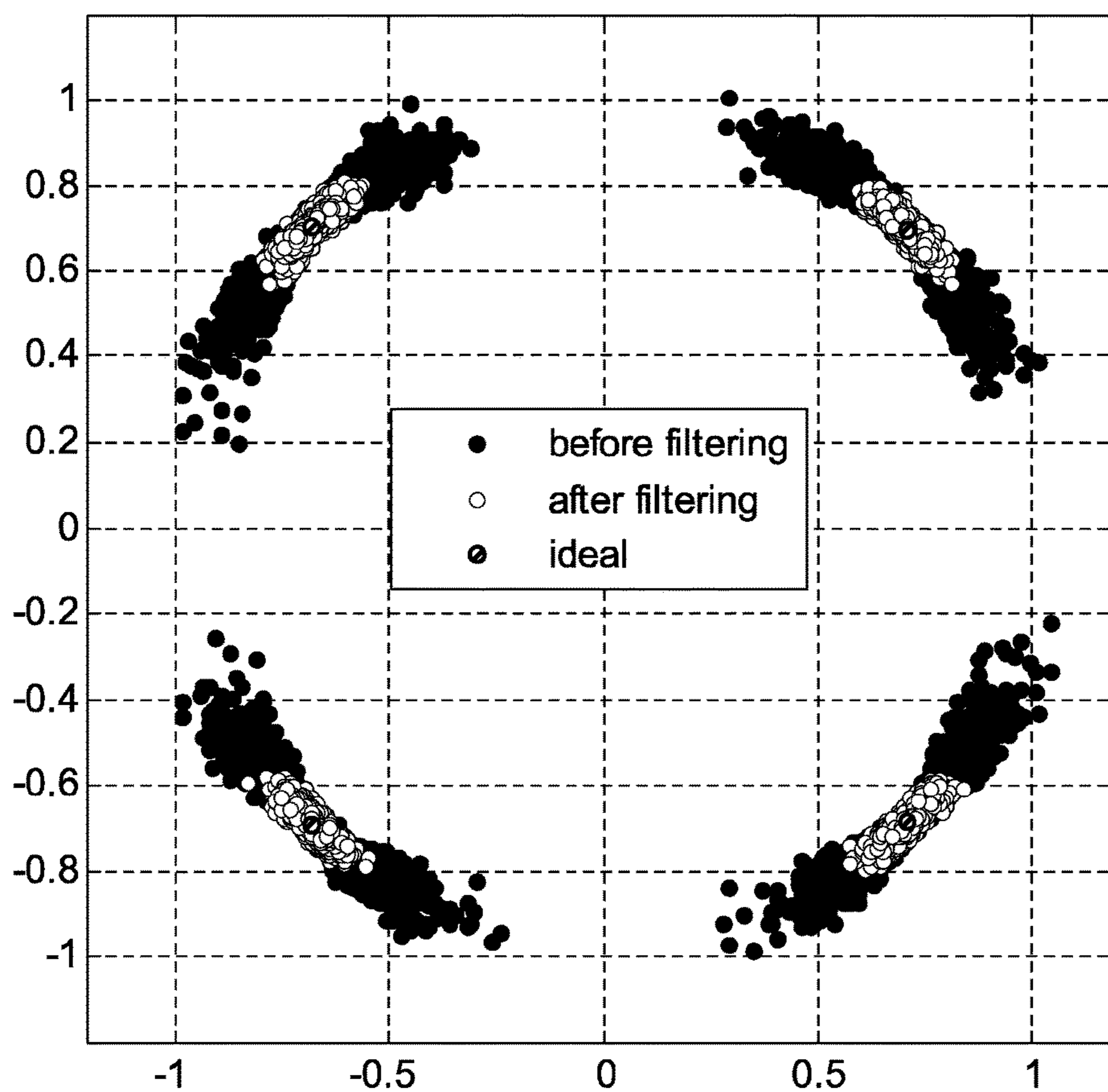
Constellation after 10-Span Transmission and Removal of Tx Filtering Effects
