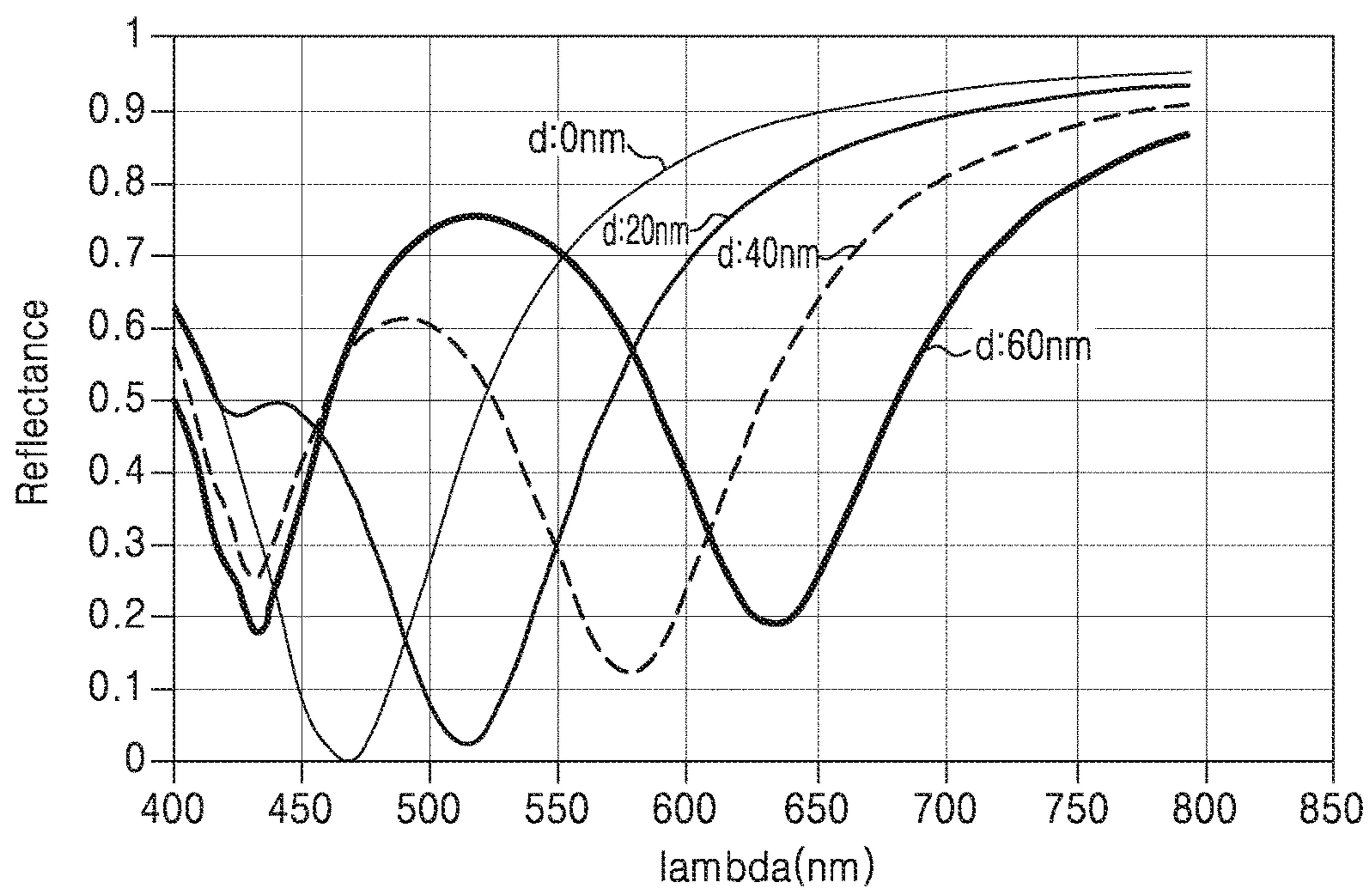
Reflectance curve
