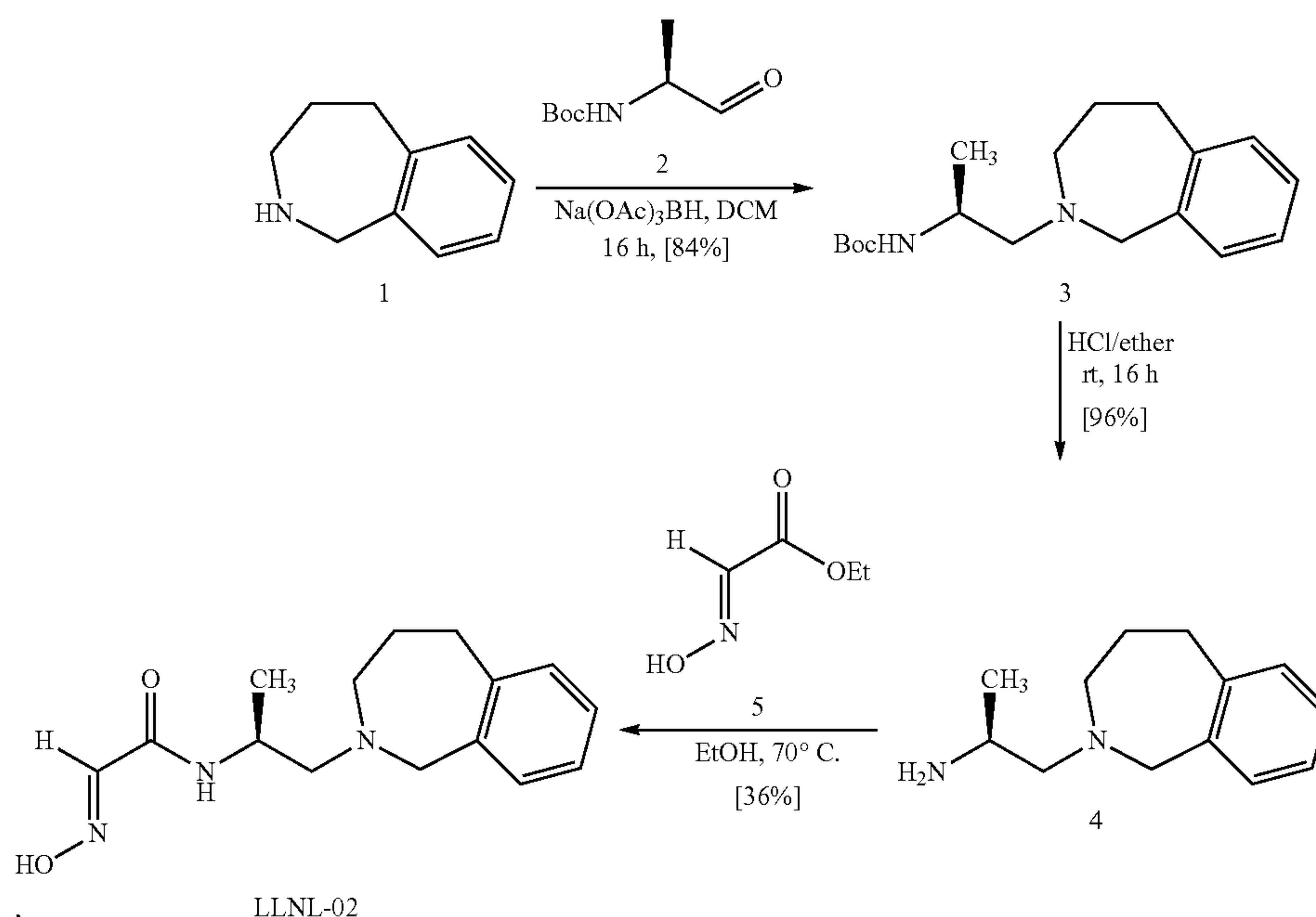
Scheme 2. Synthesis of LLNL-02 (CV11-061-A, or CV1161A)
