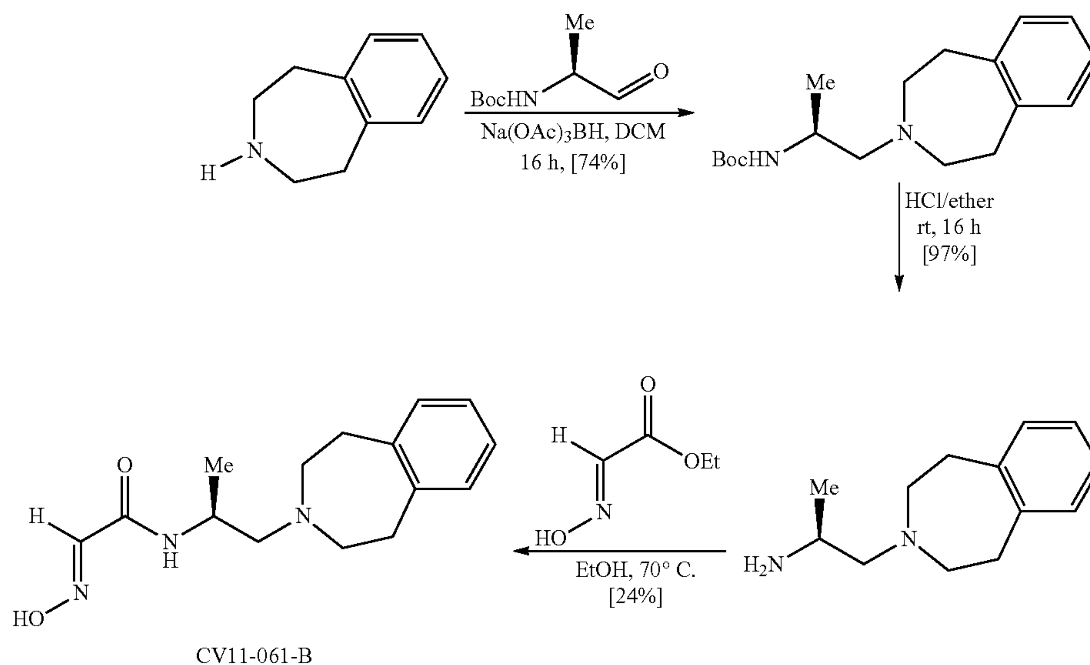
Scheme 3. Synthesis of CV11-061-B
