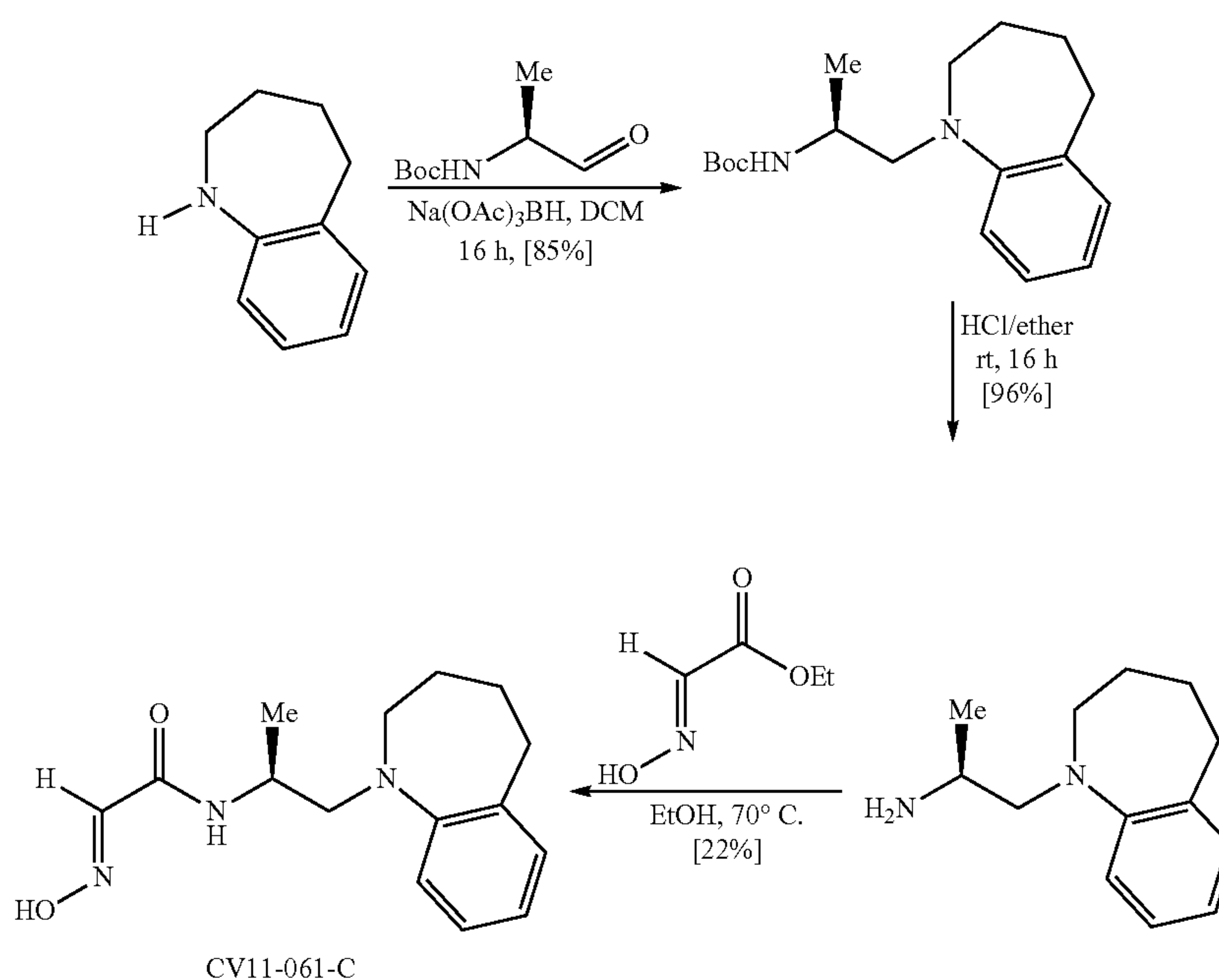
Scheme 4. Synthesis of CV11-061-C
