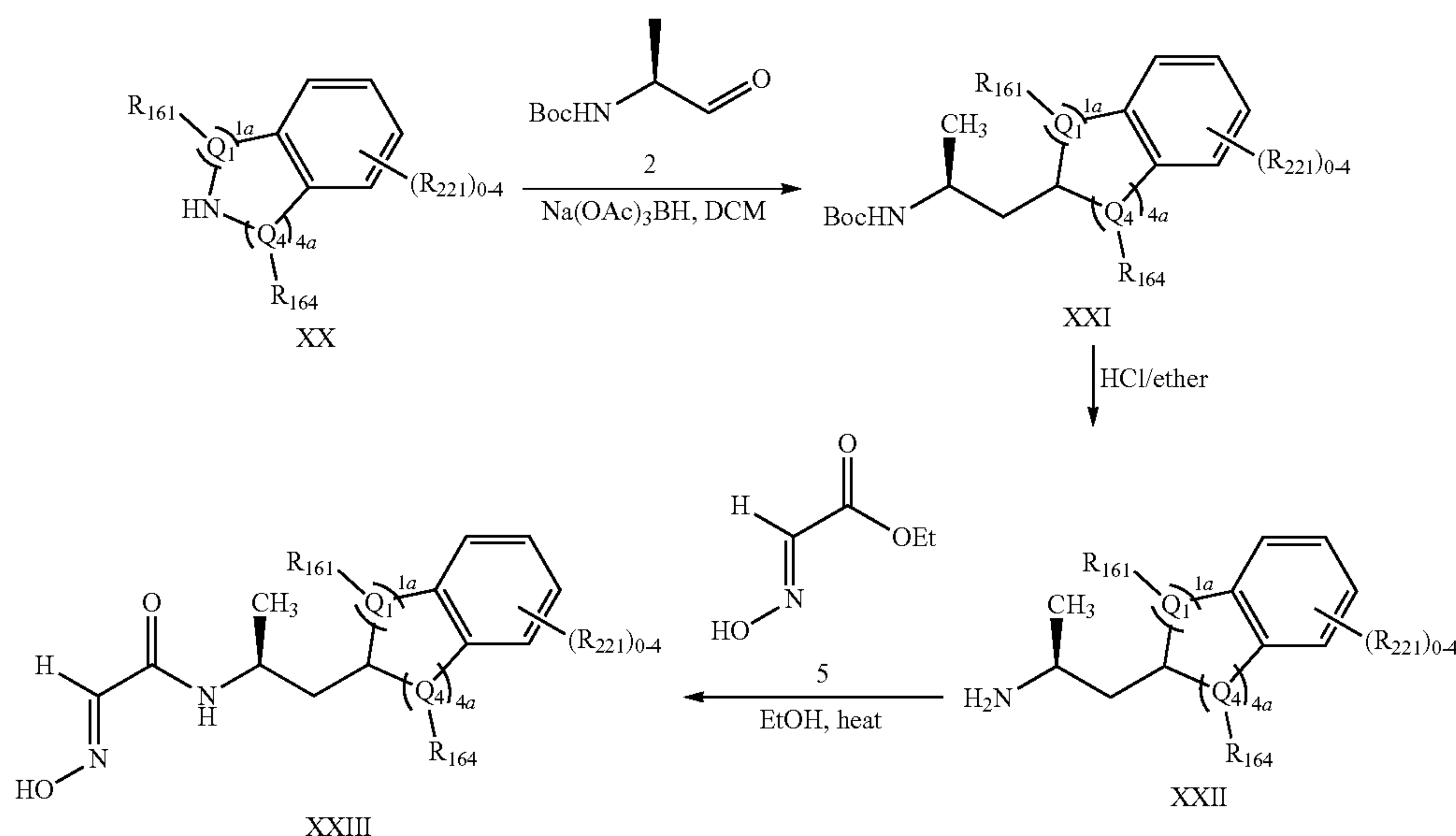
Scheme 1. General route for the construction of the benzoazepine class of compounds
