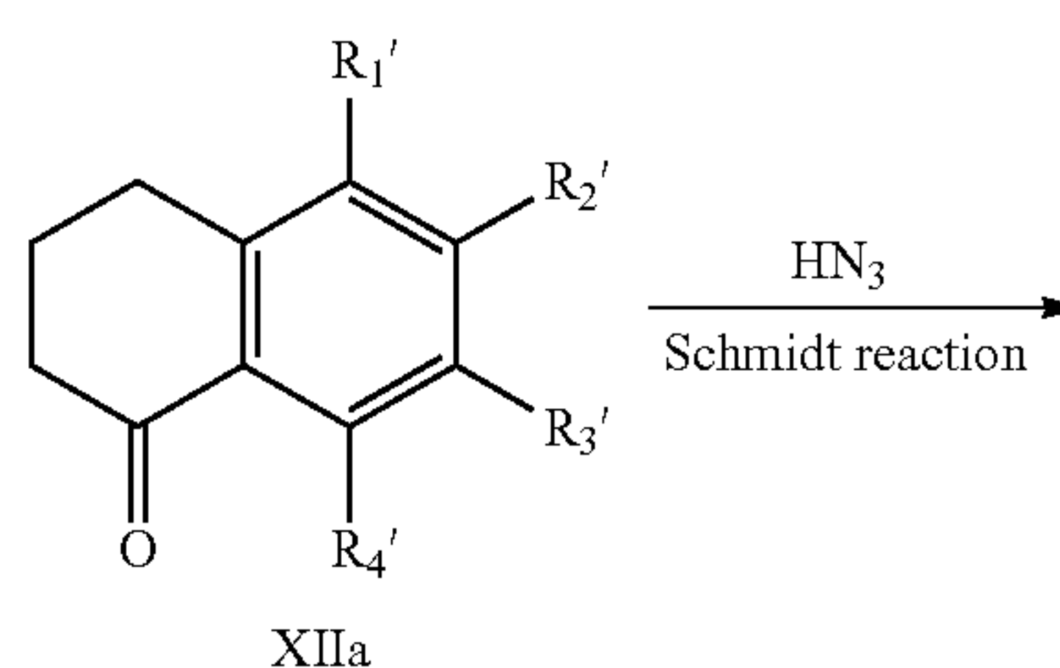
Scheme 5. Route to phenyl-ring modified analogs of LLNL-02 starting with commercially available, inexpensive and differentially substituted tetralone building blocks
