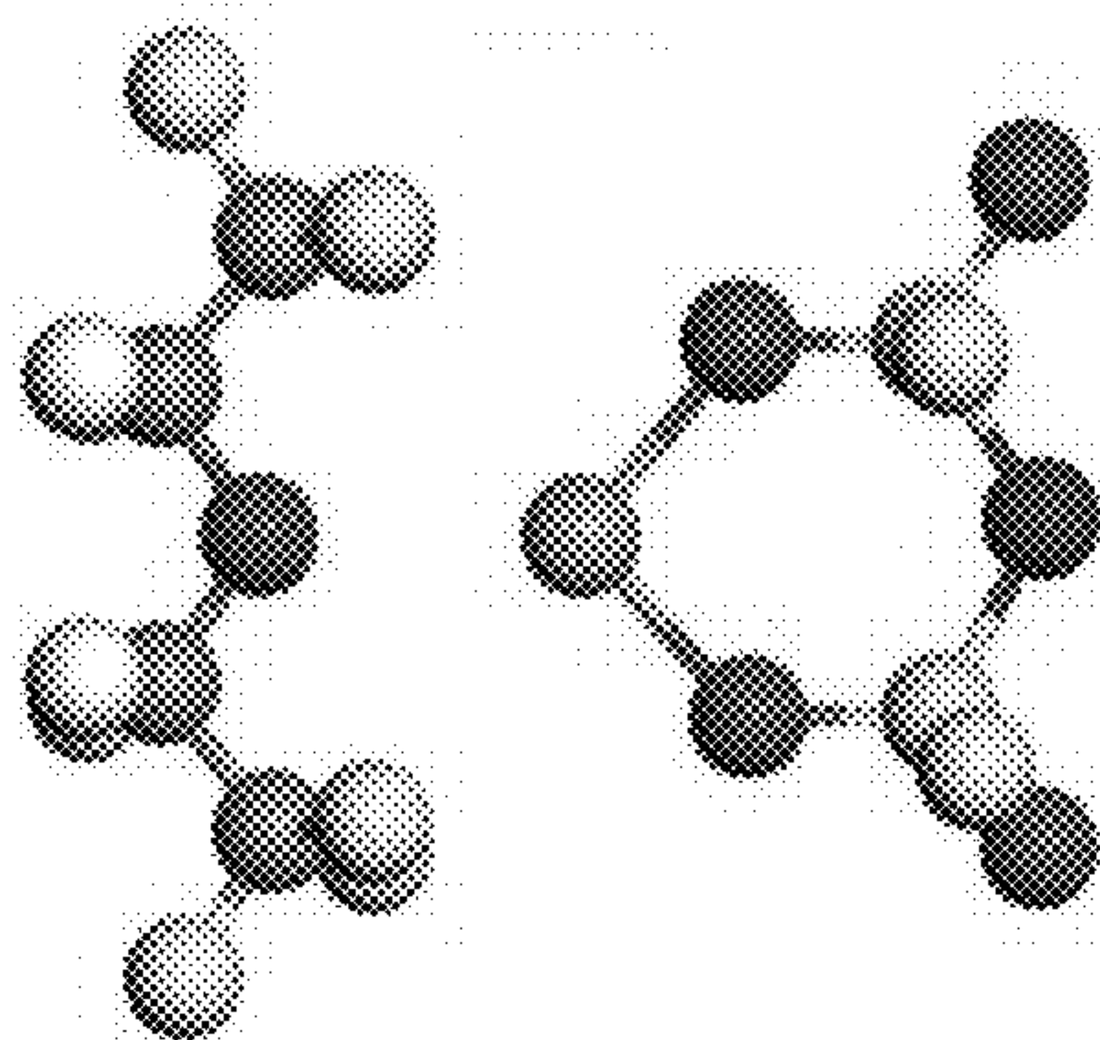
BTFE+LiFSI
