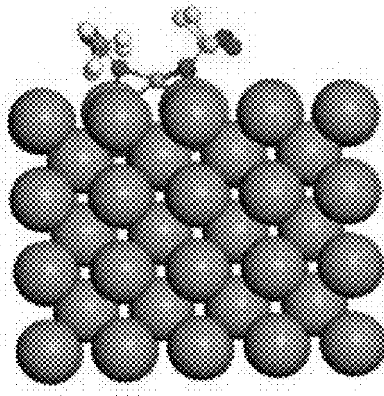
DMC-LiFSI
