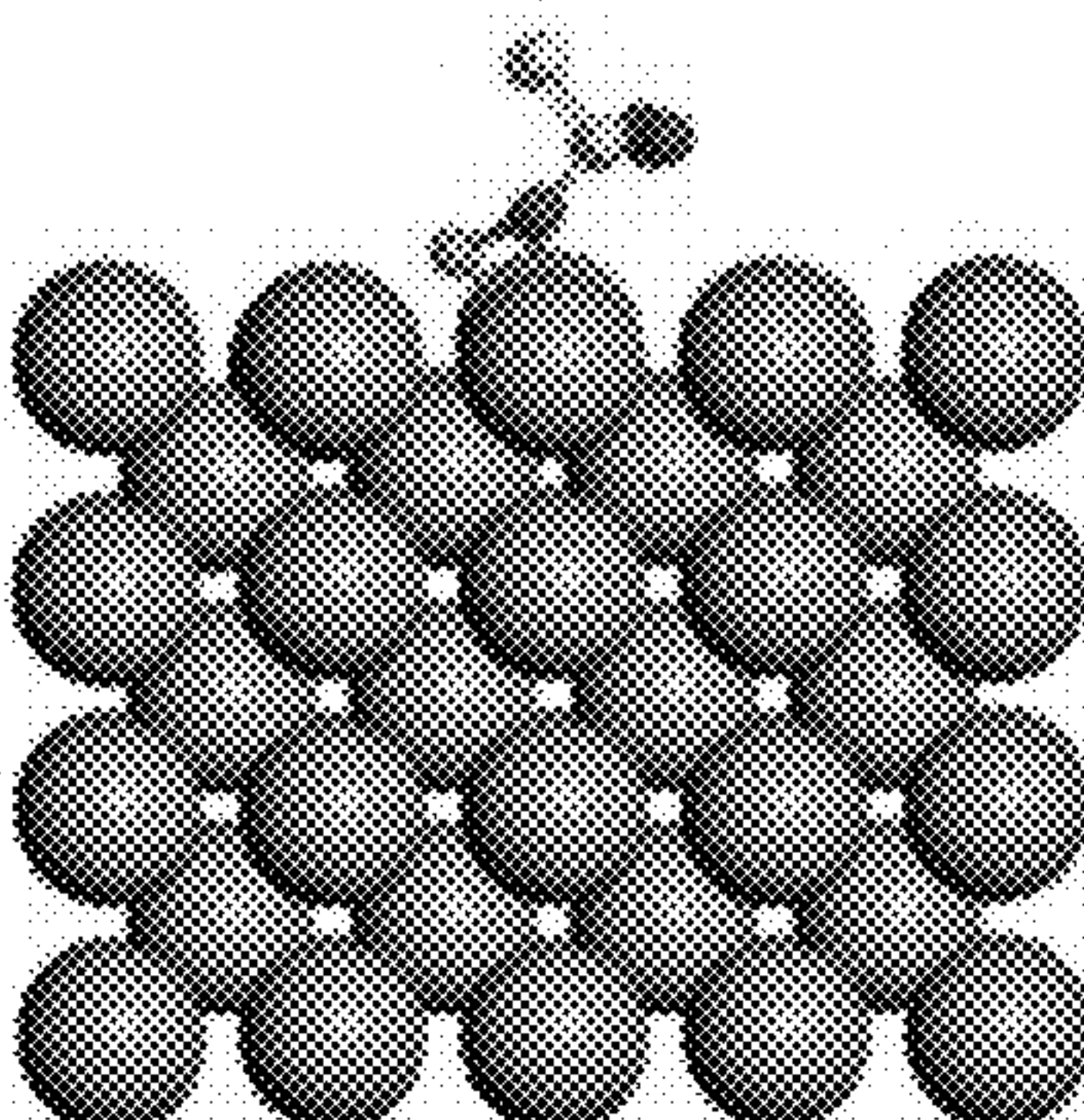
LiFSI
