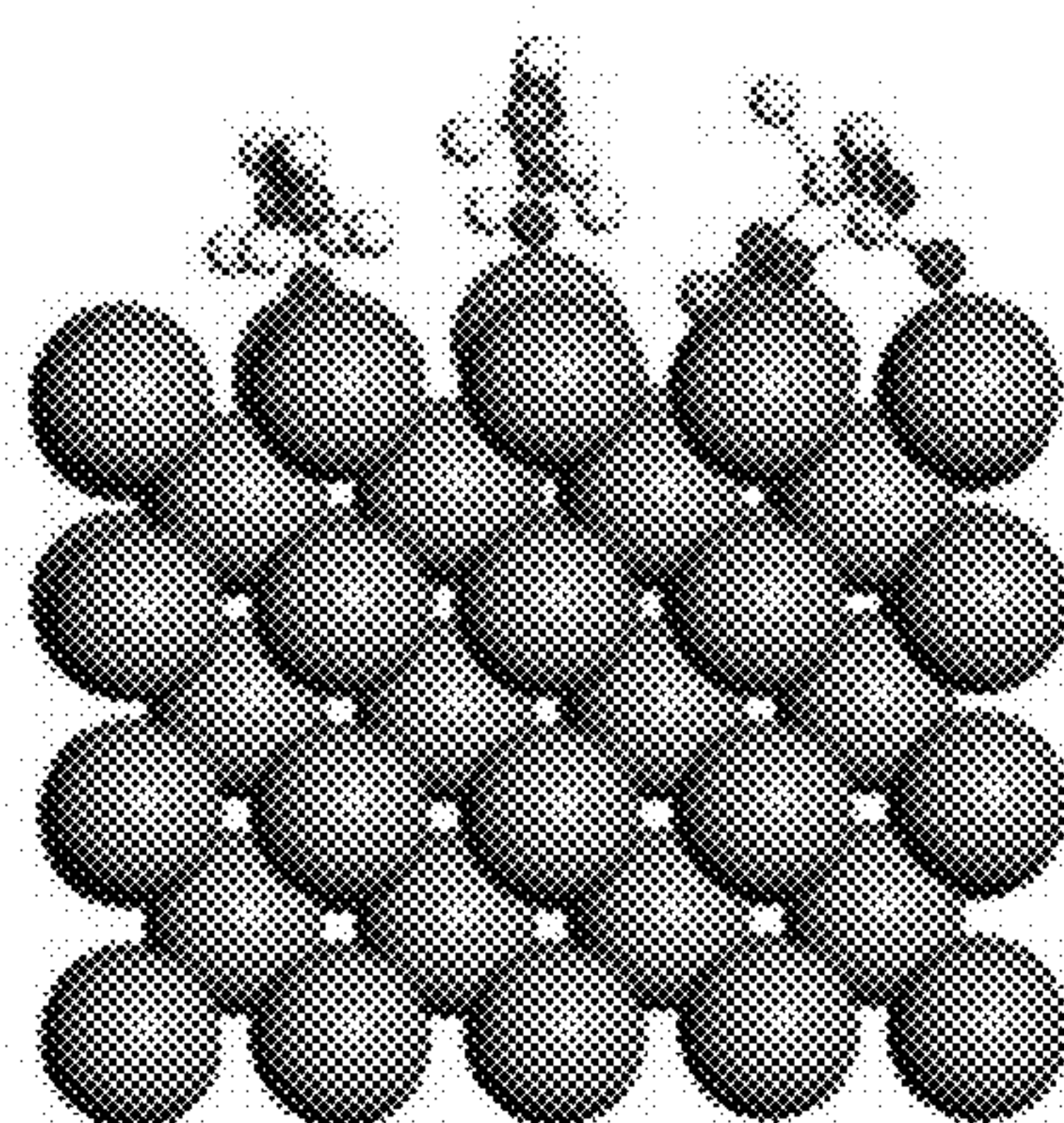
2DMC/LiFSI
