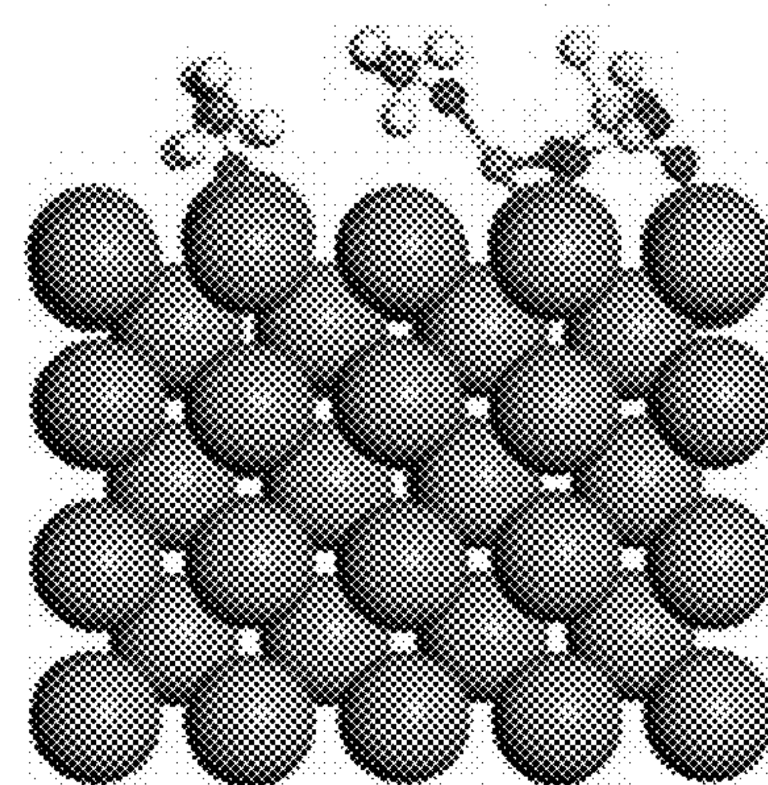
DMC/DMC-LiFSI
