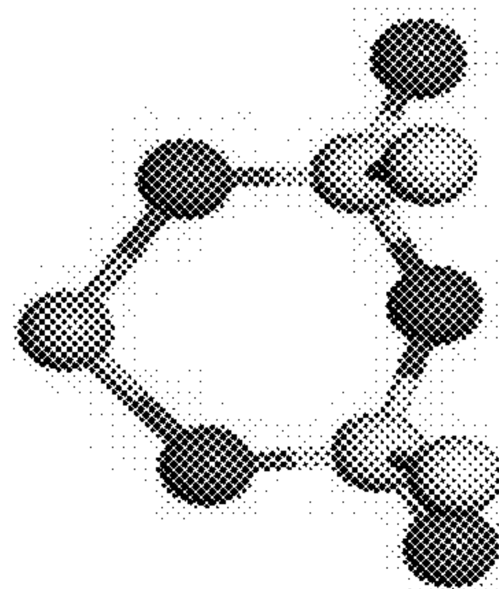
LiFSI
