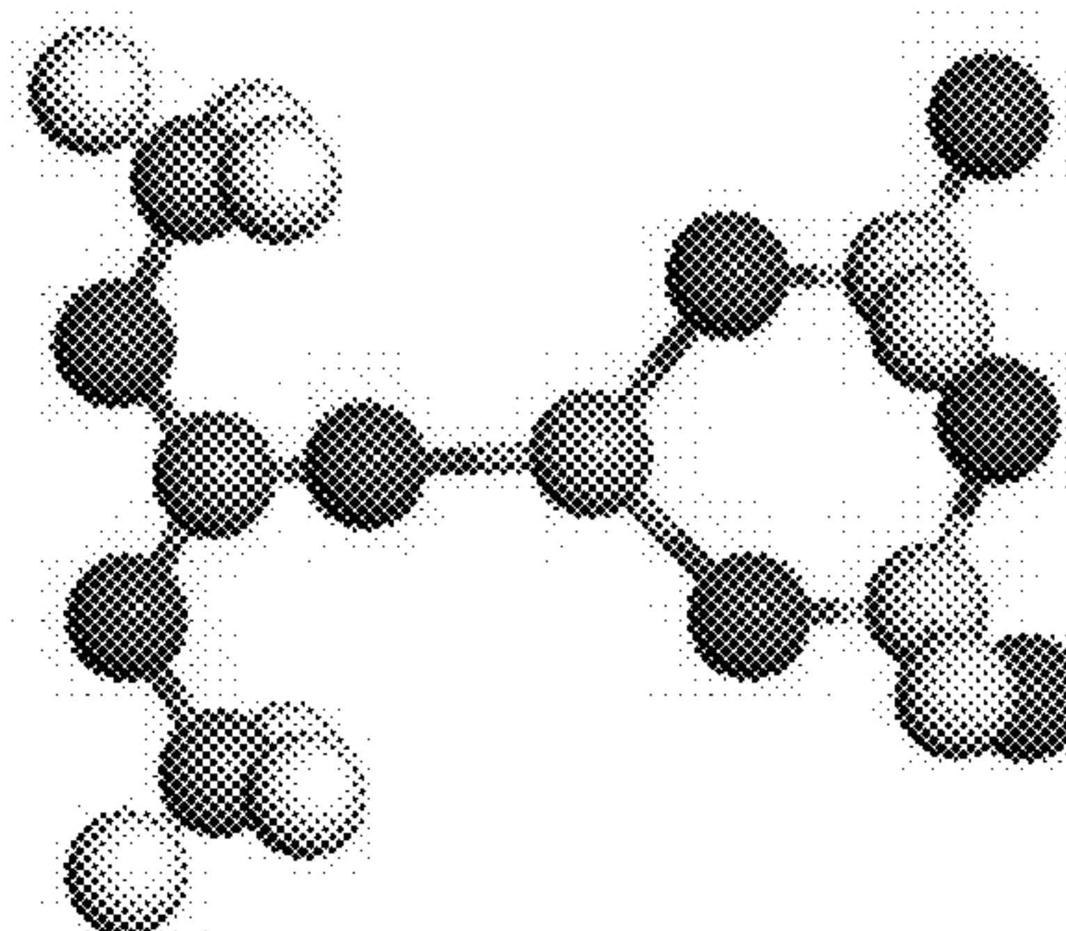
DMC+LiFSI
