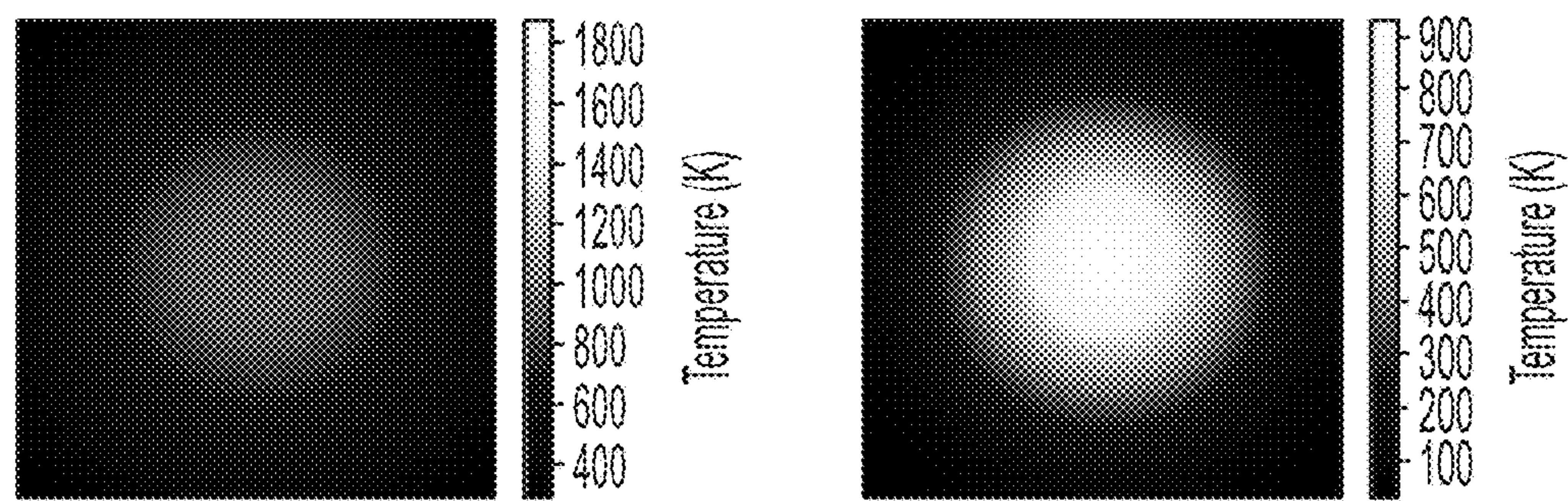
FIG. 4C Measured Temperature without TE Separation FIG. 4D Error in Measurement
