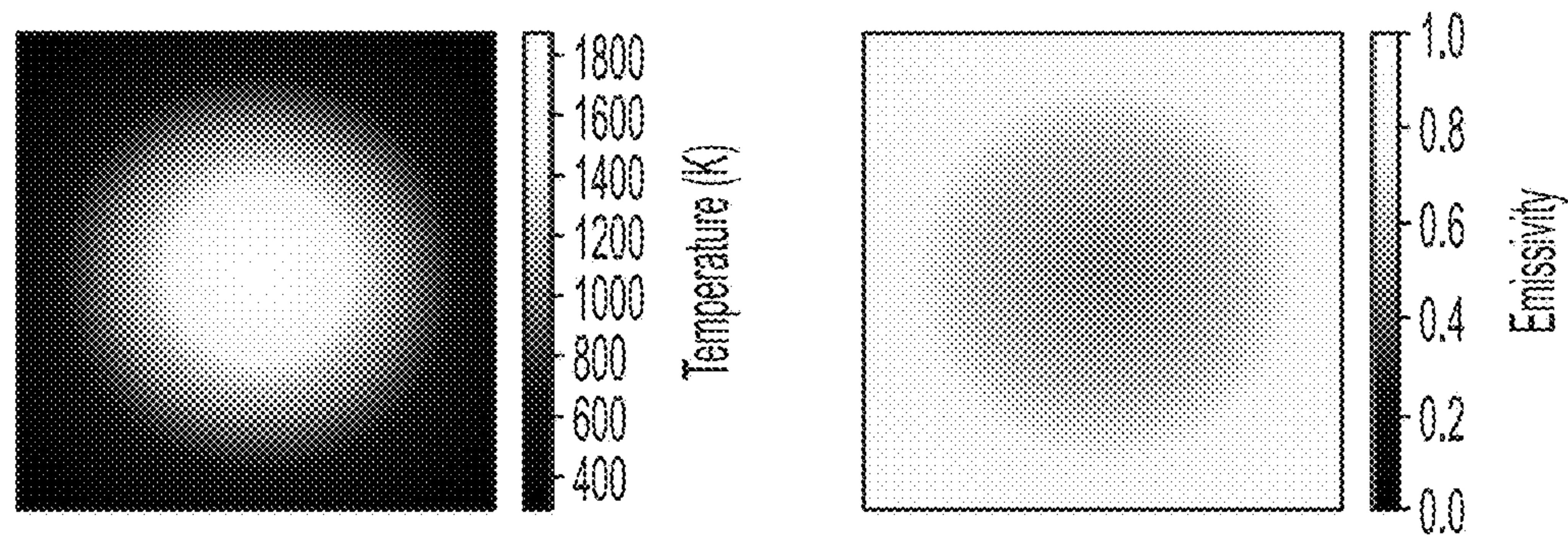
FIG. 4A Melt Pool Temperature FIG. 4B Typical Emissivity Distribution
