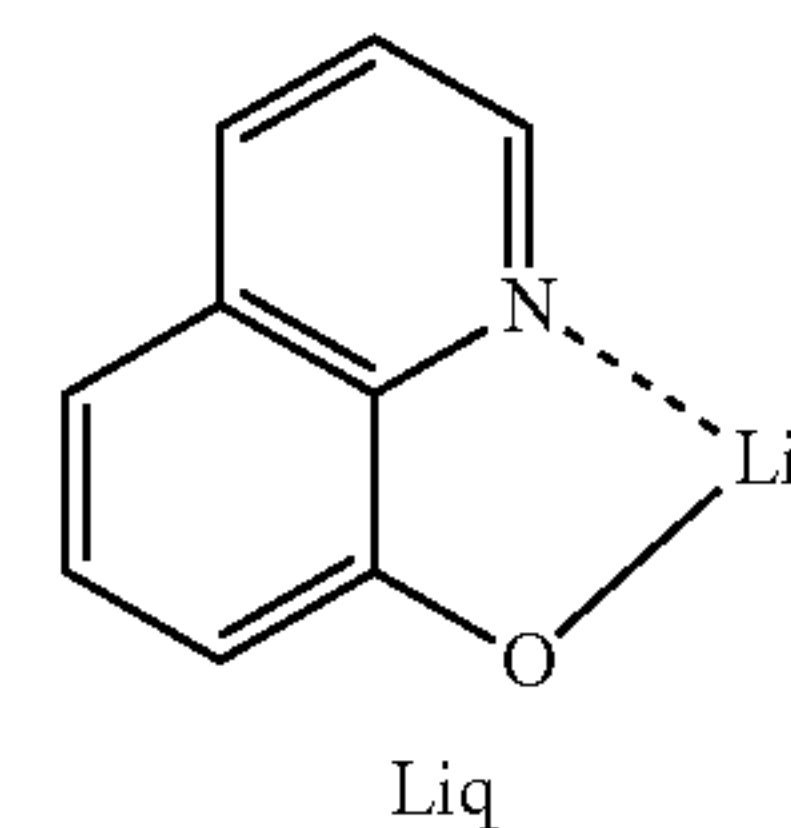
aDBT-ADN
