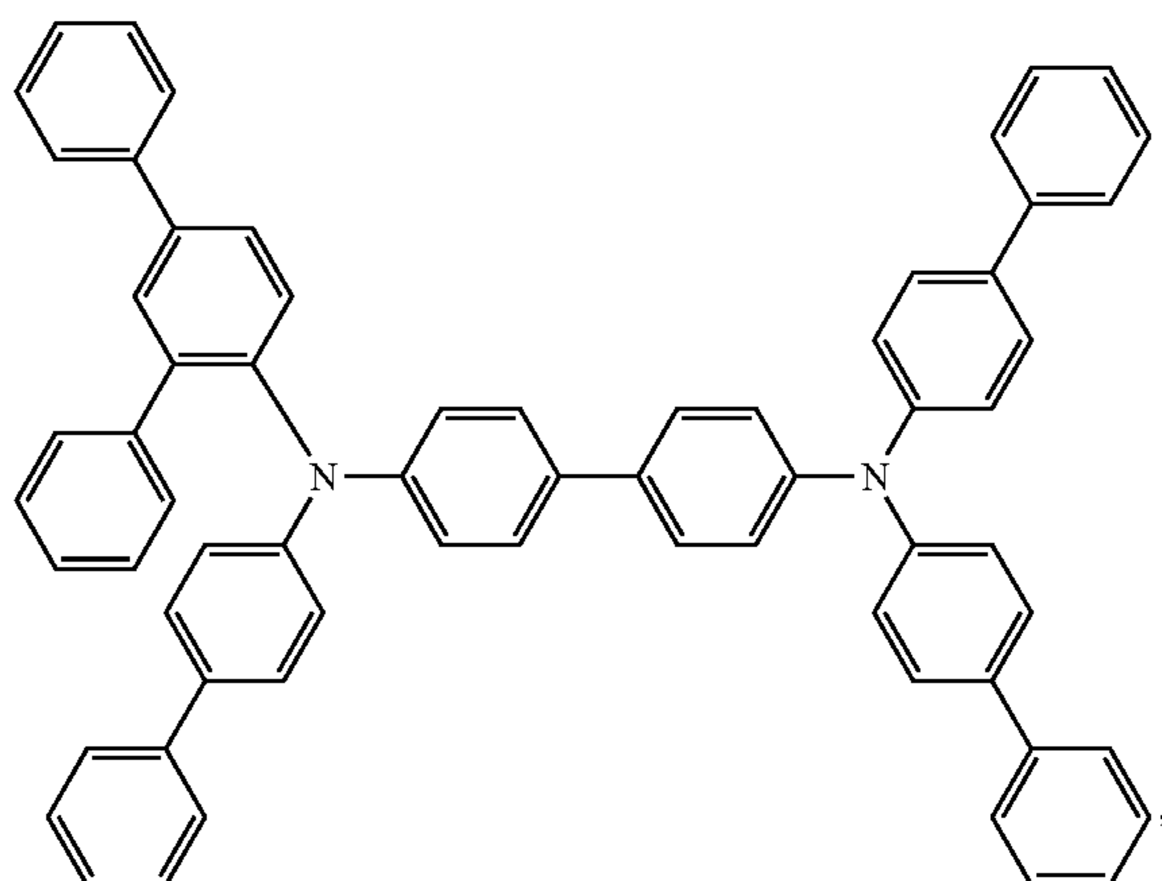
PPh-TPD
