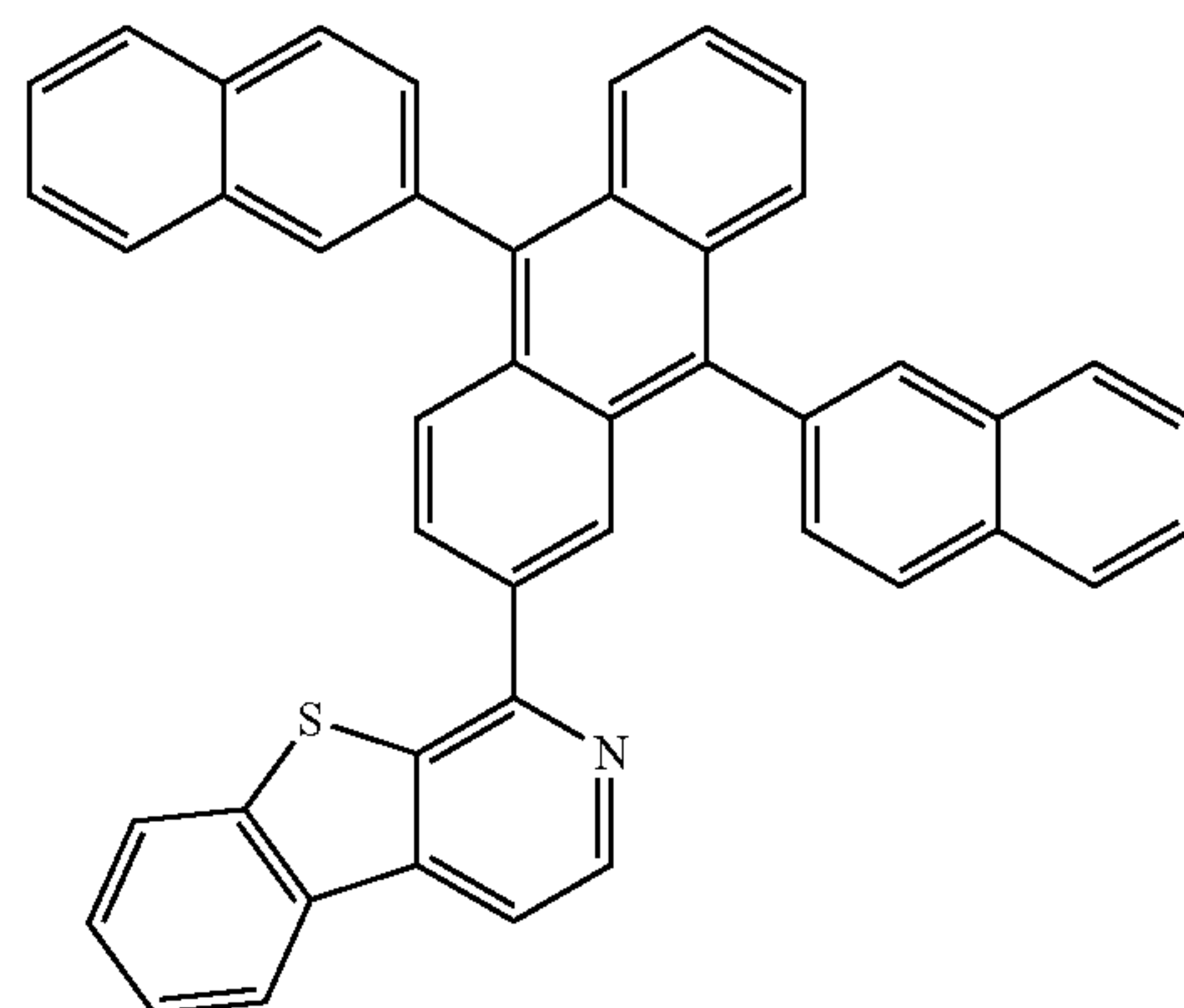
aDBT-ADN
