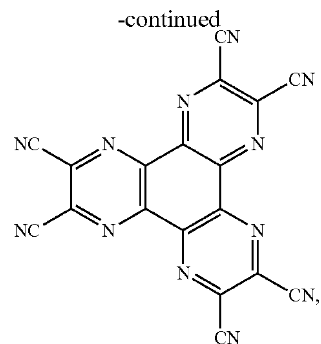
HATCN
