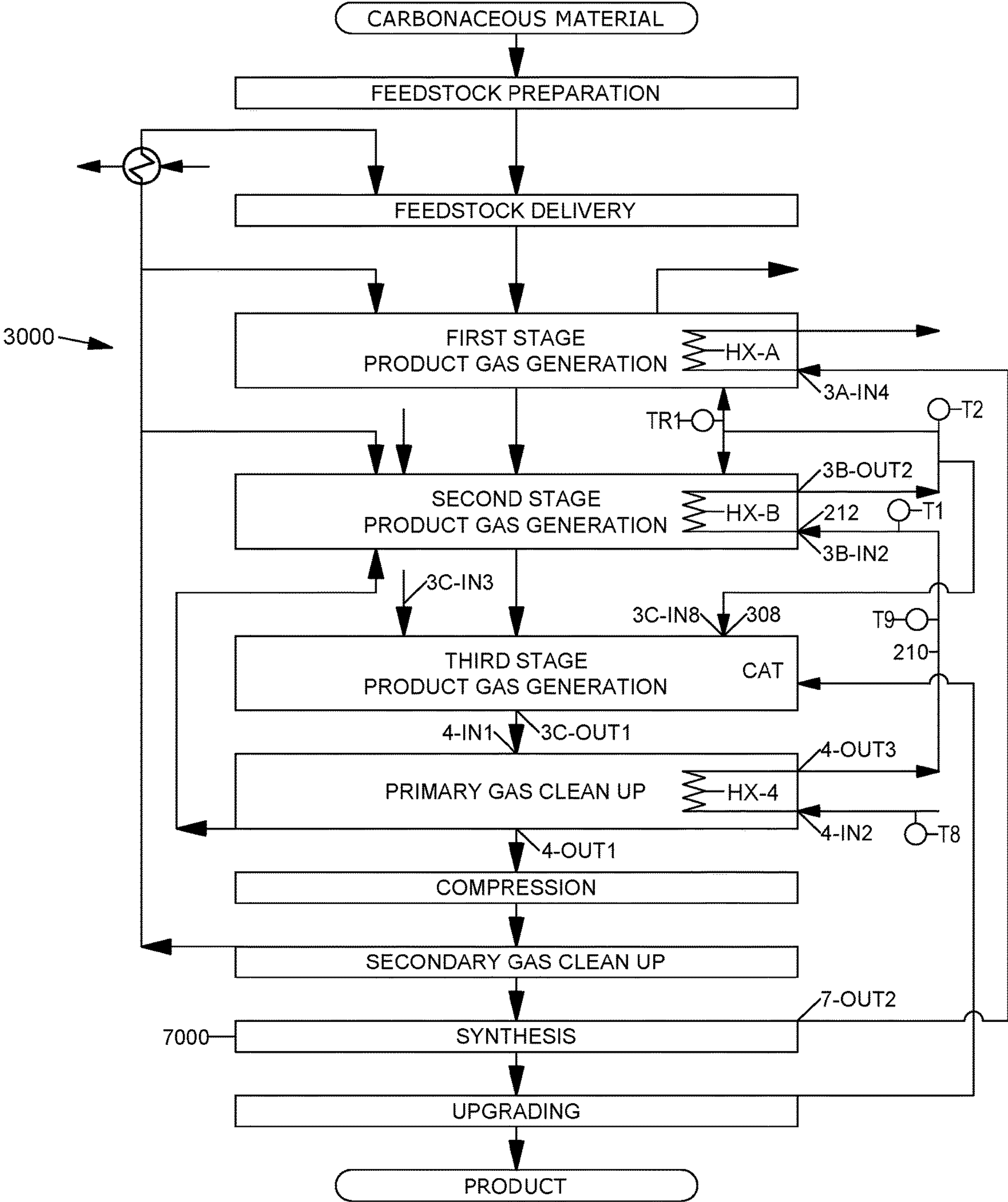
FIGURE 26 REFINERY SUPERSTRUCTURE (RSS)
