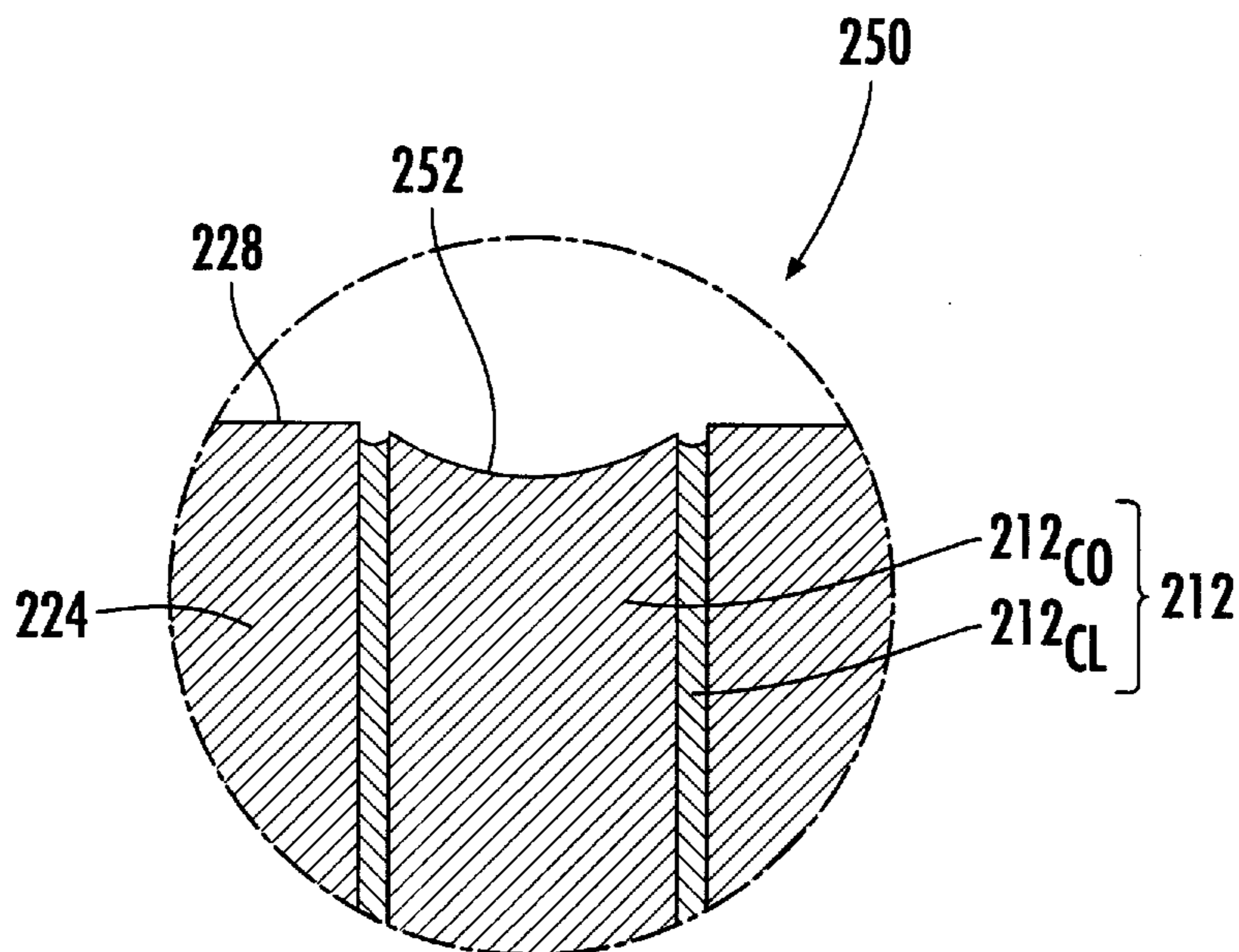
FIG. 21 (PRIOR ART)
