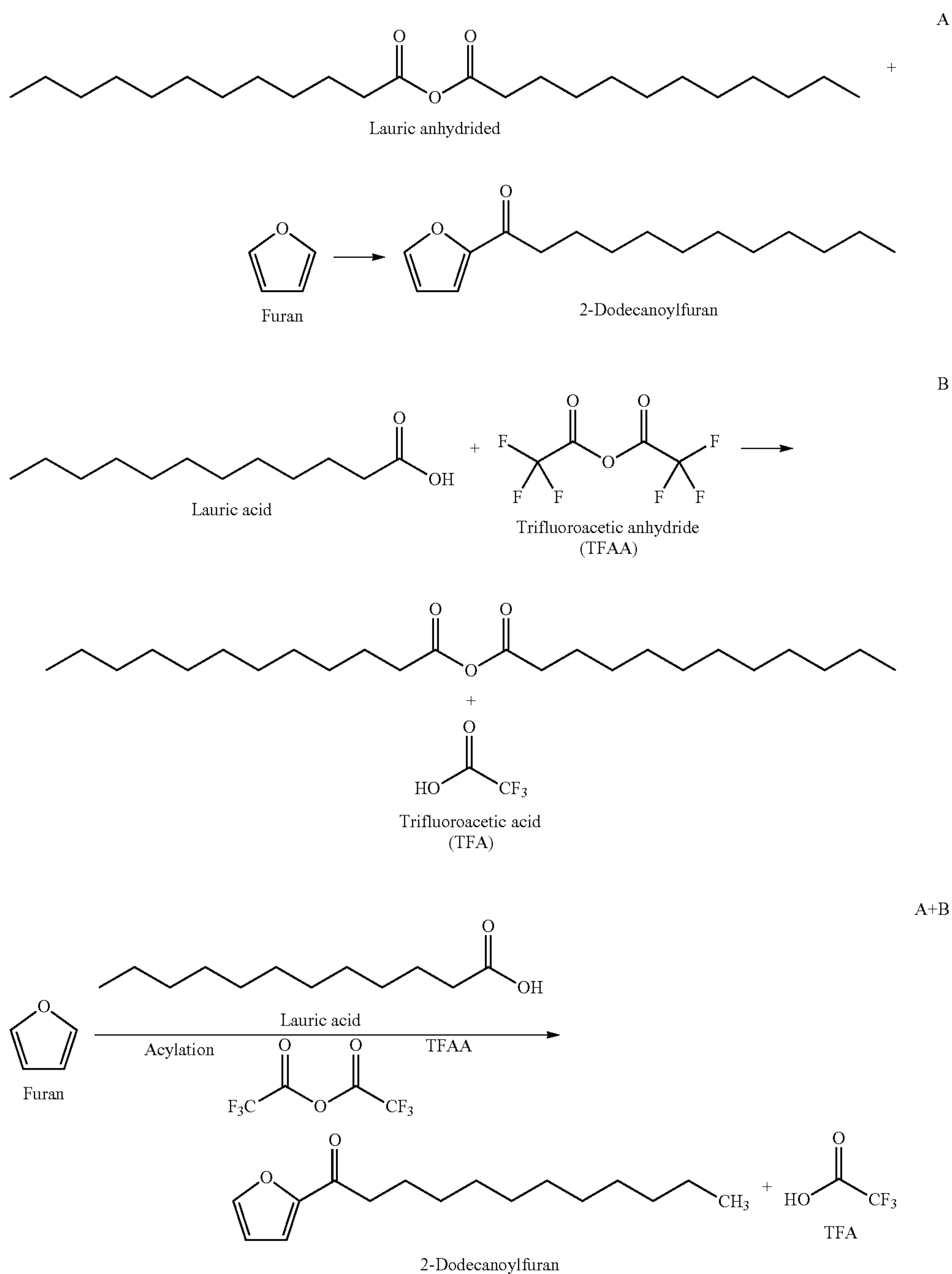
Scheme 1. Tandem anhydride and acylation of fatty acid over trifluoroacetic anhydride.
