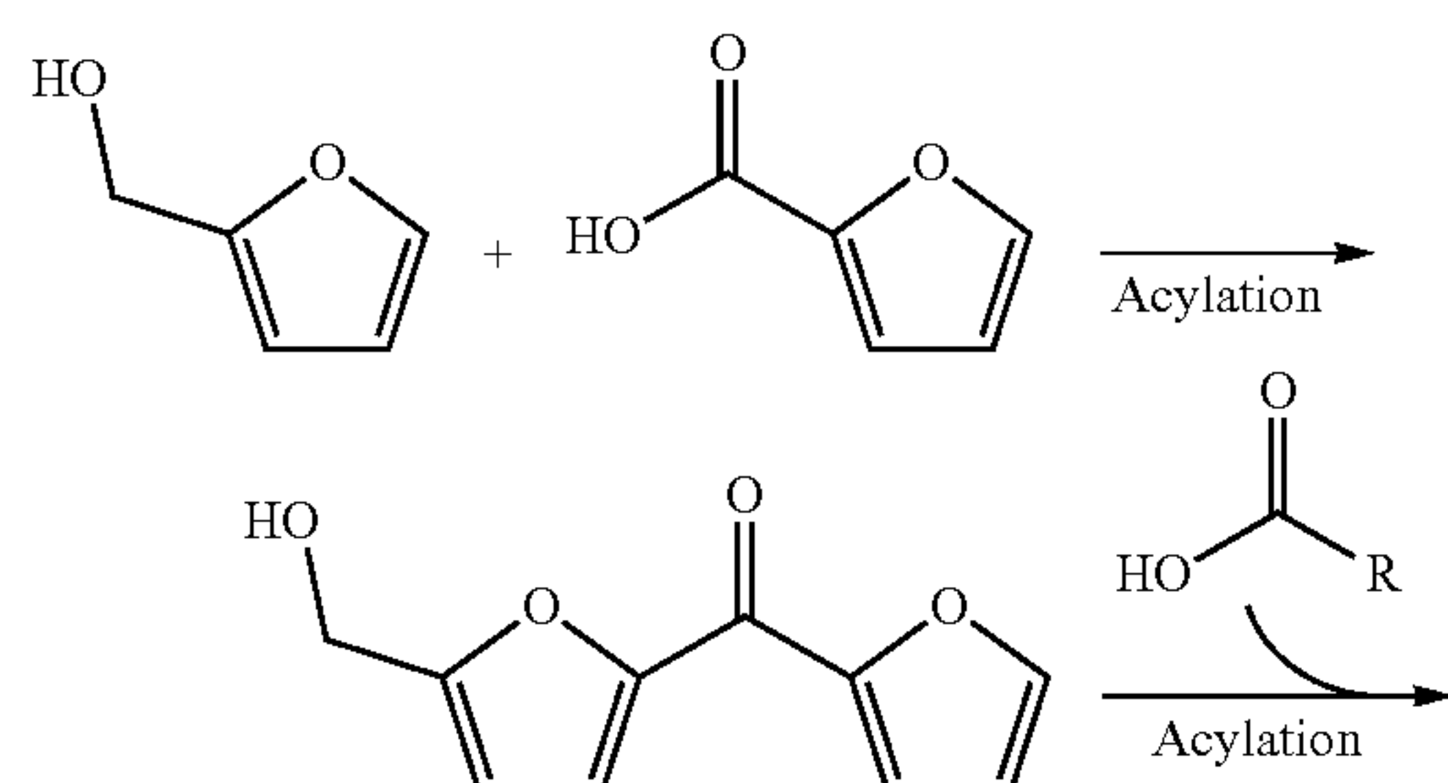
Scheme 4. An additional option for synthesis of ring opened surfactants.
