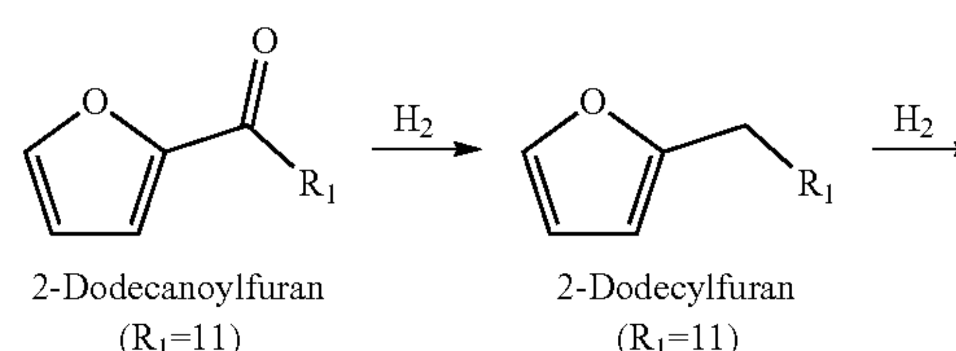
Scheme 10
