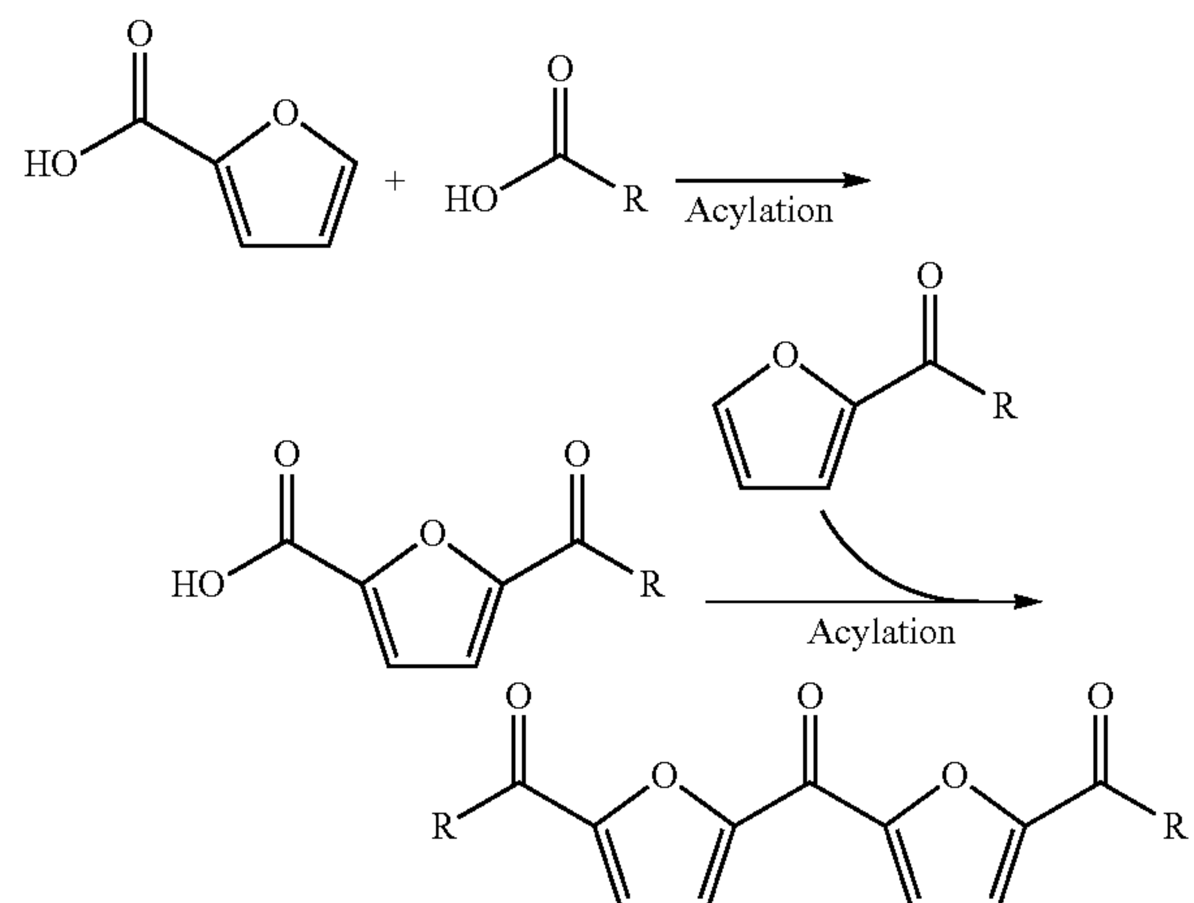
Scheme 2. Illustrative example of a synthesis of a Gemini surfactant to form a nonionic structure.
