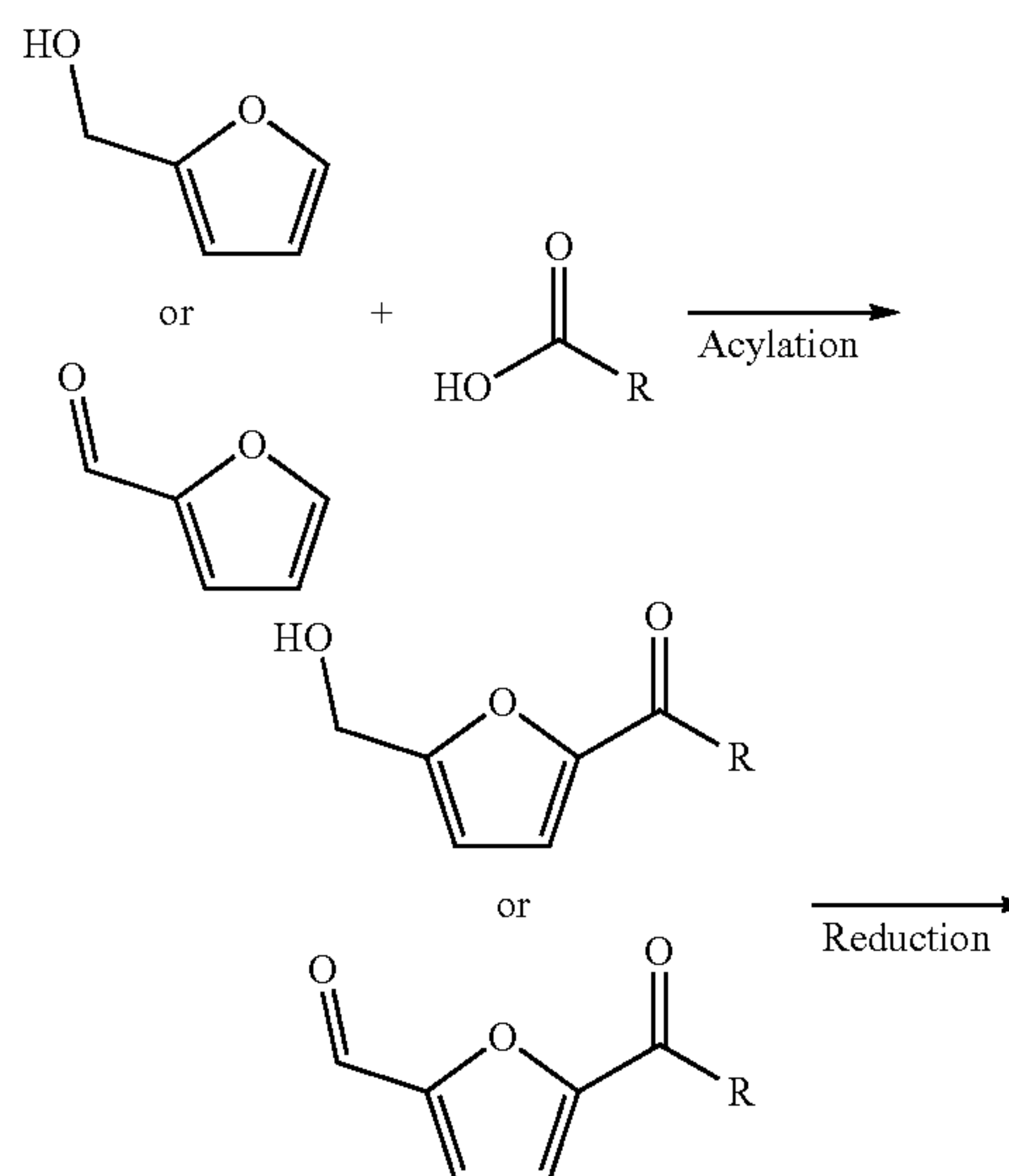
Scheme 3. Acylation of a furan-containing moiety with a hydrophobic group and subsequent reduction of all oxygen groups to hydroxyl groups, which can be further functionalized.
