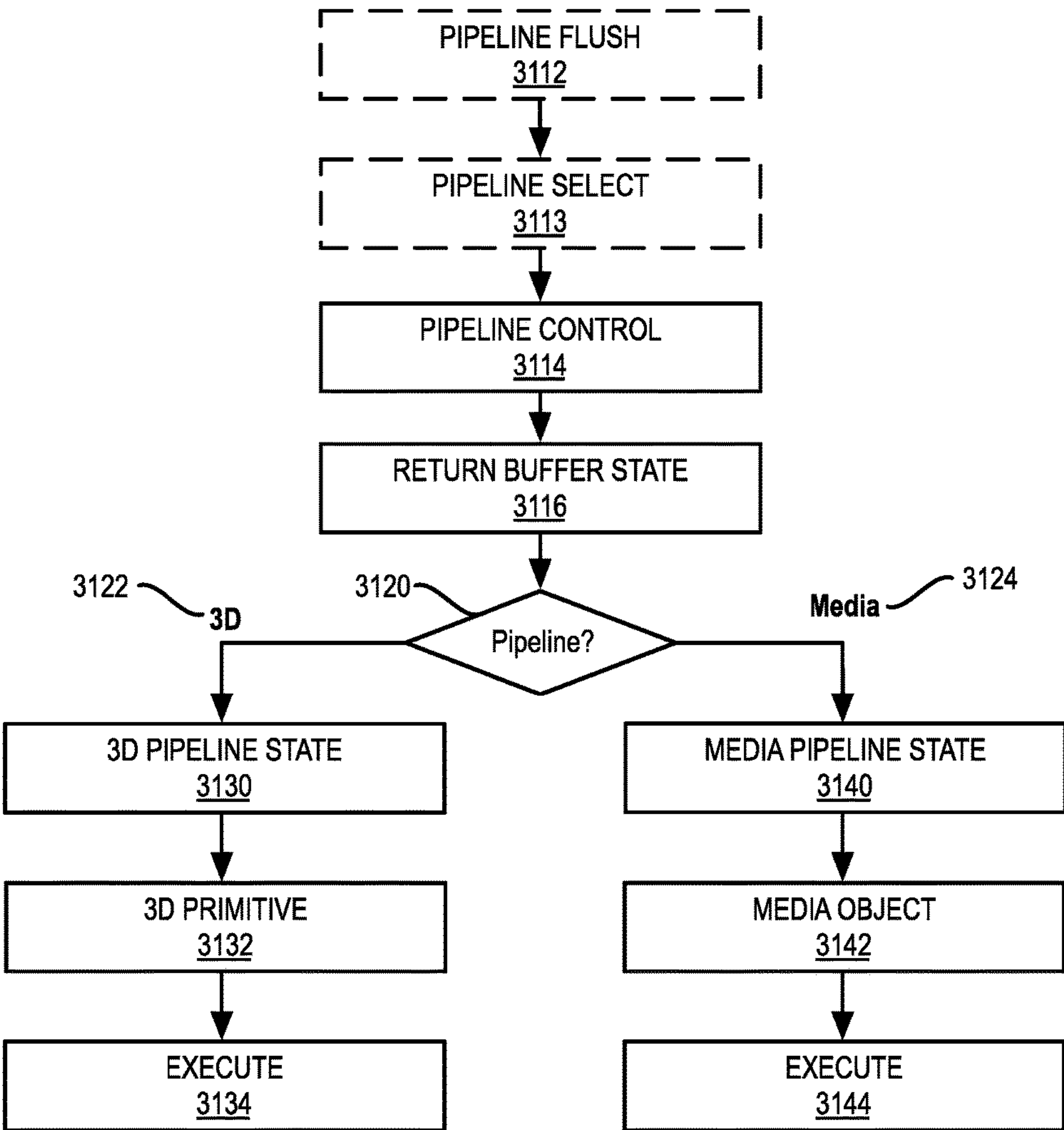
FIG. 31B GRAPHICS PROCESSOR COMMAND SEQUENCE 3110
