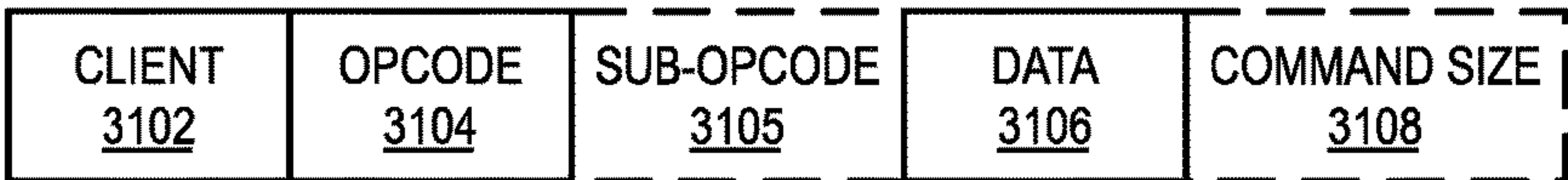
FIG. 31A GRAPHICS PROCESSOR COMMAND FORMAT 3100
