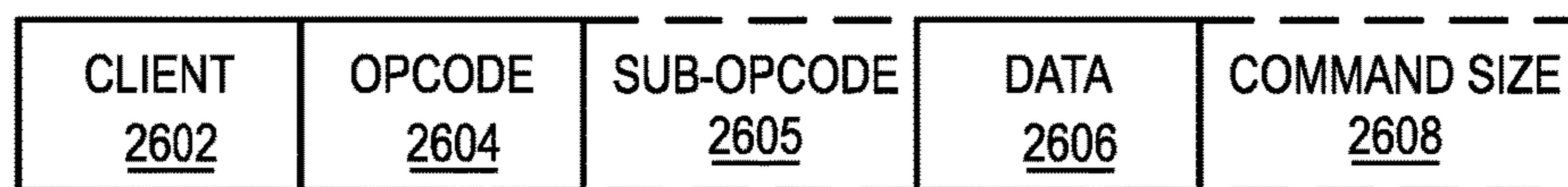
FIG. 26A GRAPHICS PROCESSOR COMMAND FORMAT 2600
