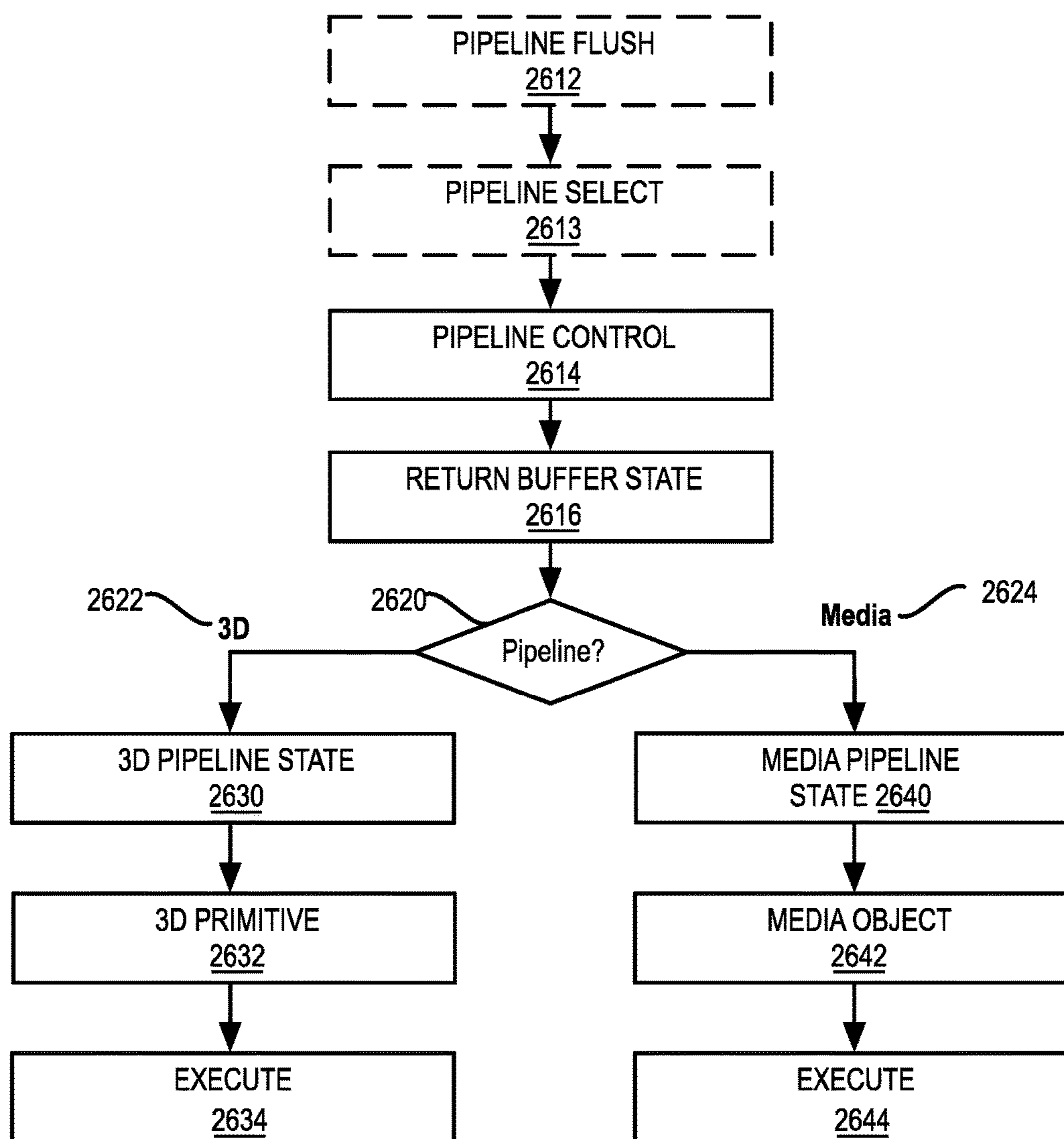
FIG. 26B GRAPHICS PROCESSOR COMMAND SEQUENCE 2610
