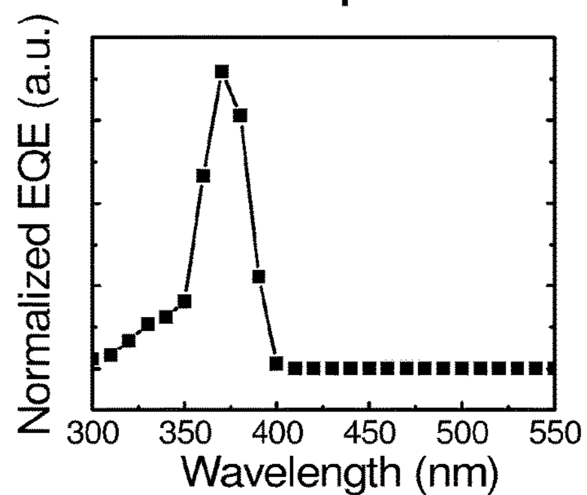
Detector spectrum
