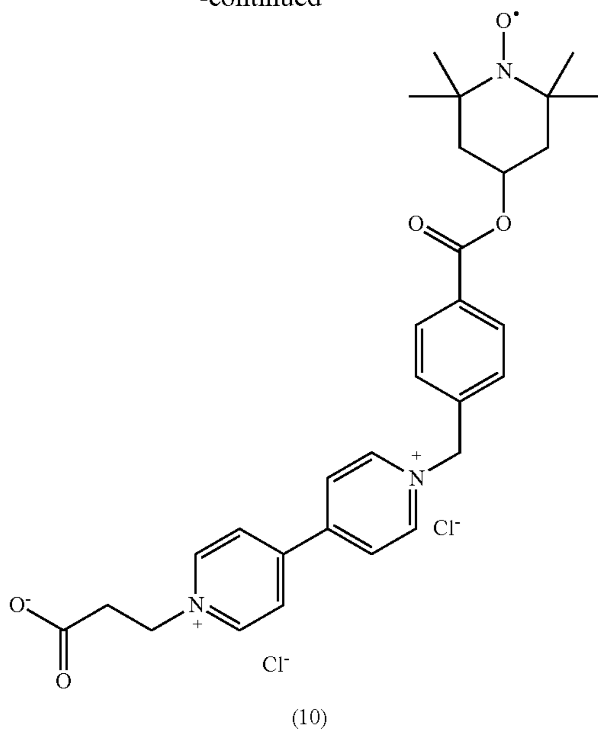
3-(1'-(4-(((1-Oxyl-2,2,6,6-tetramethylpiperidine-4-yl)oxy)carbonyl)benzyl)-[4,4'-bipyridin]-1,1'-dium-1-yl)propanoate-chloride (10, Short: Propanoate Viologen-TEMPO)
