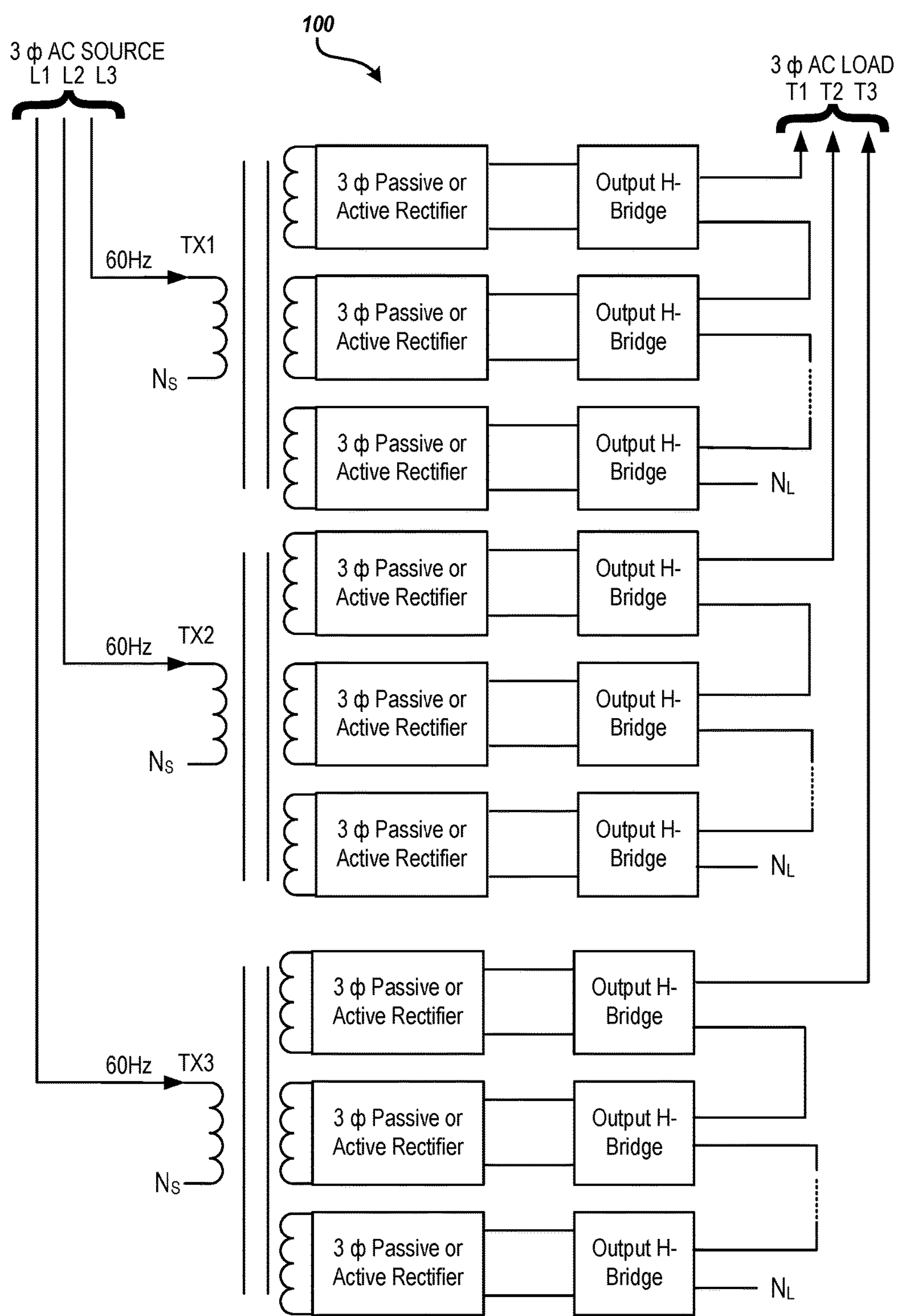
FIG. 1 (PRIOR ART)
