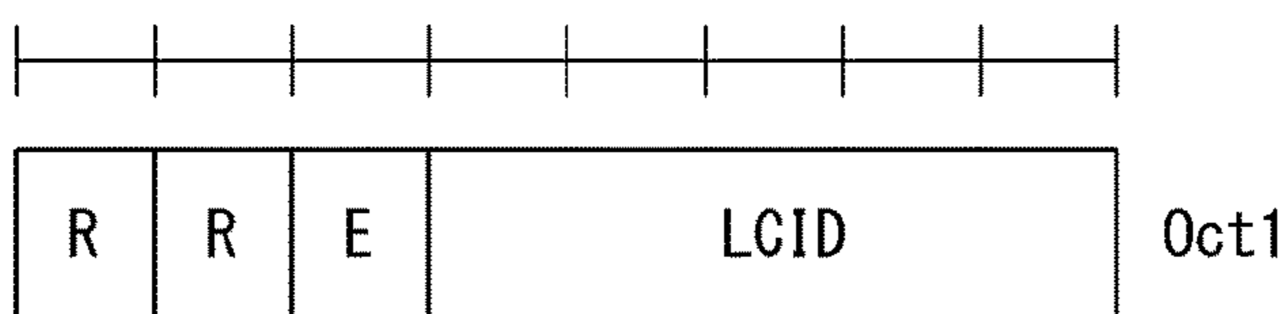
R/R/E/LCID sub-header
