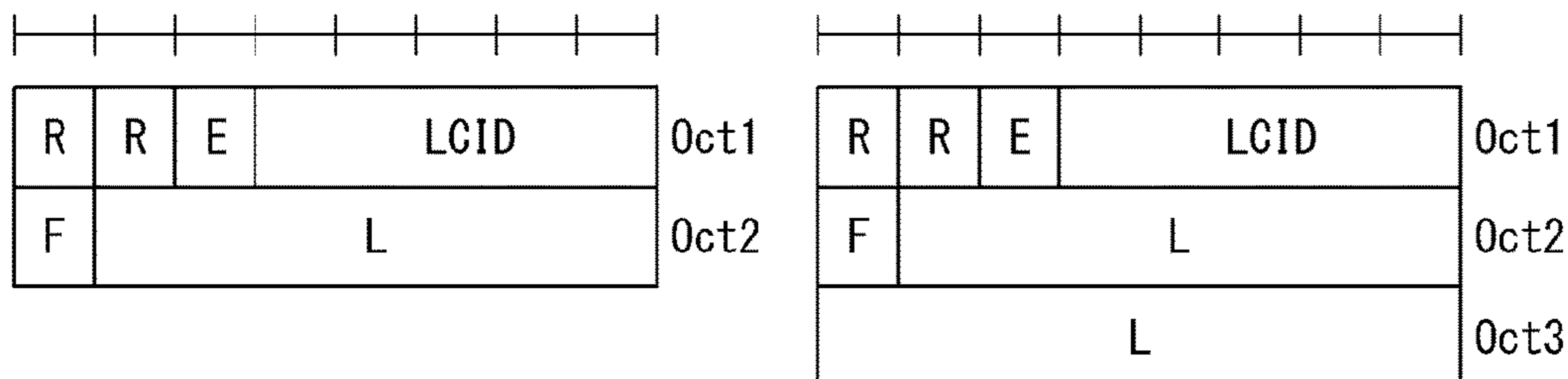
(a) R/R/E/LCID/F/L sub-header with 7-bit Lfield (b) R/R/E/LCID/F/L sub-header with 15-bit Lfield
