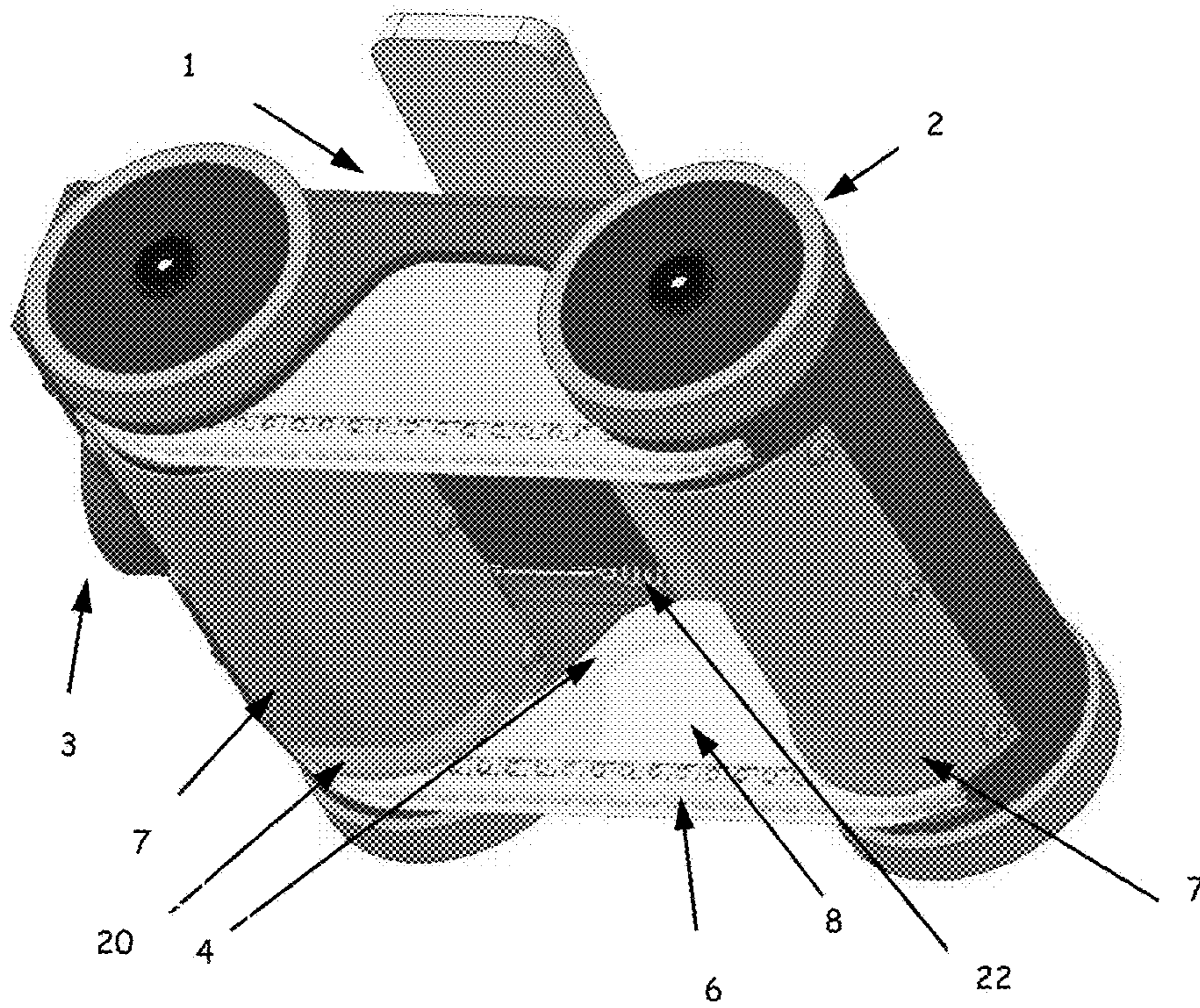
Fig. 7: View of alternate form of invention in which adaptive sealing mechanism is a combination of rigid and flexible components
