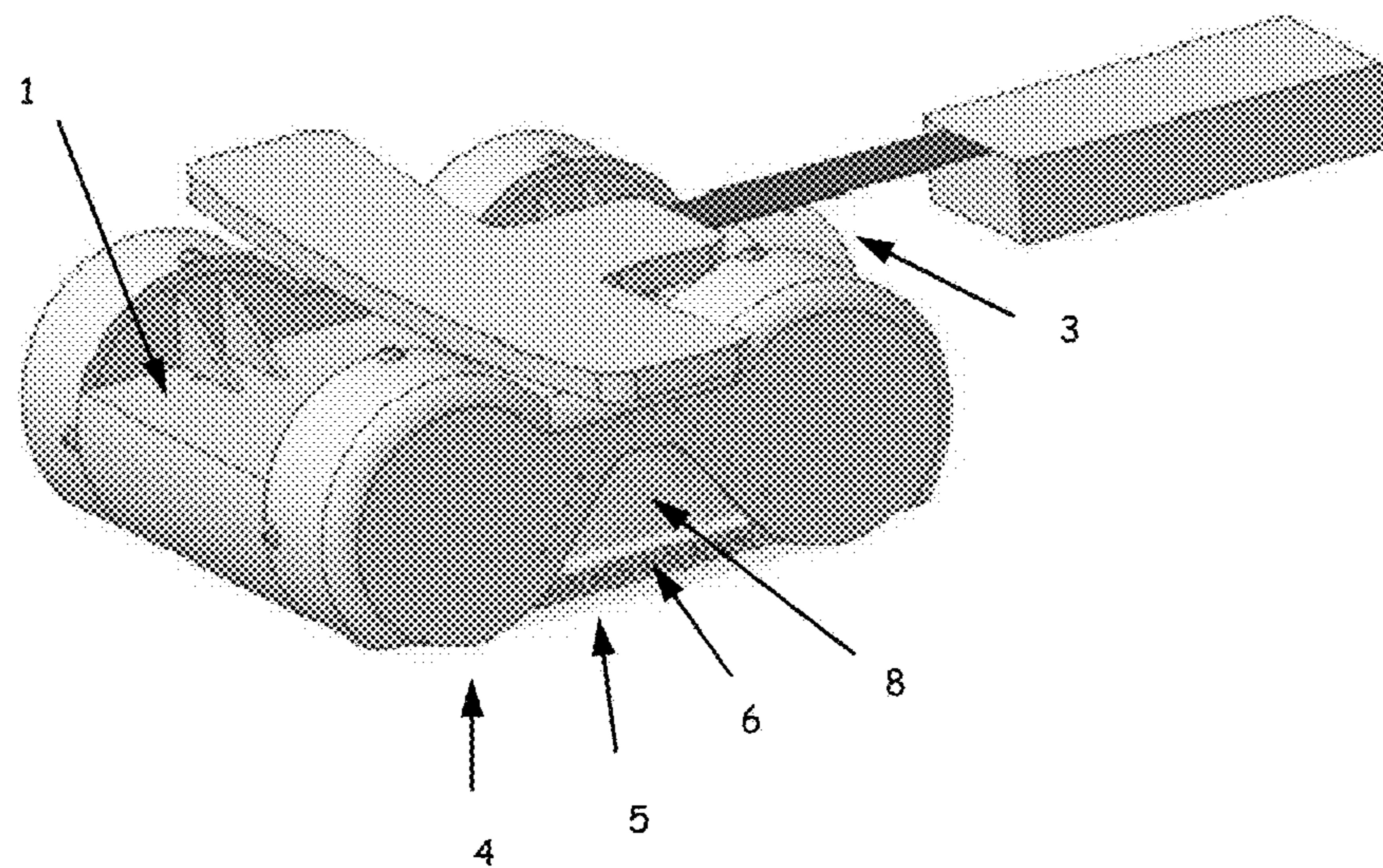
Fig. 6: Isometric view of alternate form of invention in which adaptive sealing mechanism is a combination of rigid and flexible components
