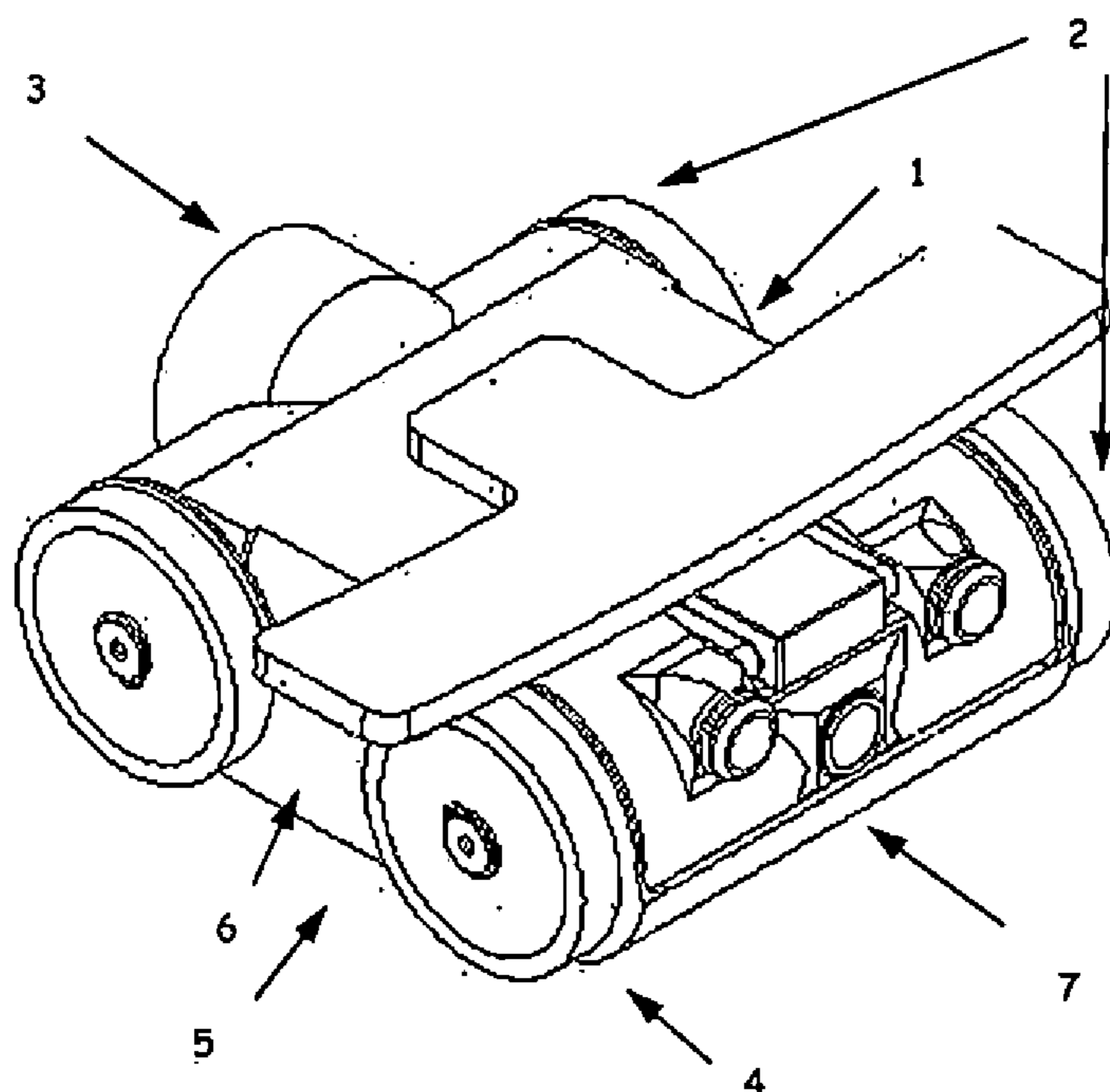
Fig. 1: Isometric view of the basic form of the invention
