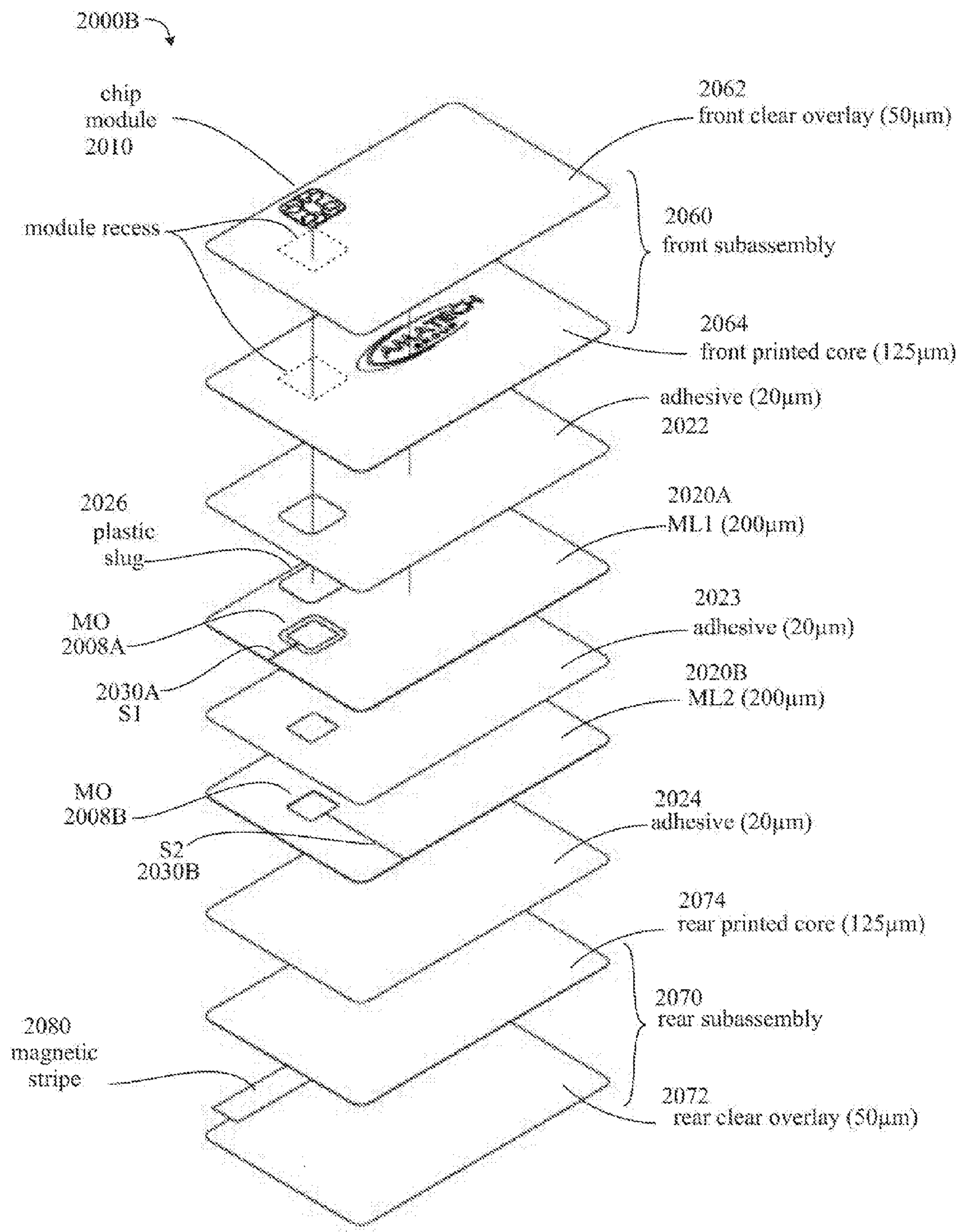
FIG. 20B two metal layers
