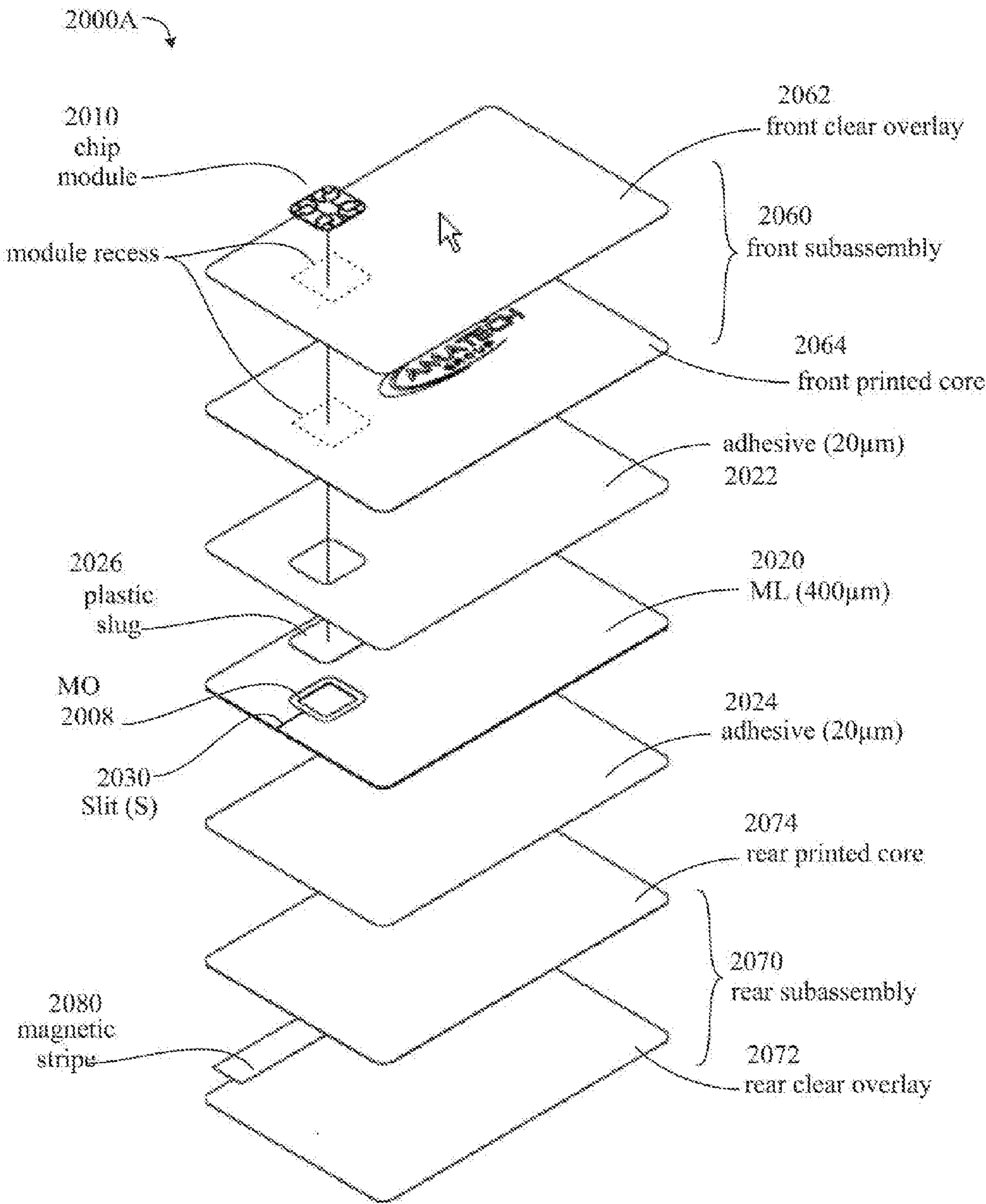
FIG. 20A “Plastic-Metal-Plastic” Hybrid Cards
