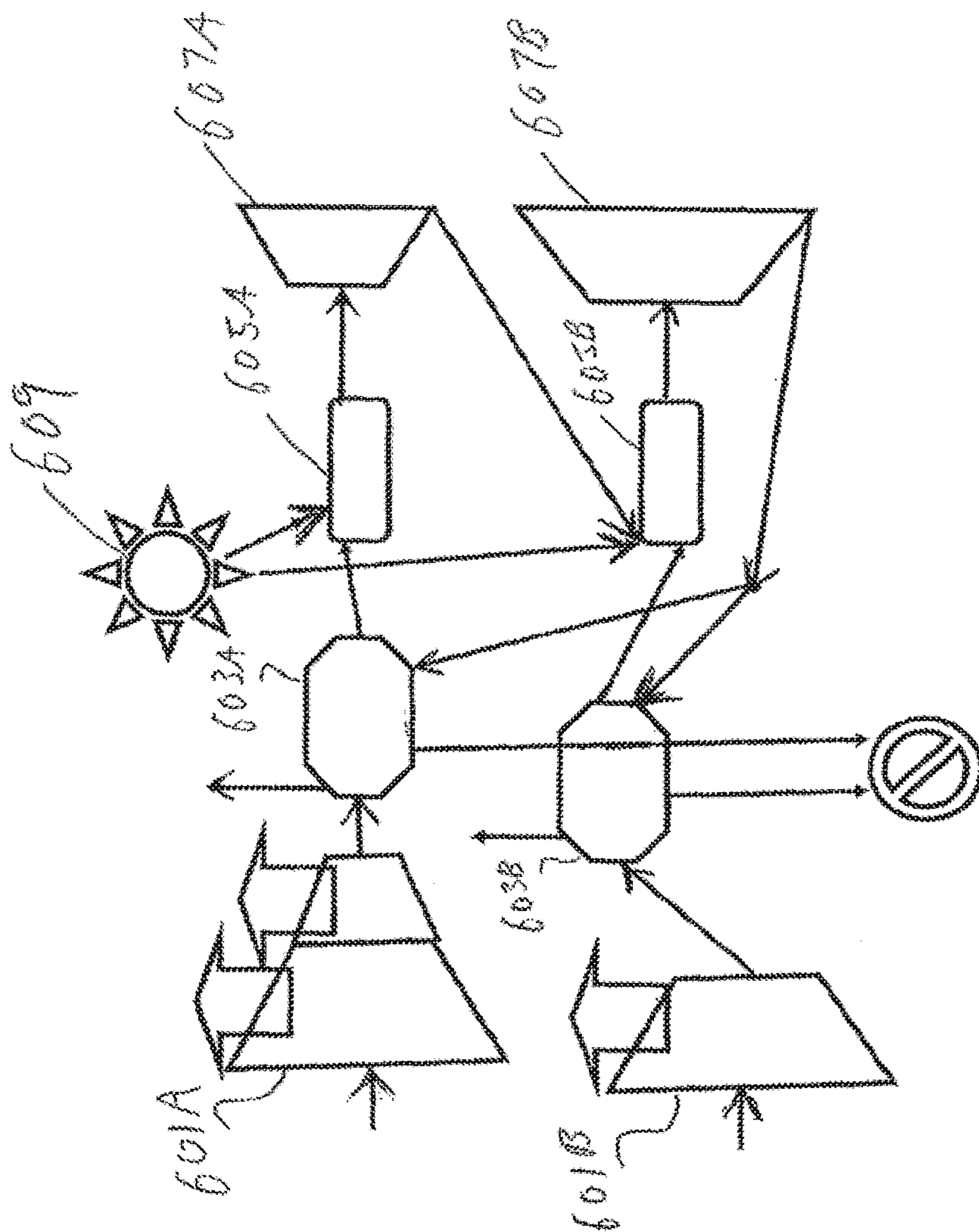
Fig. 6 Two Stage Novel Open Cycle n = 2
