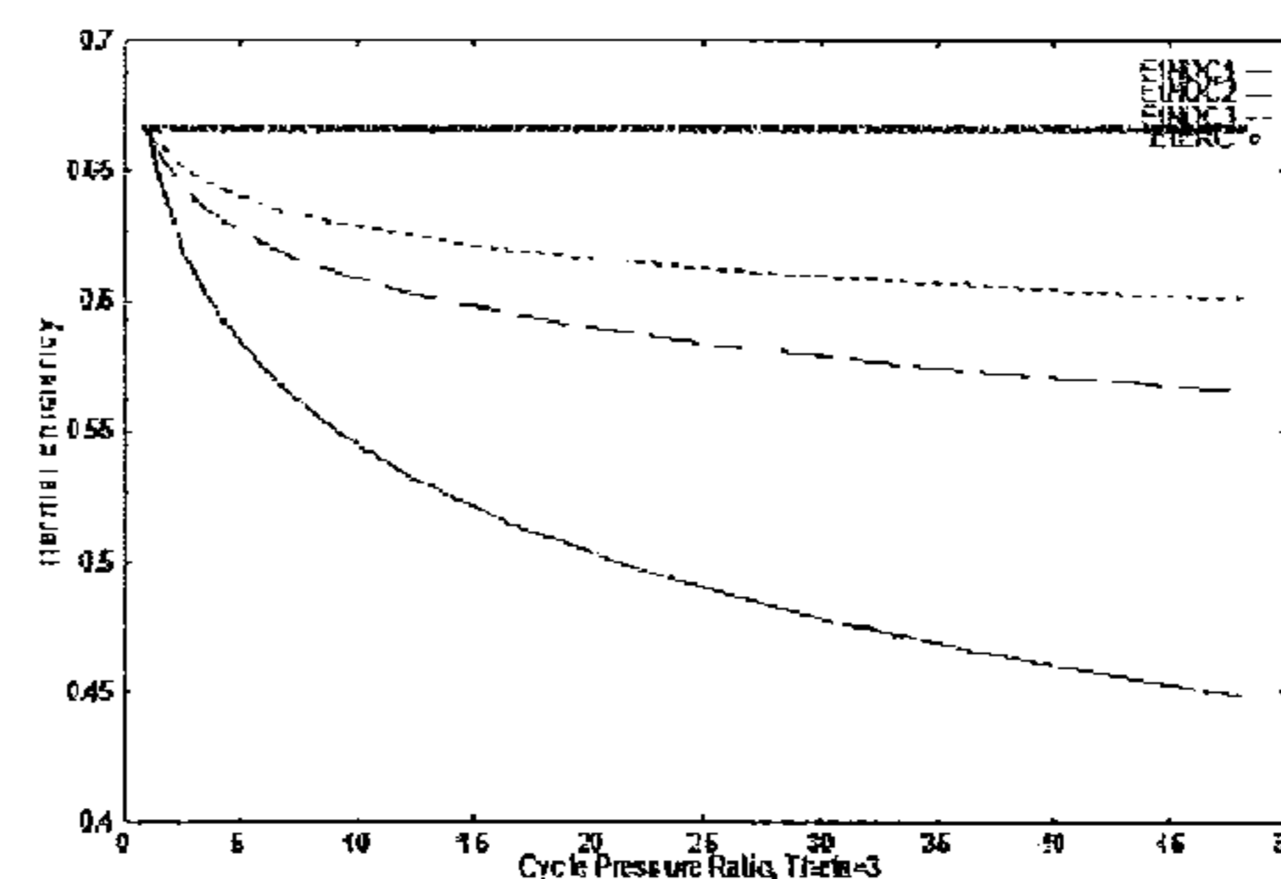
Fig. C-2(b) Variation of Thermal Efficiency for \theta = 3
