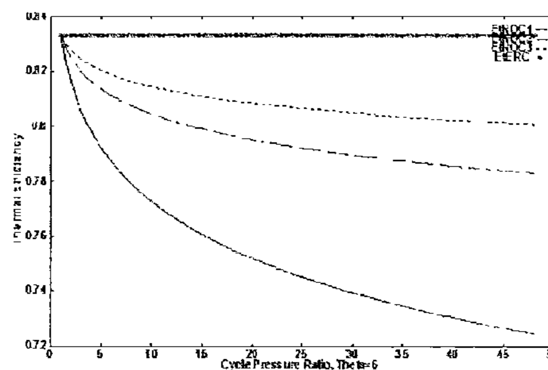
Fig. C-2(a) Variation of Thermal Efficiency for \theta = 6
