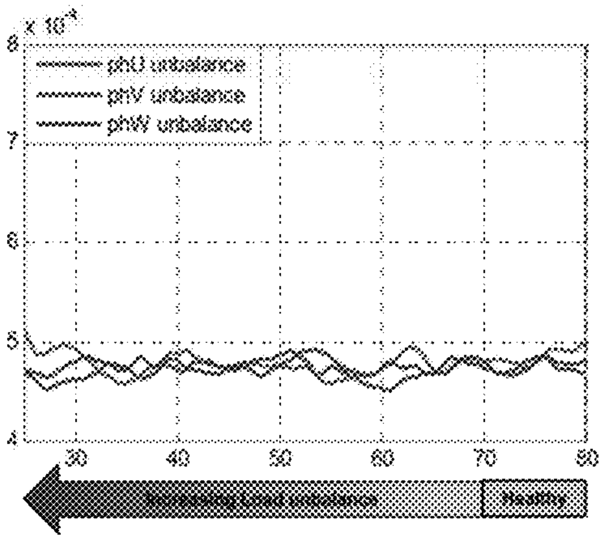
Fig 15: Magnitude of 5 th harmonic positive sequence flux under healthy and various degrees of load unbalance in three phase
