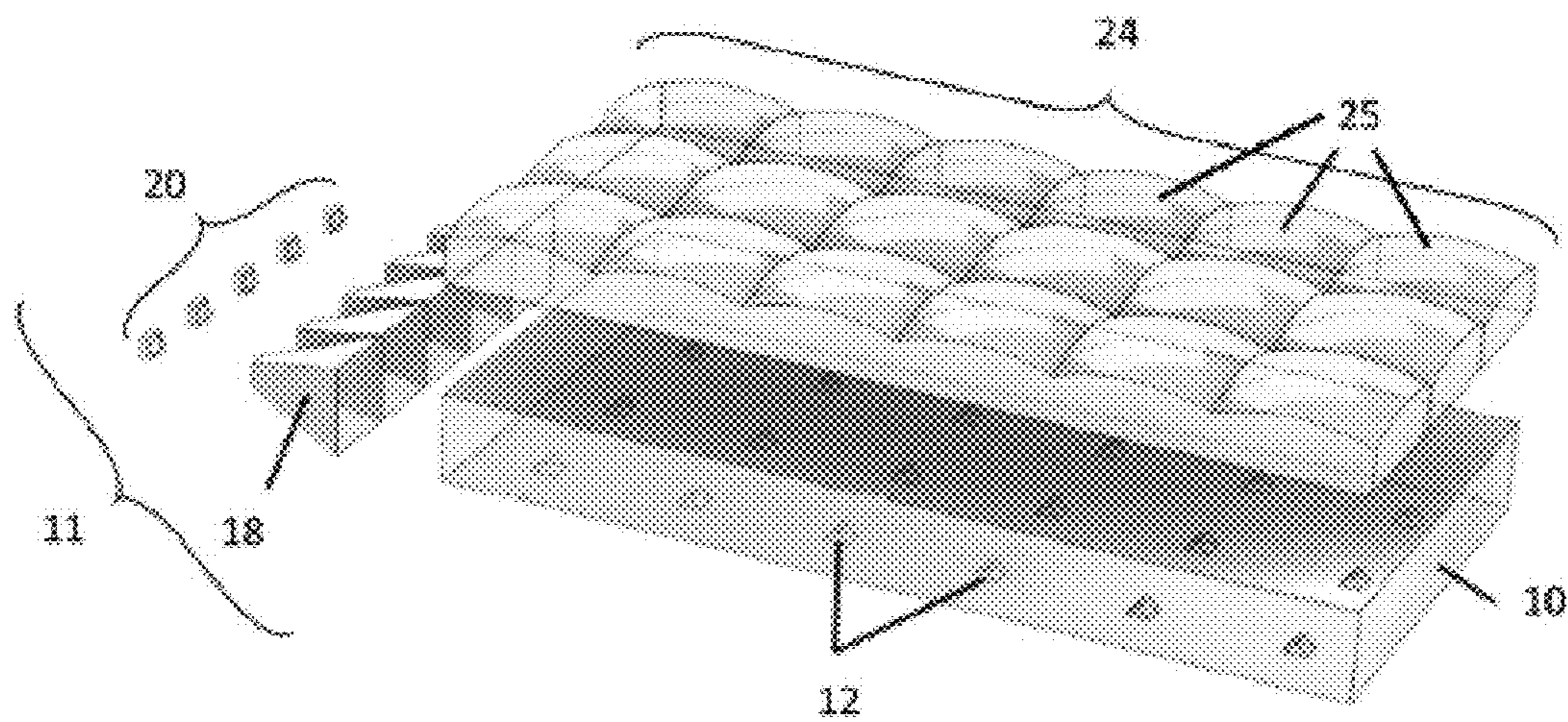
FIG. 1 (PRIOR ART)
