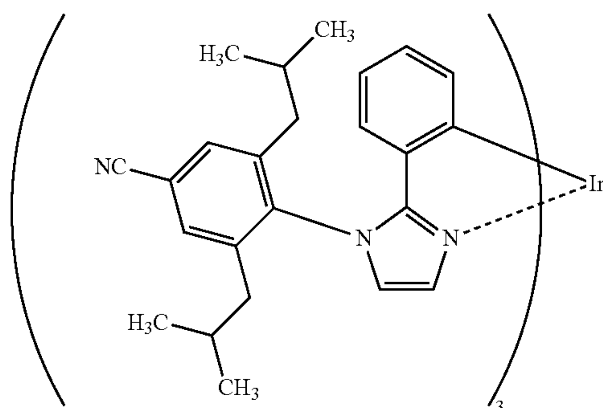
(102) \text{Ir}(\text{pim-diBuCNp})_3
