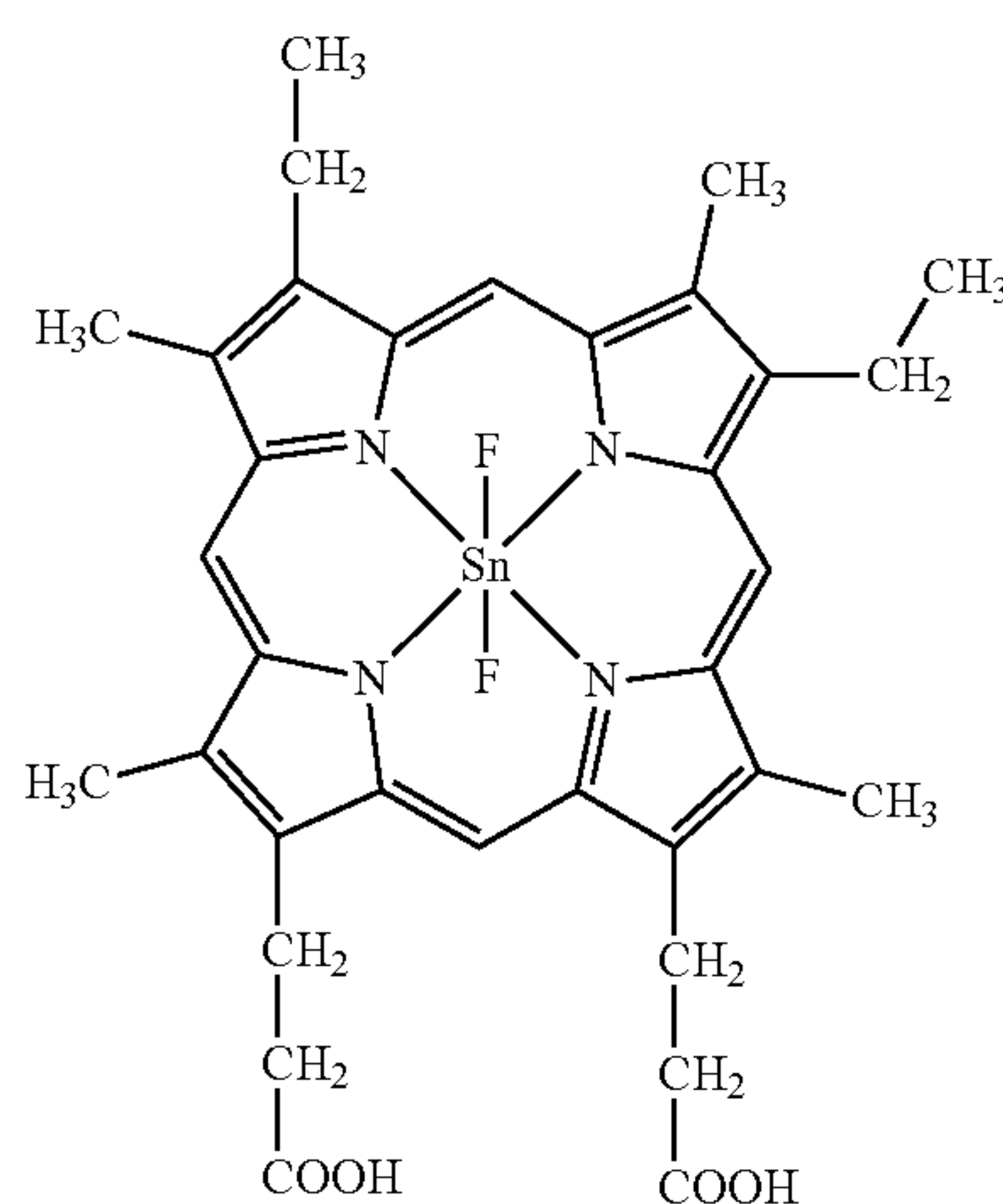
\text{SnF}_2(\text{Meso IX})
