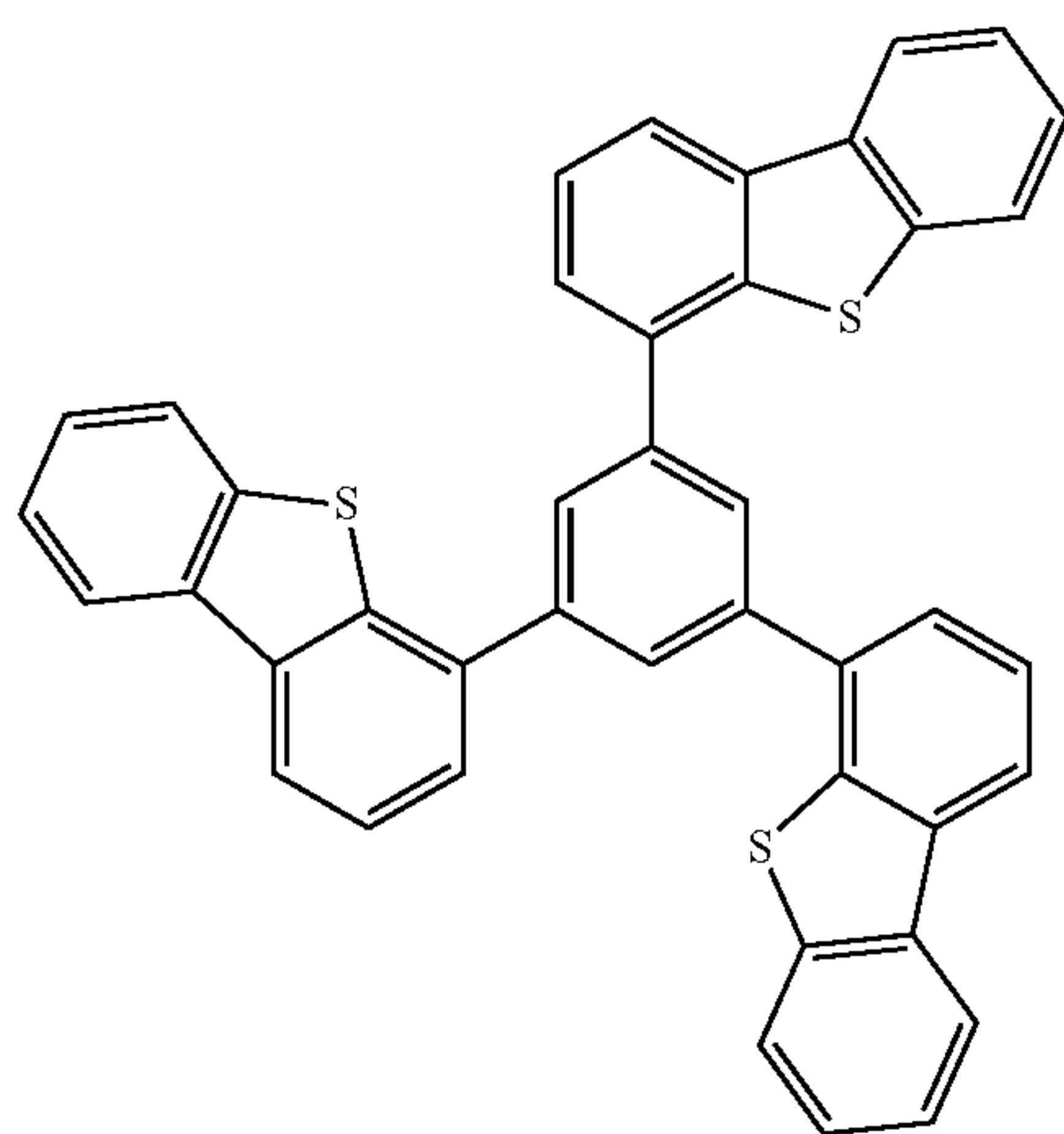
(i) DBT3P-II
