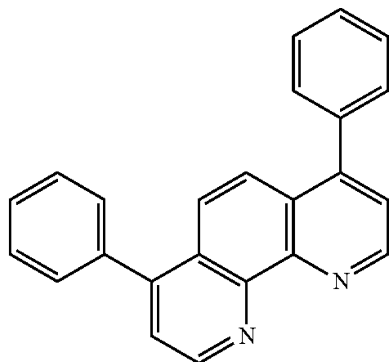
(vi) BPhen
