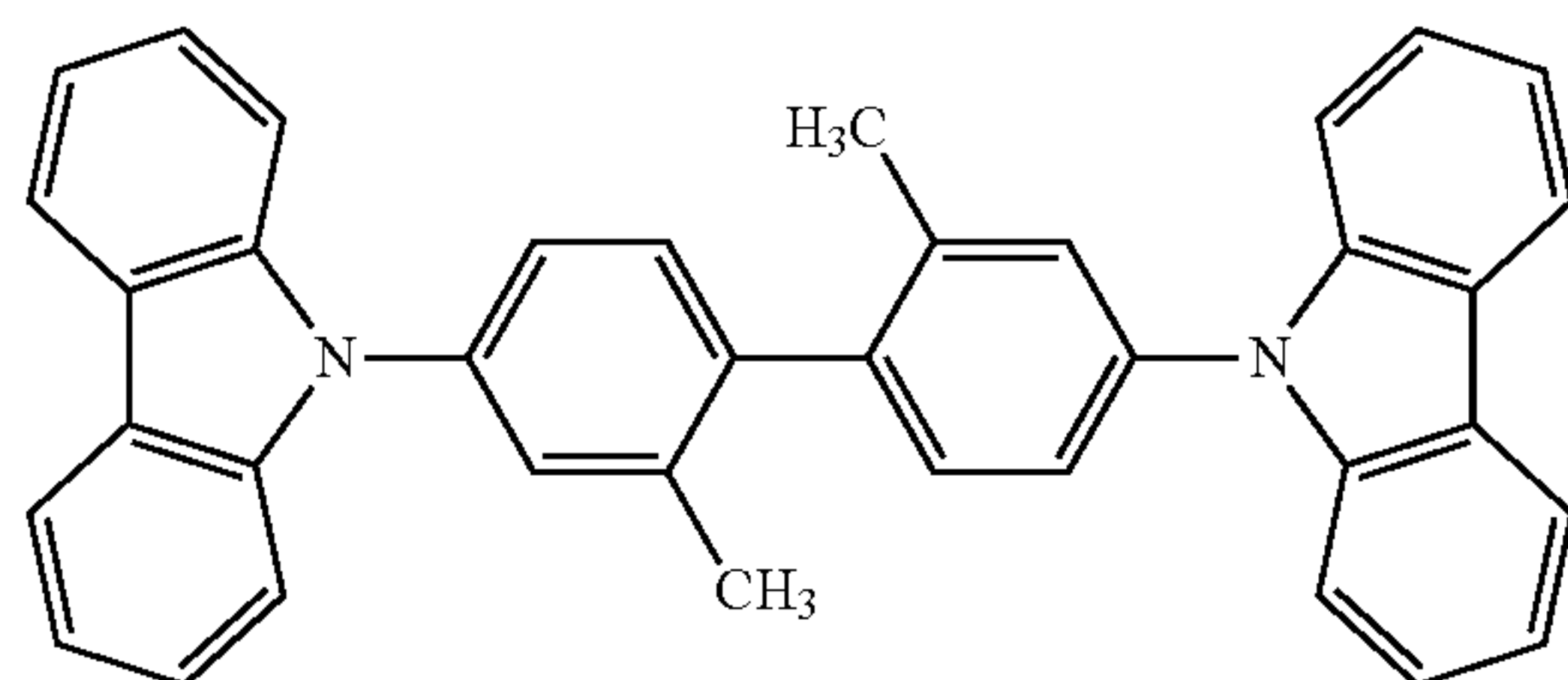
(ii) dmCBP
