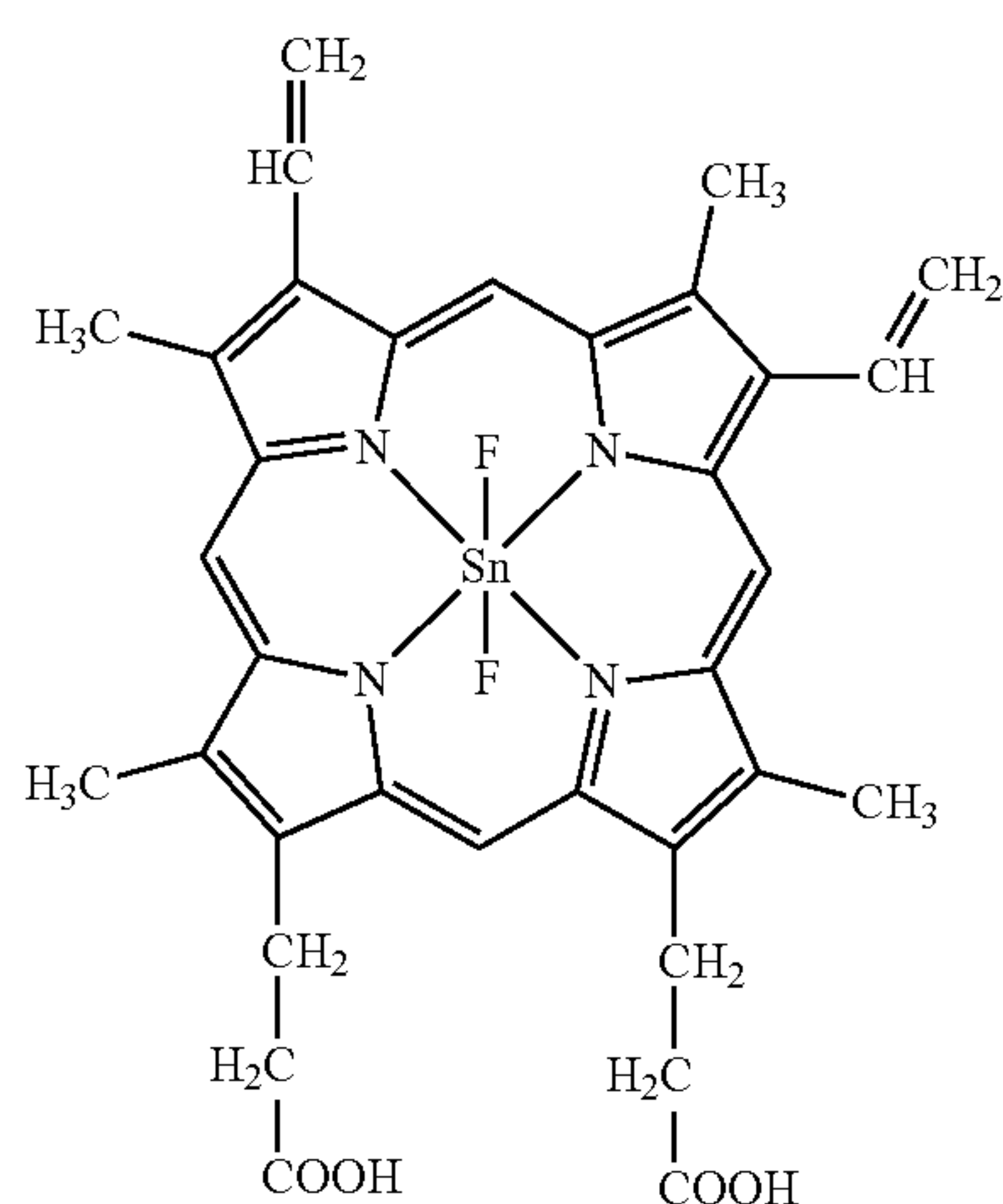
\text{SnF}_2(\text{Proto IX})
