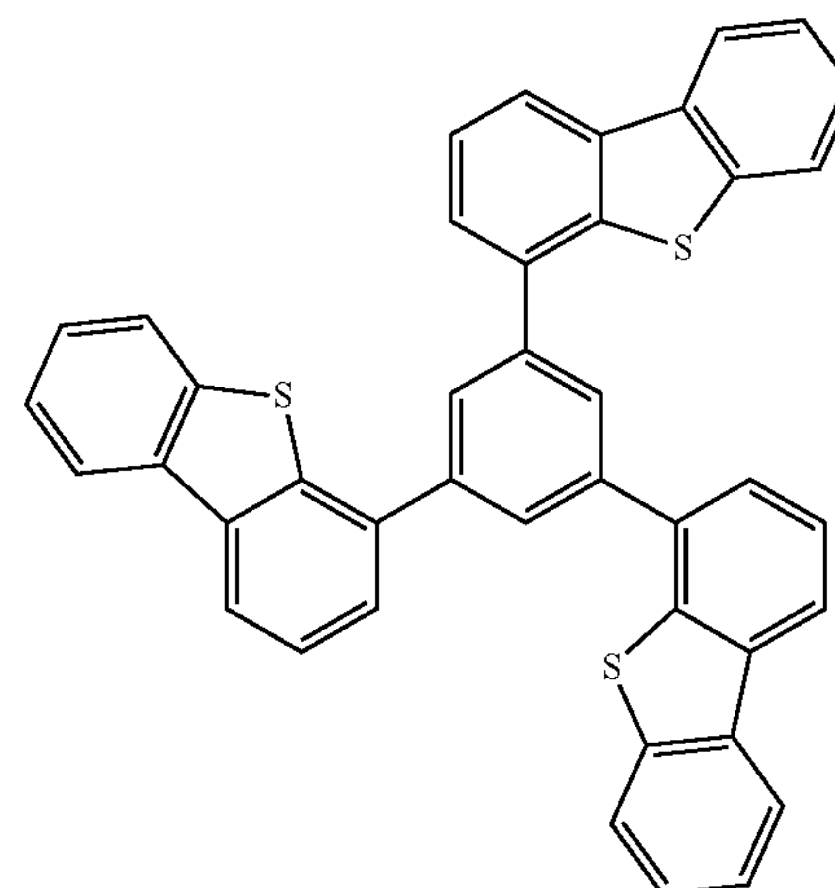
(i) DBT3P-II
