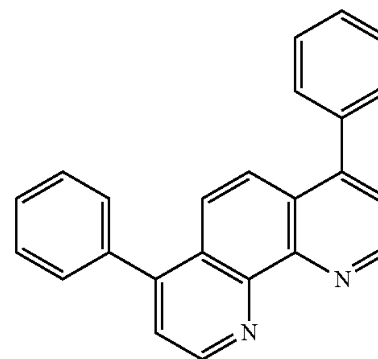
(vi) BPhen
