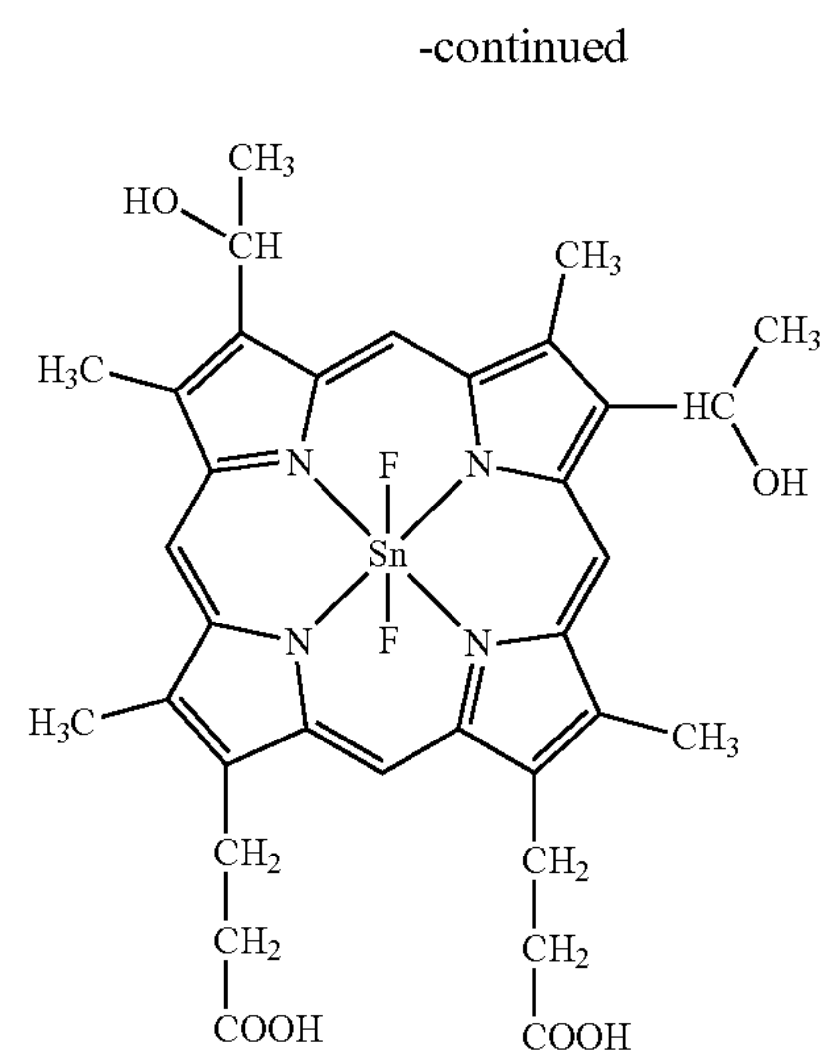
\text{SnF}_2(\text{Hemato IX})
