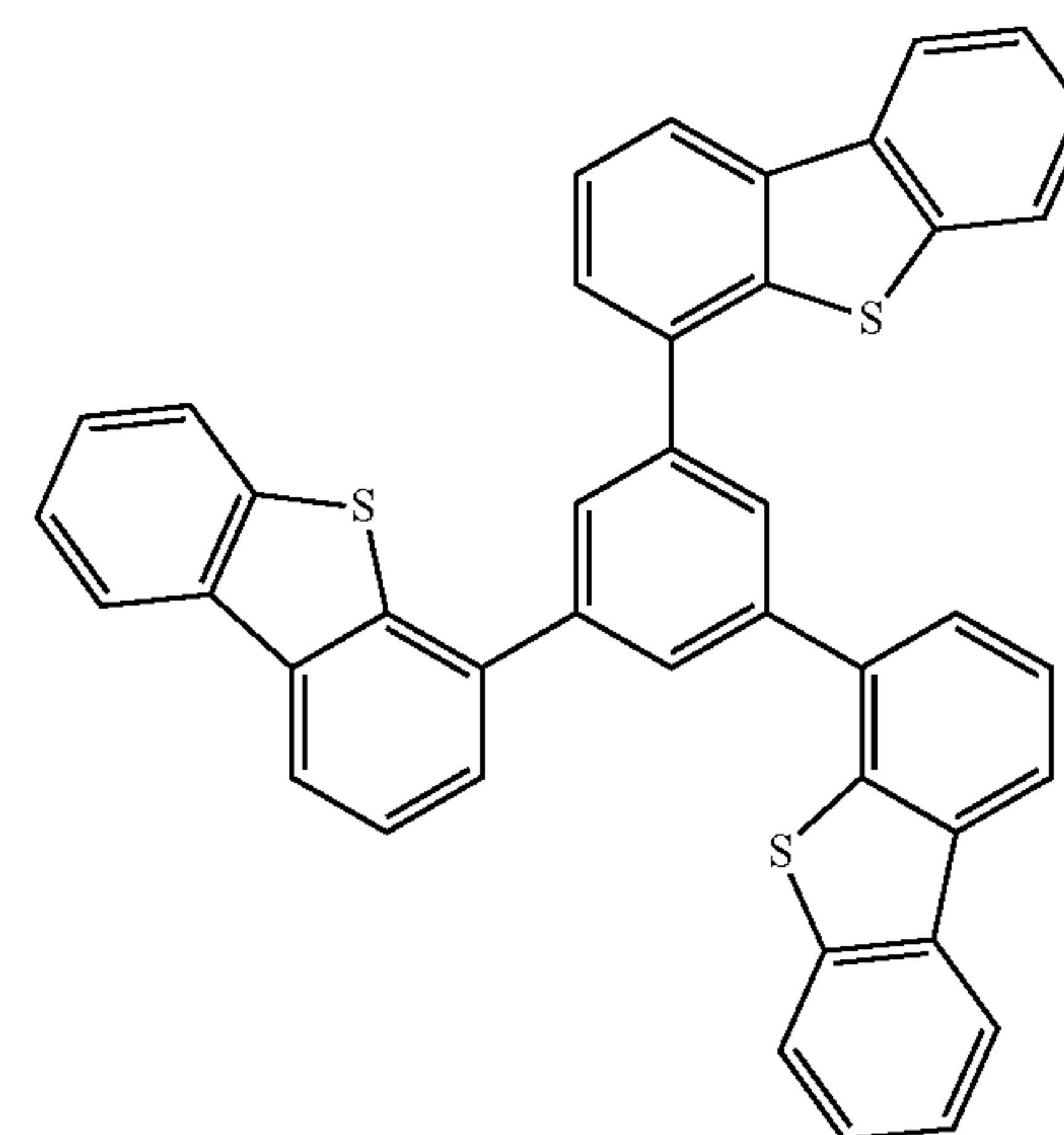
(i) DBT3P-II
