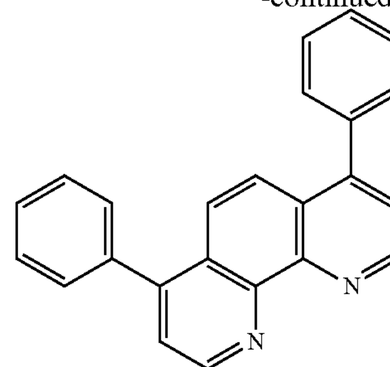
(vi) BPhen
