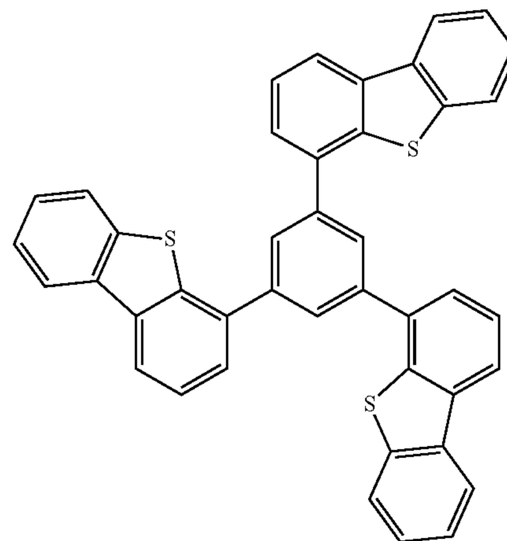
(i) DBT3P-II
