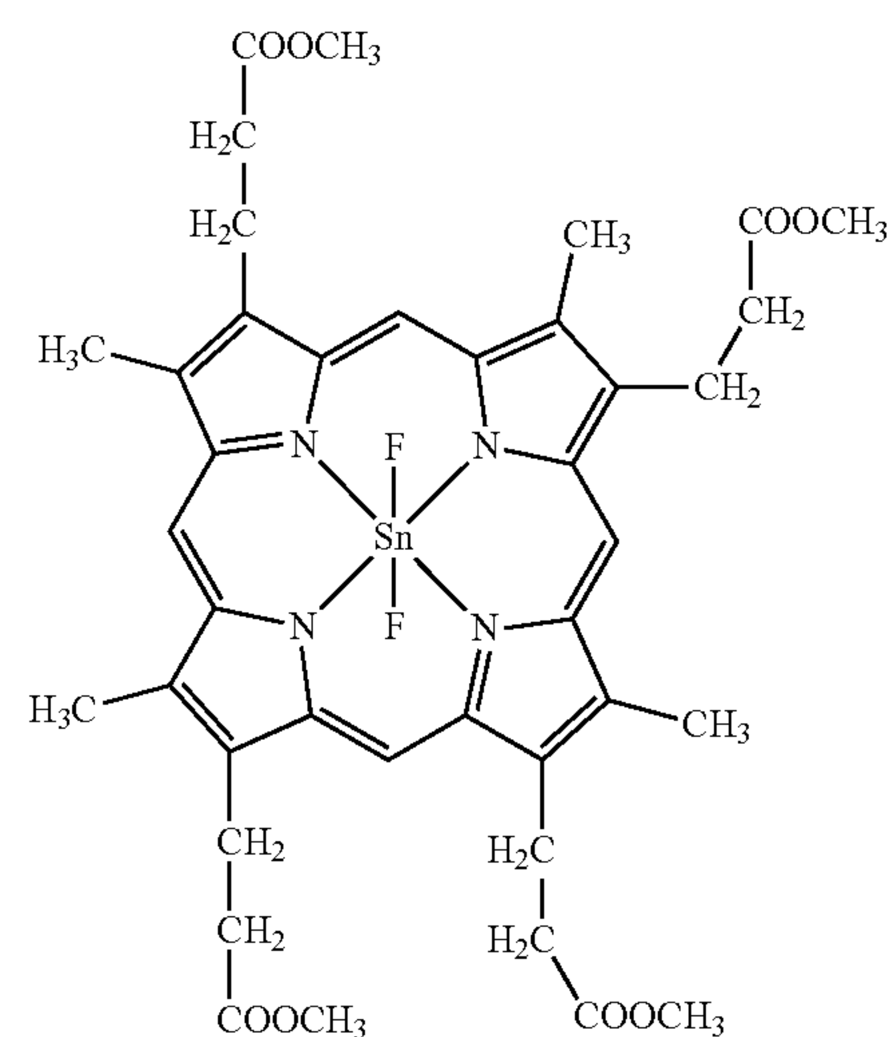
\text{SnF}_2(\text{Copro III-4Me})
