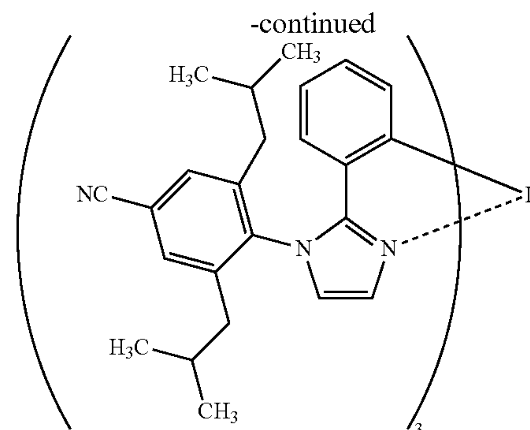
(x) \text{Ir}(\text{pim-diBuCNp})_3
