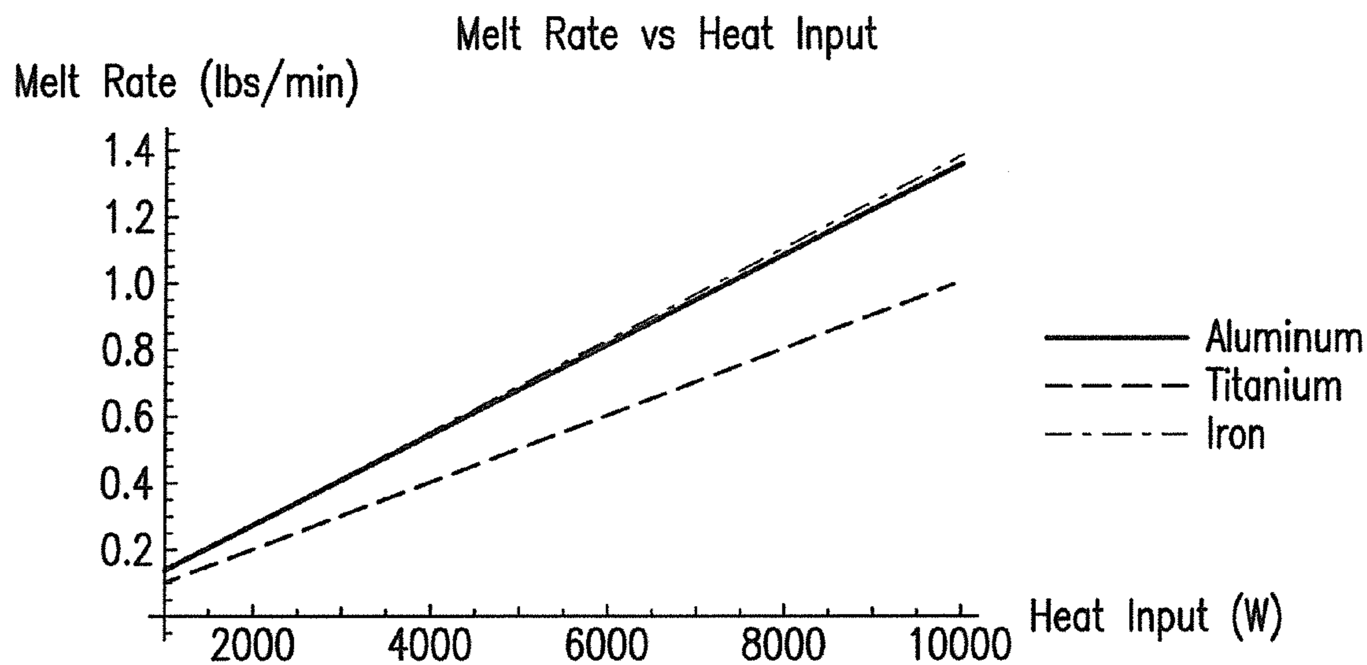
Melting rate of various materials vs the heat input to those materials
